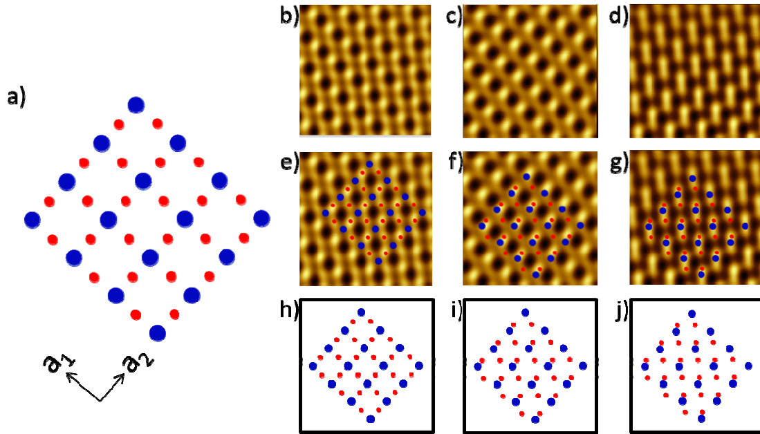
Figure 6: a) Relative bulk positions of Te ions (red) in the Te layer and nearest Tb ions (blue) from the rare-earth block layer directly below, projected onto the a - c . The axes are labeled as a_1 and a_2 since we are unable to distinguish the a - and c -axes in our measurements. b) c) and d): 25 Å square images cropped respectively from the bottom, middle, and top thirds of a Fourier-filtered 120 Å square image. The Fourier-filtered image only includes contributions from the Te and block-layer (Tb) structural signals. The block-layer signal was enhanced by a factor of 10 such that the Te and block layer signals are comparable. The differing images suggest differing relative locations for the Tb and Te ions in the three regions. e) f) and g): The specific lattice positions of the Te and Tb ions superimposed on the bottom, middle, and top images. For clarity, the Te and Tb ion positions for the bottom, middle, and top images are shown separately in h), i), and j) respectively. The shifts in the relative ion positions suggest a decoupling of the Te-layer from the rare-earth layer below.
