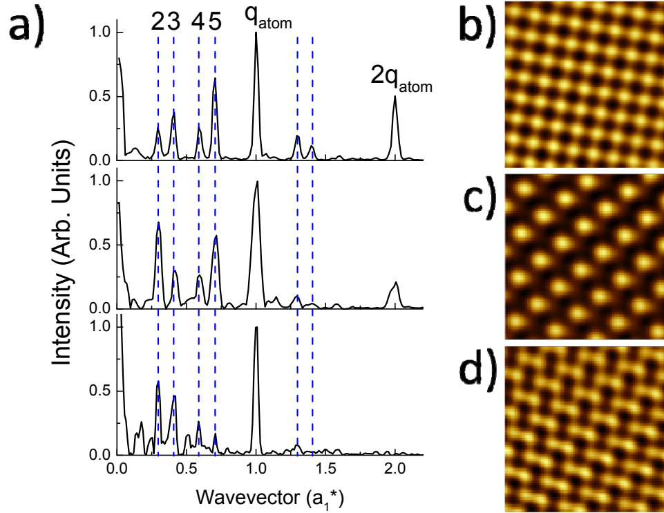
Figure 2: a) Linecuts through FFTs in the direction of the CDW (as in Figure 1d but now extending past 2q_{\text{atom}} ). The harmonic of the block signal, 2q_{\text{atom}} , is present in the top in middle plots but absent in the bottom plot. Peak 4 is present in all three cases indicating that peak is not the result of wavevector mixing involving the block harmonic, as the harmonic is absent in the bottom plot but peak 4 is still present. Slightly different tip conditions lead to variations in the relative intensities of the peaks in the FFT. Each of the FFTs, from which the linecuts are extracted, were taken on 400 Å square topographic images acquired with the same settings: I = 50 pA and V_{\text{sample}} = +150 mV with the same number of pixels and at temperatures at least 10 K below the bulk T_{\text{cdw}} . b),c),d) 25 Å square topographies which have been Fourier filtered to include only contributions from the Te net and rare-earth block signals. Small differences in tip conditions lead to a Te-dominated topography (b), a rare-earth block-dominated topography (c), and a topography which has the appearance of surface dimerization (d).
