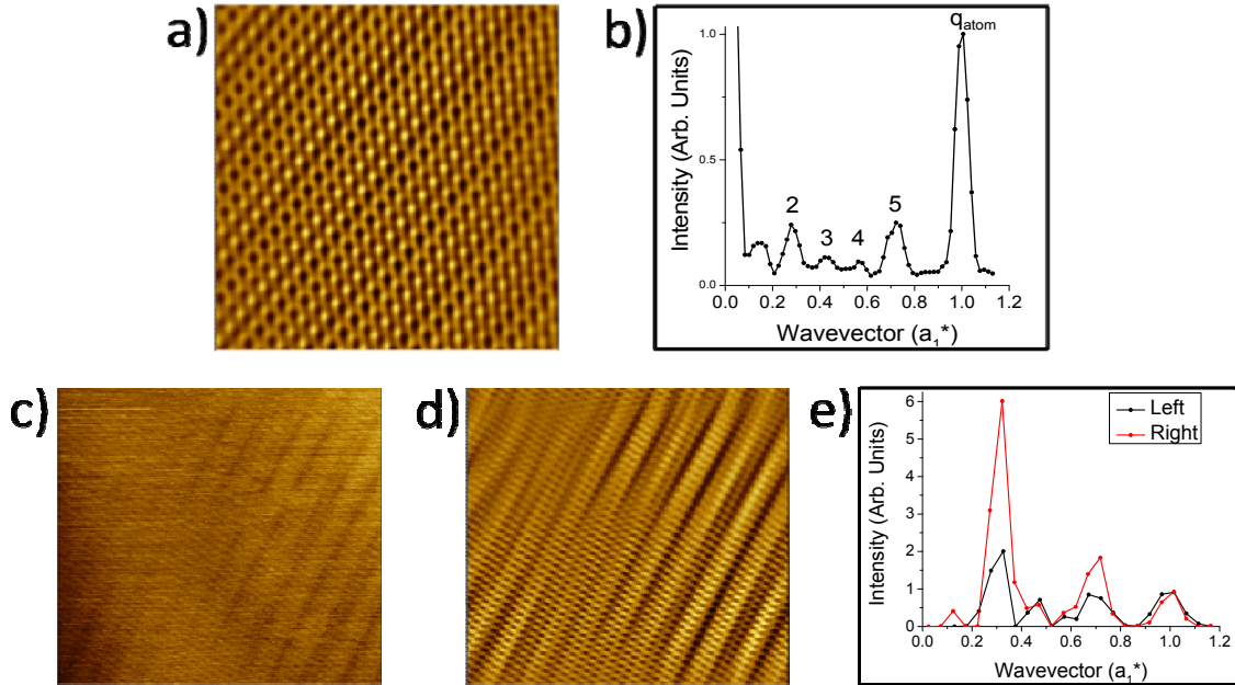
Figure 4: a) 90 Å square topography taken at 355 K with V_{sample} = +200 mV and I = 40 pA. The image was Fourier filtered to include the surface Te lattice, block layer, and CDW/wavevector mixing signals. b) Linecut through the FFT (of the raw topographic image for a) beginning at the origin, in the direction of the CDW, ending at the q_{atom} associated with the block layer. The standard 4 CDW/wavevector mixing peaks are observed. c) A 240 Å x 200 Å topography acquired at 339 K showing variations in the unidirectional CDW state across the region. V_{sample} = -200 mV and I = 70 pA d) The image in c) Fourier filtered to include Te net, block layer, and CDW/wavevector mixing signals to visibly emphasize local variations in the CDW state. e) A comparison of the linecuts through the FFTs separately for the left and right halves of image c). The \sim 2/7a_1^* CDW peak is \sim 3 larger in the right half as compared to that of the left illustrating strong variation in the a_1 -axis CDW in this region.
