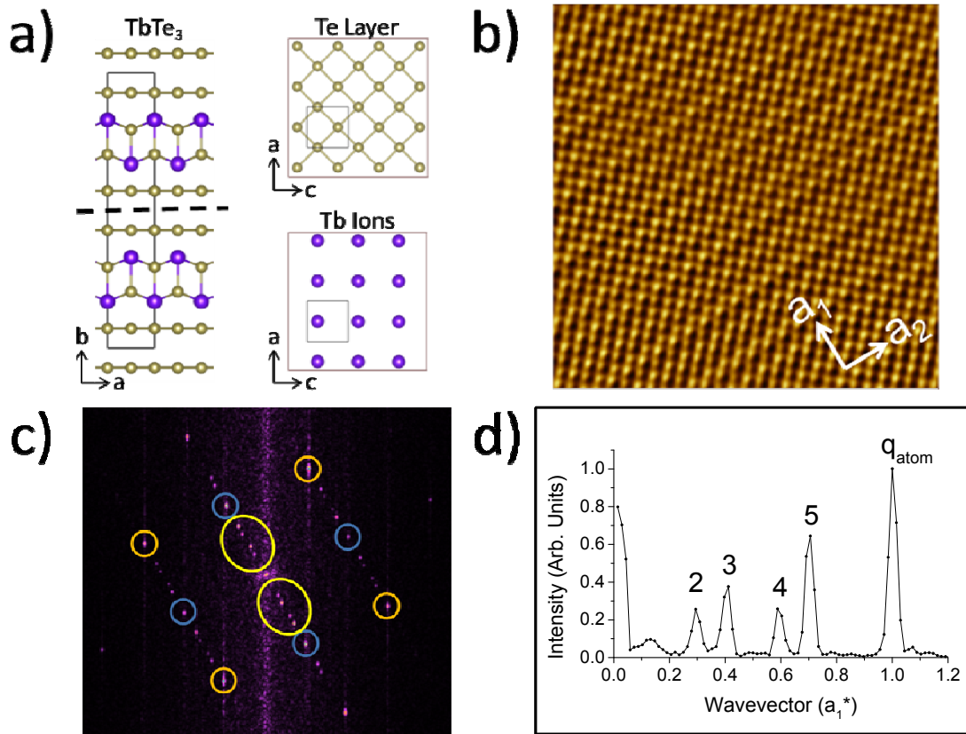
Figure 1: a) At left, the crystal structure for TbTe 3 with a black rectangle outlining the unit cell. The dotted line indicates the a - c cleave plane between the double Te layers. At right, the square lattice of the Te layer which is exposed by cleaving as well as the locations of the closest Tb ions in the rare-earth block layer directly below. The unit cell is again shown in the structures at right for reference. The crystal structures were constructed using Vesta software [51]. b) Topographic image taken over a 90 Å square region at I = 65 pA, V_{\text{Sample}} = -350 mV. The Te-square lattice of the exposed surface can be clearly seen as well as superimposed “stripes” associated with a unidirectional CDW state along the a_1 crystal axis. We use a_1 and a_2 to denote the in-plane crystal axes for our measurements since we observe unidirectional CDW order along both axes. This prevents us from unambiguously identifying the a - and c -crystal axes. c) FFT of a typical topographic image. Orange circles identify the wavevectors associated with Te-square lattice. Blue circles identify the wavevectors associated with the subsurface rare-earth block layer (Tb ions). The yellow ovals enclose peaks in the FFT which are associated with the unidirectional CDW as well as those arising from mixing between the CDW wavevector and block atomic wavevectors. d) Linecut through the FFT, beginning at the origin (center), in the direction of the CDW (through yellow oval), and ending just past q_{\text{atom}} (blue circle) associated with the block layer.
