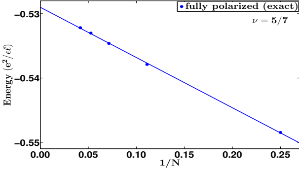
FIG. 6: Thermodynamic extrapolation of the lowest Landau level Coulomb ground state energy for the fully spin polarized state at \nu = 5/7 .
