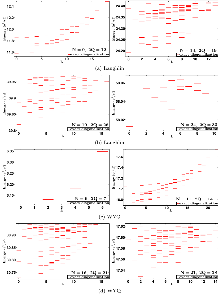
FIG. 5: Coulomb spectra obtained from exact diagonalization in the spherical geometry for N fully spin polarized electrons at \nu = 5/7 at the total flux 2Q(hc/e) corresponding to the Laughlin (top two panels (a) and (b)) and WYQ state (bottom two panels (c) and (d)).
