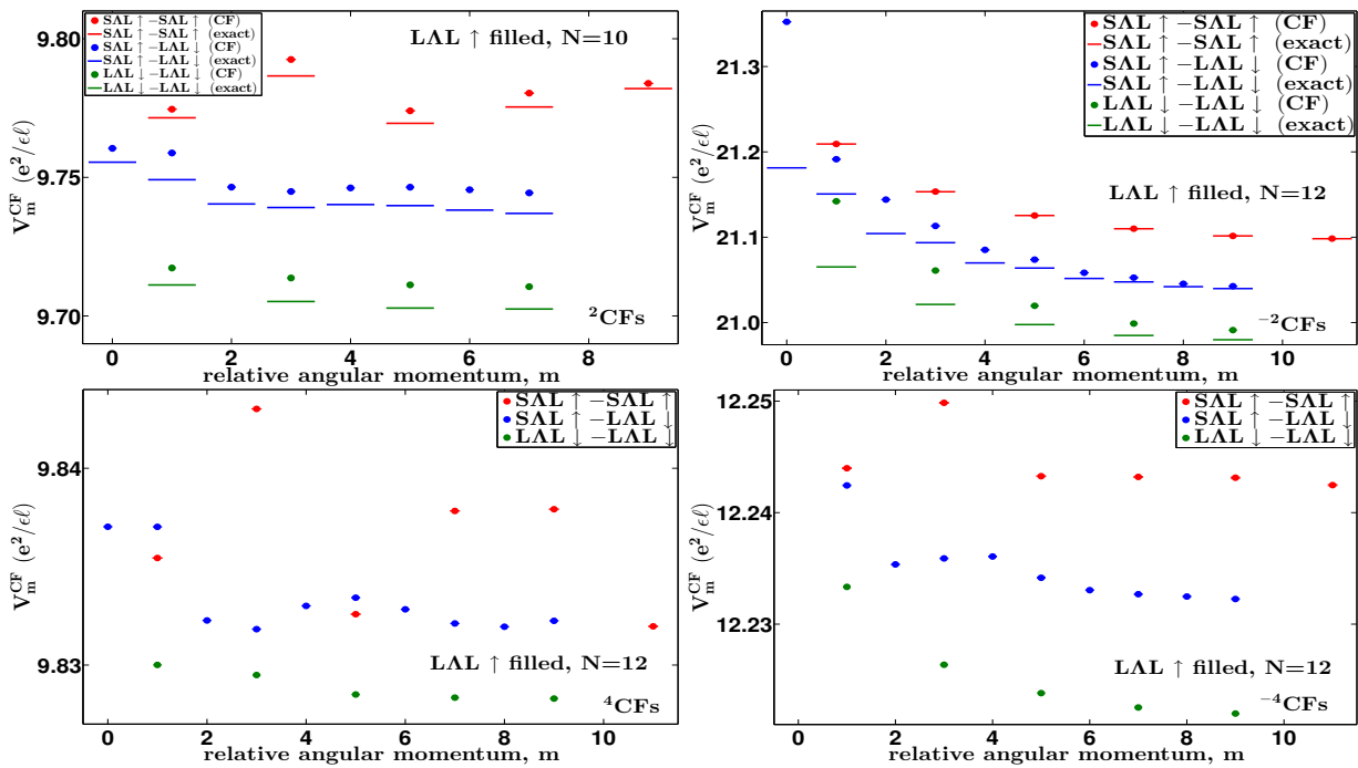
FIG. 2: Coulomb interaction energy of two composite fermions in the presence of a filled spin up lowest \Lambda level carrying two (top panels) or four (bottom panels) vortices and experiencing an effective magnetic field in the same (left panels) or opposite (right panels) direction as the external magnetic field calculated in the spherical geometry. The dashes (dots) show the energies obtained from exact (CF) diagonalization.
