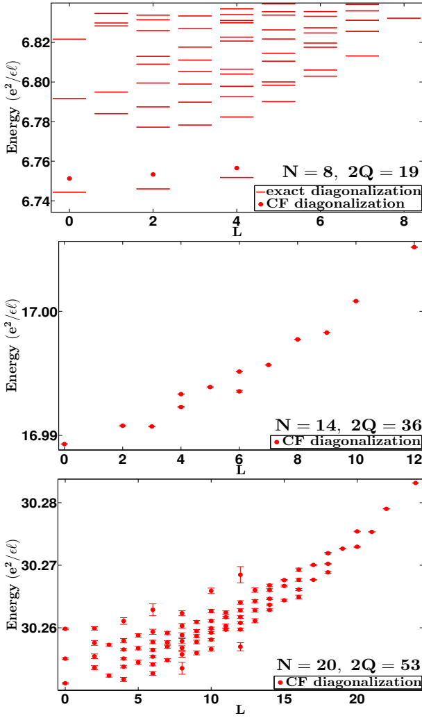
FIG. 8: Coulomb spectra in the spherical geometry for N electrons at flux 2Q(hc/e) with total spin S corresponding to the partially spin polarized state at \nu = 6/17 . The red dashes (dots) show the energies obtained from exact (CF) diagonalization.
