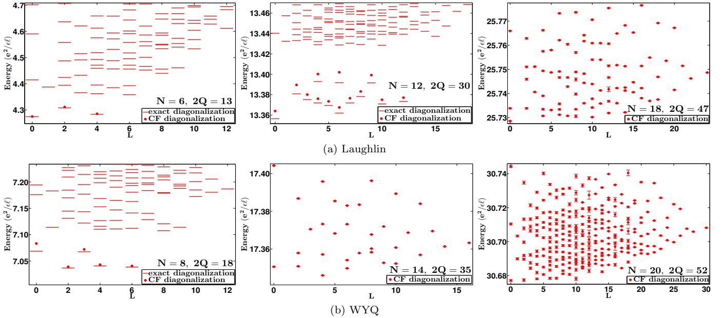
FIG. 7: Coulomb spectra in the spherical geometry for N fully spin polarized electrons at total flux 2Q(hc/e) at \nu = 6/17 . The red dashes (dots) show the energies obtained from exact (CF) diagonalization at the flux corresponding to the Laughlin (top panel (a)) and WYQ state (bottom panel (b)).
