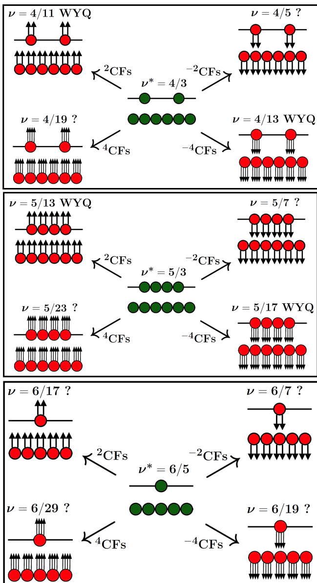
FIG. 1: (color online) Schematic of the various fractional quantum Hall states obtained from a filling \nu^* = 4/3 (top panel), \nu^* = 5/3 (middle panel) and \nu^* = 6/5 (bottom panel) of composite fermions. The green solid dots represent electrons while the red solid dots with 2p arrows are composite fermions carrying 2p vortices in the same (arrows pointing up) or opposite (arrows pointing down) direction to the external magnetic field.
