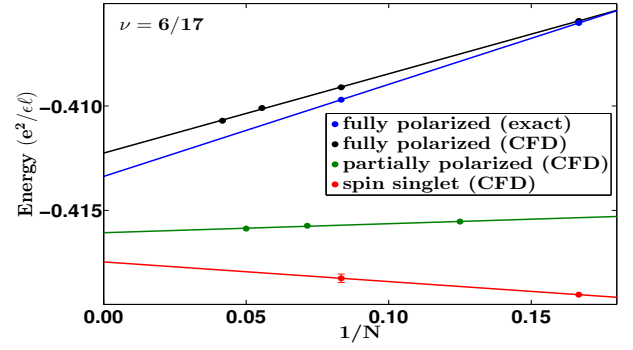
FIG. 10: Thermodynamic extrapolation of the lowest Landau level Coulomb ground state energy for different spin polarized states at \nu = 6/17 .
