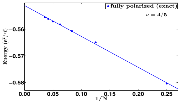
FIG. 4: Thermodynamic extrapolation of the lowest Landau level Coulomb ground state energy for the fully spin polarized state at \nu = 4/5 .
