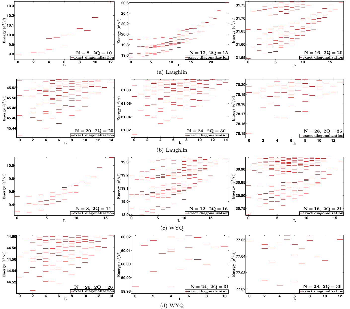
FIG. 3: Coulomb spectra obtained from exact diagonalization in the spherical geometry for N fully spin polarized electrons at \nu = 4/5 at the total flux 2Q(hc/e) corresponding to the Laughlin (top two panels (a) and (b)) and WYQ state (bottom two panels (c) and (d)).
