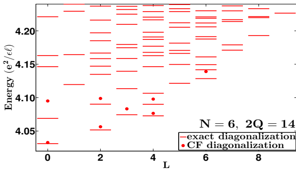
FIG. 9: Coulomb spectra in the spherical geometry for N electrons with total spin S = 0 at flux 2Q(hc/e) at \nu = 6/17 . The red dashes (dots) show the energies obtained from exact (CF) diagonalization.
