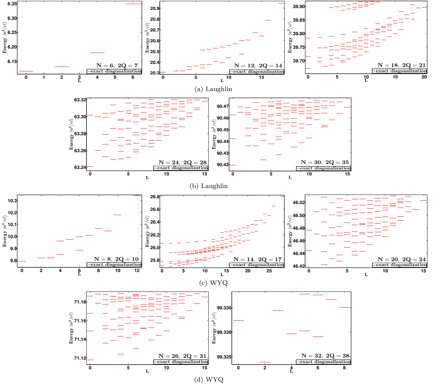
FIG. 11: Coulomb spectra obtained from exact diagonalization in the spherical geometry for N fully spin polarized electrons at \nu = 6/7 at the total flux 2Q(hc/e) corresponding to the Laughlin (top two panels (a) and (b)) and WYQ state (bottom two panels (c) and (d)).
