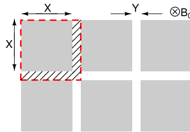
FIG. 9. (Color online) An array of square superconducting aluminium films. A magnetic field is applied perpendicular to the surface of the films. The enclosed area by dashed line indicates one unit cell.
