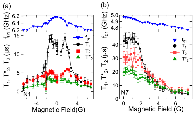
FIG. 6. (Color online) The qubit transition frequencies ( f_{01} ) and three time scales ( T_1, T_2^* , and T_2 ) were measured at the sweet spots over the wide range of magnetic field for the N1 (a) and N7 (b).
