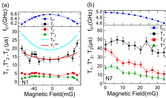
FIG. 5. (Color online) (a) Magnetic field dependence of the N1 qubit frequency ( f_{01} ), three measured time scales ( T_1, T_2^* , and T_2 ) and two calculated time scales ( T_P and T_1^{\text{cal}} ) at low magnetic field, much smaller than the SQUID oscillation period. T_P (Purcell time) was calculated by T_P = 1/\Gamma_P . Here \Gamma_P is the Purcell rate related to the fundamental resonance mode of the cavity, and T_1^{\text{cal}} by 1/T_1^{\text{cal}} = 1/T_{\text{other}} + 1/T_P (see texts) (b) The qubit frequency and three measured time scales for N7.
