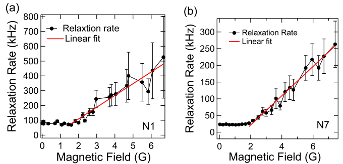
FIG. 7. (Color online) The relaxation rates \Gamma=1/T_1 versus magnetic field were plotted for both N1 (a) and N7 (b). All measurements have been done at the sweet spots. The linear fits (red solid lines) were shown over the magnetic field range where the vortices were present in the electrodes.
