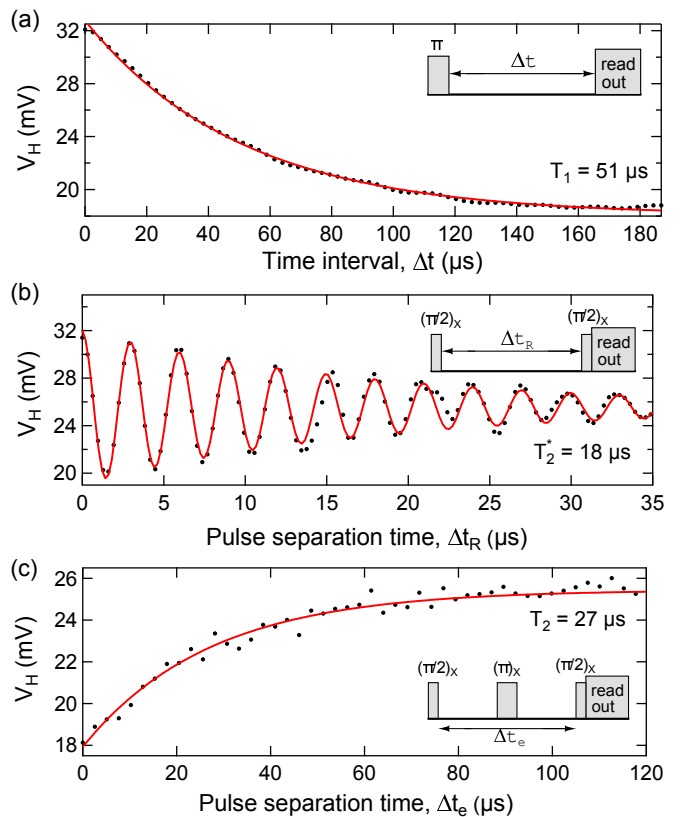
FIG. 4. (Color online) Time domain measurements of the N7 sample at B = 7.5 \text{ mG} . (a) Relaxation time measurement ( T_1 = 51 \mu\text{s} ) (b) Ramsey fringe experiment ( T_2^* = 18 \mu\text{s} ) (c) Hahn spin echo experiment ( T_2 = 27 \mu\text{s} ). The red solid lines are the fits to the data. See the main text for the fitting functions.
