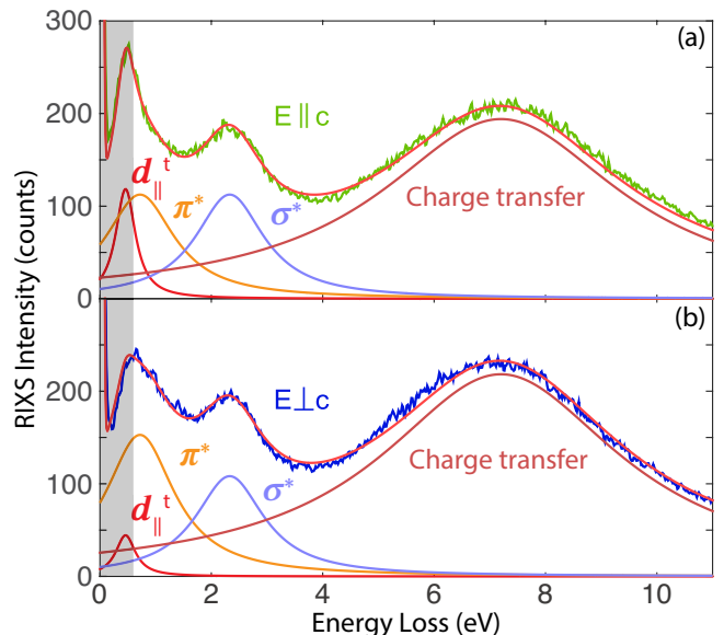
FIG. 4: Polarization dependence and feature attribution: Four-Lorentzian fits of the experimental data measured with incident polarization (a) parallel and (b) perpendicular to the c_R -axis. The band gap of bulk \text{VO}_2 is shaded in to highlight likely in-gap states. Three low energy features nominally represent the singlet-triplet mode ( d_{\parallel}^t at E_t=0.46 eV, width \Gamma=0.43 eV), and dd excitations into non-bonding \pi^* ( t_{2g} ) orbitals ( E=0.72 eV, \Gamma=1.5 eV) and \sigma^* ( e_g ) orbitals ( E=2.33 eV, \Gamma=1.5 eV). The broad feature at E=7.2 eV is attributed to metal-ligand charge transfer excitations ( E=7.2 eV, \Gamma=5.25 eV). The singlet-triplet excitation constitutes 23% weight of the combined d_{\parallel}^t/\pi^* feature when polarization is parallel to the c_R -axis, and just 8% under orthogonal polarization.
