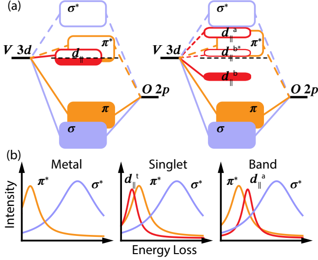
FIG. 1: Orbital symmetries of VO 2 electronic states: (a) Orbital symmetries of electronic states are labeled for (left) the high-temperature metallic state and (right) the low-temperature insulating state, with the Fermi level indicated by a dashed line. The labels d_{\parallel}^t and d_{\parallel}^a indicate gapped d_{\parallel} -symmetry states expected in the M1 phase. (b) Schematics show anticipated RIXS excitations that could be achieved by changing the symmetry of a d_{\parallel} electron. Scenarios are presented for (left) the rutile metal and for hypothetical M1 insulating states based on (middle) strongly correlated singlets and (right) itinerant Peierls band physics.
