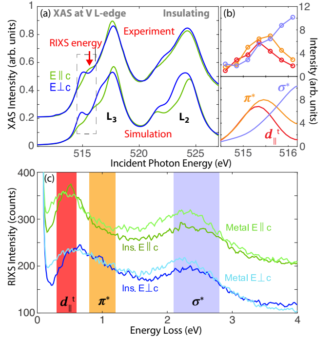
FIG. 2: XAS and RIXS across the metal-insulator transition: (a) (top) Experimental and (bottom) theoretical XAS spectra of M1 phase VO 2 are shown for two incident photon polarization conditions. (b) (top) The M1 phase \mathbf{E} \parallel \mathbf{c}_R incident energy dependence of highlighted energy loss windows in panel (c) is compared with (bottom) simulations for the d_{\parallel}^t , \pi^* , and \sigma^* excitations. Statistical error bars are slightly smaller than the plotted circles, and simulation curves are weighted to match the integration windows, as described in the SM [20]. (c) RIXS spectra in the insulating and metallic states at temperatures T=260 K and 320 K, respectively. The two \mathbf{E} \parallel \mathbf{c}_R curves are upward offset by 100 counts.
