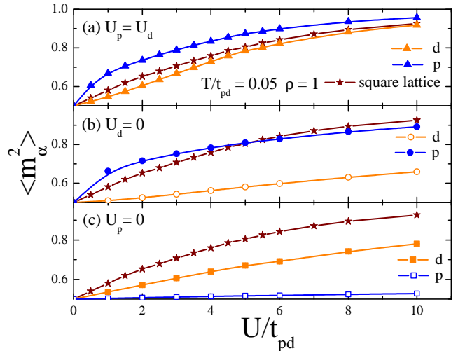
FIG. 10. (Color online) Local moment on d sites [light (orange) color] and on p sites [dark (blue) color], as functions of the on-site repulsion for (a) the homogeneous case, (b) U_p = U , U_d = 0 , and (c) U_d = U , U_p = 0 . Data for the usual square lattice are also shown (stars), for comparison.
