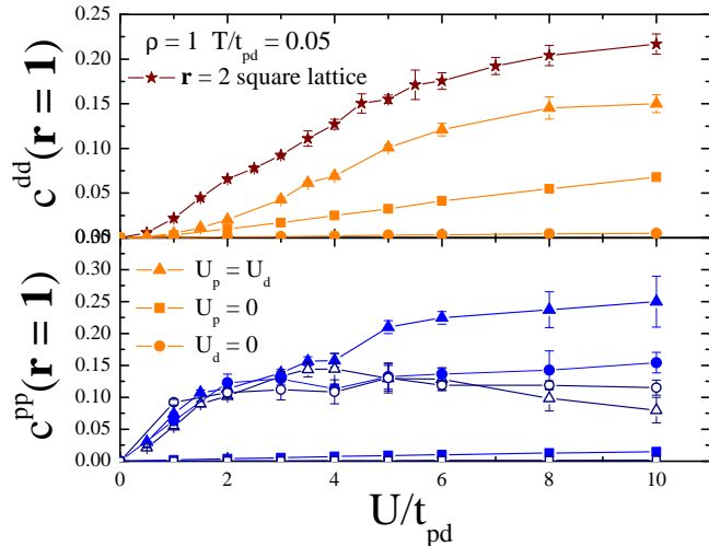
FIG. 11. (Color online) Spin correlations between first neighbor like-sites. The upper panel displays the correlations between d sites, while the lower panel shows those between p sites; in the latter case, the p sites may have an intervening d site (filled symbols), or not (empty symbols). Data for the usual square lattice are shown, but the fair comparison in this case is with sites on different sublattices (hence two lattice spacings apart, or r = 2 ); see text.
