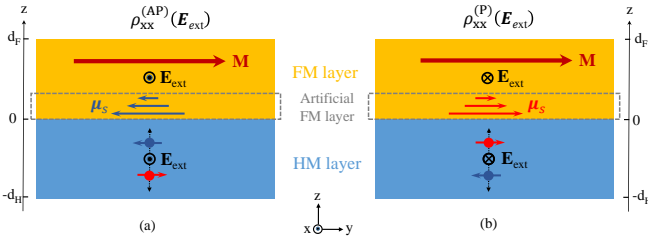
FIG. 1. Schematic diagrams showing the mechanism of non-linear longitudinal resistivity in HM/FM bilayers due to spin accumulation in the FM layer induced by spin Hall effect in the HM layer. The external electric field \mathbf{E}_{ext} is applied in the positive x -direction in (a) and in the negative x -direction in (b). The dotted arrows in the HM layer denotes the directions of the spin Hall currents. The solid arrows in the grey dashed boxes describe the magnitude and direction of the spin accumulation \mu_s which may be regarded as an artificial FM layer. The difference in longitudinal resistivity of the bilayer in antiparallel (a) and parallel (b) configurations arises from the spin-dependence of the mobility in the FM layer in analogy with CIP-GMR.
