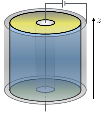
FIG. 1: (Color online) Schematic of the topological coaxial cable geometry. The axion insulator (blue) is enclosed in a cylindrical capacitor (silver). A voltage applied to the capacitor creates the axial gauge field vortex (5) in the axion insulator through RSOC. Annular contacts (gold) are placed on both ends to measure the longitudinal conductance, allowing current to be carried through the vortex and edge modes. The number of such modes is dependent on the voltage across the capacitor.
