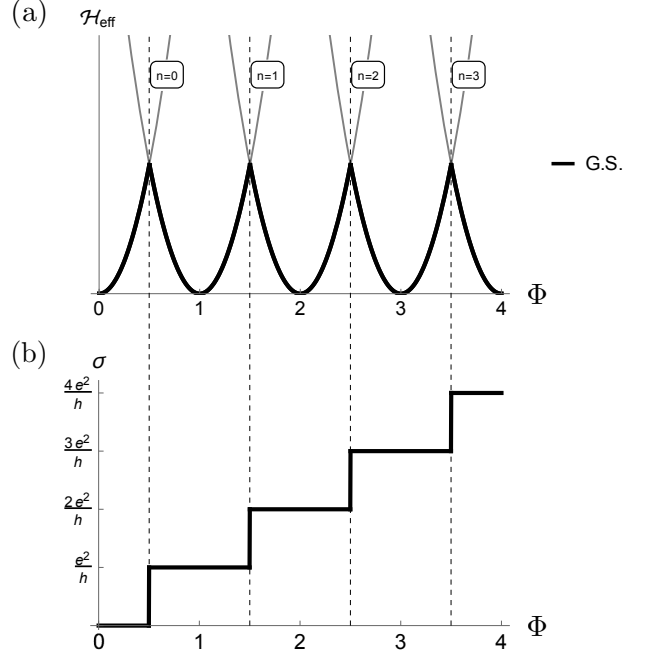
FIG. 2: (a) Energy of the effective Hamiltonian plotted against the applied axial gauge field strength \Phi for the lowest few vorticities n of \Delta , as given by Eq. (8). This energy is minimized when n is the nearest integer to \Phi (the thick black line). (b) Longitudinal conductivity \sigma of the topological coaxial cable plotted against the applied axial gauge field strength \Phi . The conductivity is a step-function in \Phi , with jumps when \Phi takes half-integer values, corresponding to changes in the vorticity n which minimizes the effective Hamiltonian. Dashed lines highlight this correspondence.
