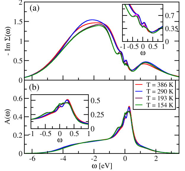
FIG. 11. (color online) (a) Imaginary part of the self-energy (b) single particle spectral function on the real frequency axis obtained from the maximum entropy method for different temperatures and U = 2.3 eV, J = 0.5 eV.
