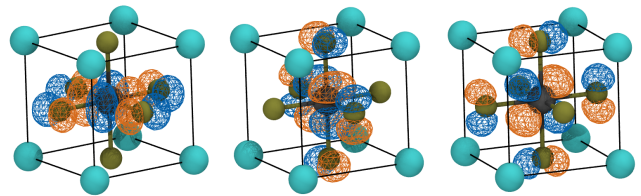
FIG. 3. (color online) Orbital plots of maximally localized Wannier functions used to reproduce the low energy subspace Hamiltonian.
