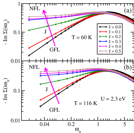
FIG. 5. (color online) Imaginary part of the Matsubara self energy ( -\text{Im}\Sigma(i\omega_n) ) for U = 2.3 eV and different J values for (a) T=60 K (b) T=116 K.
