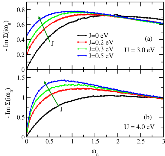
FIG. 6. (color online) Imaginary part of the self energy for T=60 K and different J values (see legend) with (a) U = 3 eV, and (b) U = 4 eV.
