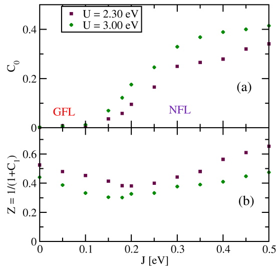
FIG. 8. (color online) Imaginary part of the self energy ( -\text{Im} \Sigma(i\omega_n) ) fitted to a fourth order polynomial: (a) zeroth order coefficient, C_0 (b) Z = 1/(1 + C_1) , where C_1 is the linear coefficient, for different J values, U=2.3 and 3.0 eV and T = 60 K.
