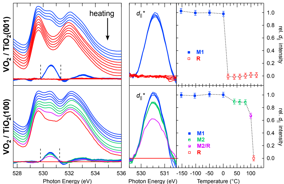
FIG. 2: (Left) Temperature dependent O K-edge XAS measurements of \text{VO}_2/\text{TiO}_2(001) and \text{VO}_2/\text{TiO}_2(100) with (right) an expanded view of the d_{\parallel} feature and its peak intensity as a function of temperature.
