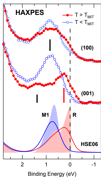
FIG. 5: Valence band HAXPES of VO 2 /TiO 2 (100) and VO 2 /TiO 2 (001) collected above and below T_{MIT} . (Bottom) HSE06 hybrid DFT calculations showing the total DOS for the M1 and R phase. Solid bars indicate the coherent (red) and incoherent (black) contributions to the V 3d feature.
