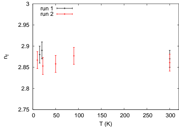
FIG. 6: Total 5f occupancy estimate n_f of URu 2 Si 2 as a function of temperature from both experimental runs. The lowest measured temperature is 10 K. No measurable temperature dependence was observed. Taking all these data together and allowing for some systematic error gives n_f = 2.87 \pm 0.08 .
