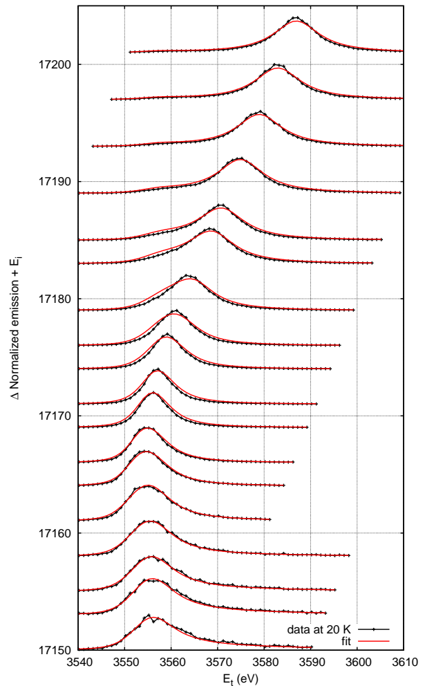
FIG. 5: RXES data and fit at 20 K for \text{URu}_2\text{Si}_2 .
