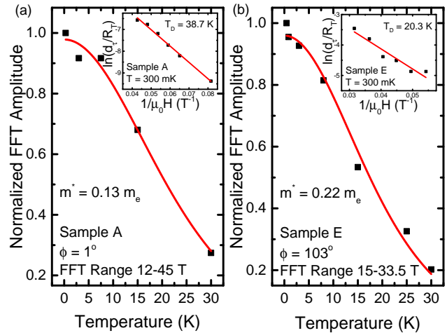
FIG. 4. (color online) (Panel a) The temperature dependence of the oscillation amplitude of Sample A at \phi = 1^\circ . (Panel b) The temperature dependence of the oscillation amplitude of Sample E at \phi = 103^\circ . The insets are the Dingle-fits of the oscillation amplitude, with the vertical axis the ratio of the log of the oscillation amplitude and the thermal damping factor.
