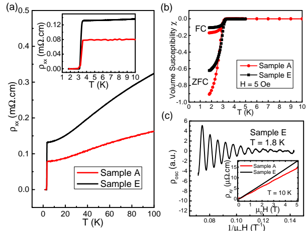
FIG. 2. (color online) The superconducting signal and transport properties of two Nb doped \text{Bi}_2\text{Se}_3 crystals. (Panel a) The resistivity of Sample A and E as a function of temperature, T . (Panel b) Volume magnetic susceptibility of Nb-doped \text{Bi}_2\text{Se}_3 crystals, measured in Zero-Field-Cool (ZFC) and Field-Cool (FC) conditions. For Sample A, the Meissner effect in the ZFC condition reaches close to -1, indicating a nearly 100% superconducting volume. (Panel c) Shubnikov-de Haas oscillations in Sample E with field along the sample crystalline c -axis. The inset shows the Hall signal from the two samples.
