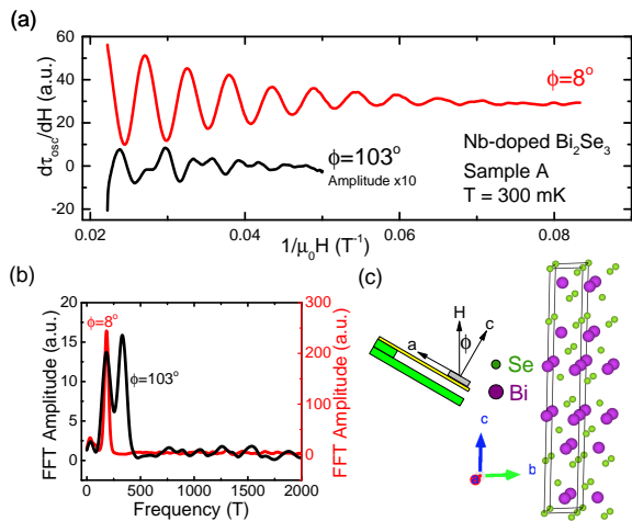
FIG. 1. (color online) (Panel a) Derivative of oscillatory magnetic torque of Nb-doped \text{Bi}_2\text{Se}_3 . Torque from Sample A is plotted against inverse magnetic field 1/\mu_0 H . A polynomial background has been subtracted from the torque \tau-H curves to obtain the oscillatory torque \tau_{osc} and the derivative with respect to field was taken to emphasize the oscillation signal. The top curve in red is taken at tilt angle of magnetic field around 8^\circ and shows 1 oscillation frequency. The lower curve in black is taken at tilt angle of magnetic field around 103^\circ and shows 2 oscillation frequencies. The amplitude of the second curve is multiplied by a factor of 10 and the two curves have been shifted apart for clarity. (Panel b) The Fast Fourier Transformation (FFT) of the two \tau_{osc}-1/\mu_0 H traces. (Panel c) A sketch of the torque magnetometry setup is shown together with the crystal structure of \text{Bi}_2\text{Se}_3 to demonstrate the magnetic field rotation plane.
