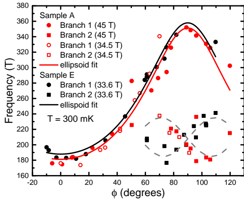
FIG. 3. (color online) Comparison of the angular dependence of the oscillation frequencies of Nb-doped \text{Bi}_2\text{Se}_3 in Sample A (red) and Sample E (black) taken at T = 300 mK. The solid lines are fits for ellipsoidal Fermi Surfaces. The dashed lines are guides for eyes for the second Fermi Pocket. The maximum magnetic field used in each run is labeled in the legend.
