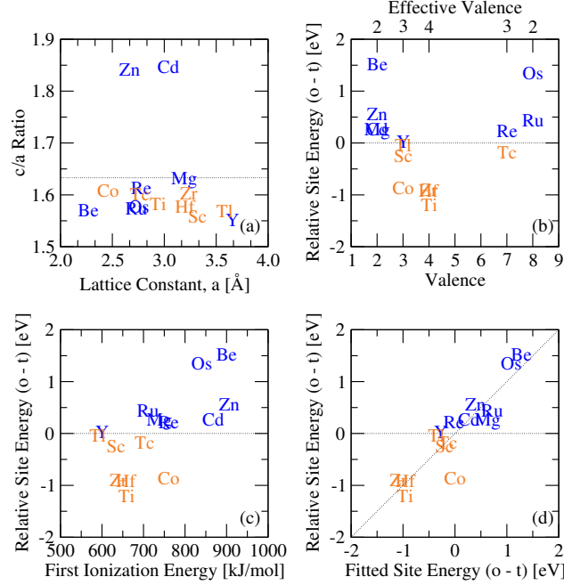
FIG. 6. (color online). Correlation between the relative oxygen interstitial site energy and physical properties of the 15 HCP elements. Each elemental symbol is centered on the corresponding data for that element. a) Comparison of the lattice constant and the c/a ratio for the HCP elements. The dotted line represents the ideal HCP c/a = 1.633 . b) Correlation between the octahedral–tetrahedral/hexahedral energy difference and the common metal valence as well as the effective valence. c) Correlation between the octahedral–tetrahedral/hexahedral energy difference and the first ionization energy. d) Linear regression fit ( R^2 = 0.8240 ) of the DFT relative site energies to the c/a ratio, the effective valence, and the first ionization energy. The primary outlier is Co, due to its magnetic ordering. The effective valence is determined according to crystal-field splitting. HCP elements are colored according to the oxygen ground-state configuration in that element, orange for octahedral site and blue for tetrahedral/hexahedral site.
