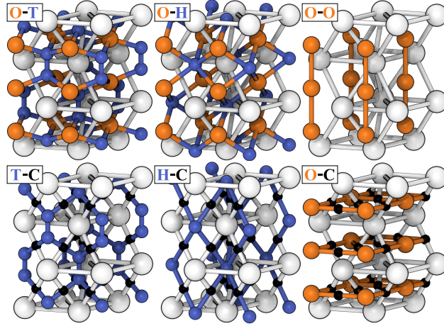
FIG. 2. (color online). Connectivity network for transitions between interstitial sites in the HCP lattice. Note that the O-T and T-C networks also include T-T transitions between neighboring tetrahedral sites. White spheres represent the HCP lattice atoms, orange for octahedral, blue for tetrahedral and hexahedral, and black for crowdion interstitial sites.
