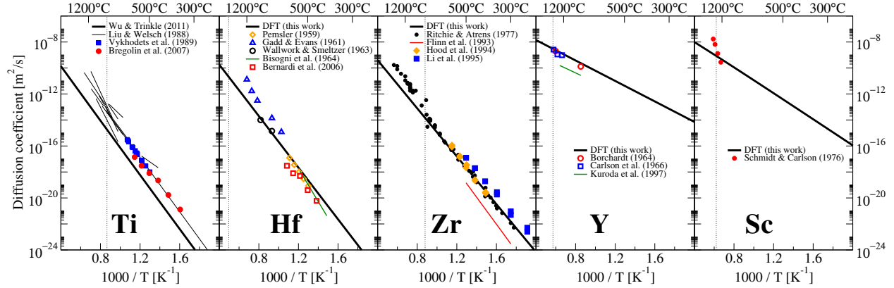
FIG. 4. (color online). Comparison between our DFT predicted and experimentally measured oxygen diffusivity in \text{Ti}^{5-7} , \text{Hf}^{8-12} , \text{Zr}^{13-16} , \text{Y}^{17-19} , and \text{Sc}^{20} . We have previously reported the DFT data for oxygen diffusion in titanium 21 , while the other DFT predictions are from this work. For Ti, the data labeled as Liu and Welsch comes from their review paper covering experiments ranging from 1957-1983. For Zr, the data labeled as Ritchie and Atrens comes from their review paper, the data points plotted only includes experiments without the effect of grain boundary diffusion. The vertical dotted lines show the \alpha - \beta transition temperatures for each element: 1155K for Ti, 2016K for Hf, 1137K for Zr, 1751K for Y, and 1610K for Sc.
