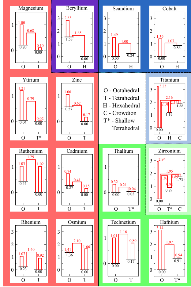
FIG. 3. (color online). Oxygen interstitial site energies and diffusion barriers in all 15 HCP elements. Energy in units of eV is represented on the vertical axis, while possible metastable interstitial sites for each element is placed on the horizontal axis. The elements are grouped by commonalities of interstitial stability; on the right, elements have the octahedral interstitial site as the ground-state configuration, while elements on the left do not. The dotted line separate elements with hexahedral sites (Be, Co, Sc, and Ti) versus elements with tetrahedral sites. The dashed line separate elements with crowdion sites (Ti and Zr) versus elements that do not. Relative site energies are given in black, while possible transitions between sites are connected by red lines with the respective saddle point energies given in red, also relative to the ground-state configuration energy. Some tetrahedral sites are labeled shallow tetrahedral (T*) due to the low T-T transition barrier in that element.
