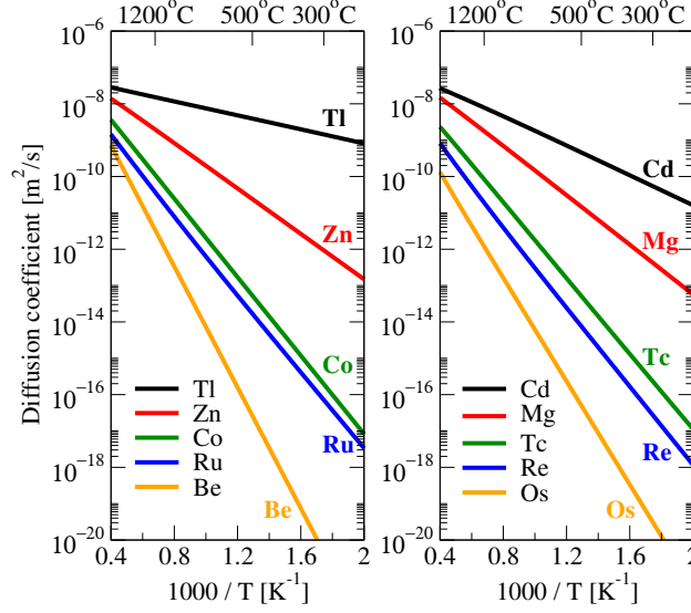
FIG. 5. (color online). DFT oxygen diffusion predictions for the remaining 10 HCP elements. No experimental data were found in the literature.
