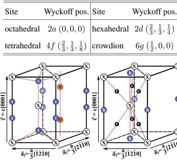
FIG. 1. (color online). Wyckoff positions and unit cell locations for oxygen interstitial sites in HCP systems. On the left: o ctahedral (orange) and t etrahedral (blue). On the right: h exahedral (blue) and c rowdion (black).
