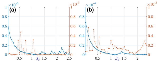
Figure 8: Relative differences of S_{1,501}^z (blue) calculated for J_{xy} = 1 , \alpha = 2 and \langle S_1^+ S_{501}^- \rangle (red) calculated for J_{xy} = -1 , \alpha = 2 caused by (a) increasing L from 5000 to 10^4 (with K increasing from 9 to 10) and (b) decreasing \epsilon_f from 10^{-10} to 10^{-11} (with K increasing from 9 to 10).
