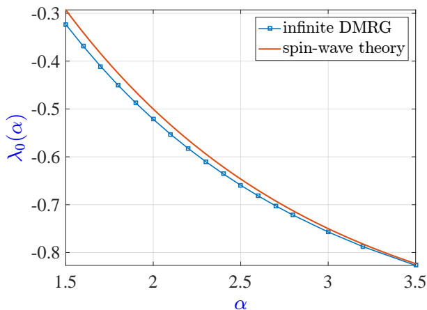
Figure 2: Comparison of the (first-order) transition point \lambda_0(\alpha) out of the FM phase calculated using infinite-size DMRG and spin-wave theory for J_{xy} = 1 . The spin-wave theory predicts \lambda_0(\alpha) = -\eta(\alpha)/\lambda(\alpha) . The infinite-size DMRG calculations use a bond dimension \chi = 100 , and increasing \chi to 200 does not yield results distinguishable within the resolution of the plot. The transition point is numerically determined by finding the value of J_z at which the ground state energy density obtained from infinite-size DMRG calculations is equal to that of the FM state.
