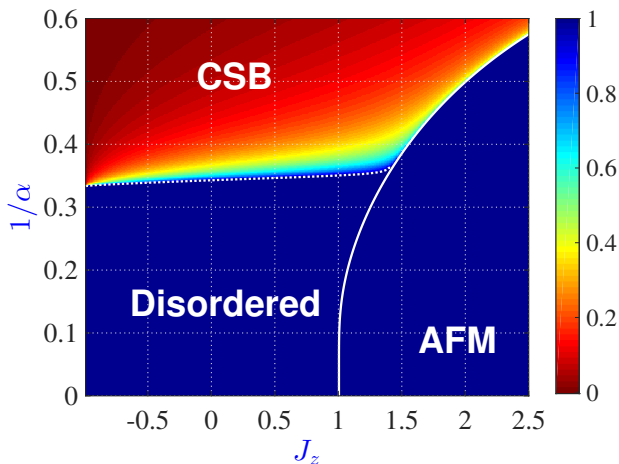
Figure 5: Spin-wave excitation density \langle a_i^\dagger a_i \rangle calculated using Eq. (14) for an infinite-size chain. For J_z > \zeta(\alpha)/\eta(\alpha) (region to the right of the white line), imaginary frequencies appear in the Bogoliubov spectrum, indicating a classical instability toward the AFM phase. The region above the dotted and solid white lines has \langle a_i^\dagger a_i \rangle \leq 1 , and is associated with the CSB phase. The remaining region in the plot has \langle a_i^\dagger a_i \rangle > 1 , and is expected to be disordered. The disordered phase can be either the XY or the Haldane phase, but the spin-wave theory cannot distinguish one from the other. For better visibility, we have set \langle a_i^\dagger a_i \rangle = 1 for regions without CSB in the plot.
