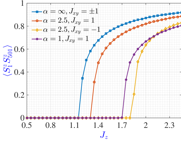
Figure 4: \langle S_1^z S_{501}^z \rangle as a function of J_z calculated using infinite-size DMRG for a few different sets of \alpha and J_{xy} . The Haldane-to-AFM phase transition is clearly observed and we locate the transition point by finding the critical J_z (restricted to J_z > 0 ) above which \langle S_1^z S_{501}^z \rangle > 0.1 . The curves shown look identical when we increase the bond dimension used from 100 to 200.
