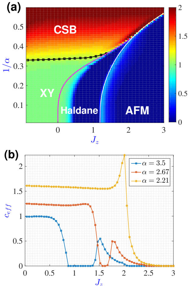
Figure 6: Calculation of the effective central charge c_{\text{eff}} as a function of J_z and \alpha for J_{xy} = -1 , extracted from finite-size DMRG calculations with N_1 = 100 , N_2 = 110 , and a maximum bond dimension of 500. (a) The black squares (fitted by the black line) show where c_{\text{eff}} starts to deviate from 1 when going from the XY to the CSB phase. The purple line and white line are from Fig. 3, and show the boundaries of the Haldane phase. (The calculation of c_{\text{eff}} is inaccurate in predicting the location of the XY-to-Haldane transition due to strong finite-size effects 61,86–88 .) For better contrast, locations with c > 2 are shown with the color corresponding to c = 2 . (b) For our finite-size chains, the XY-to-Haldane BKT phase transition is signaled by a continuous drop of c_{\text{eff}} from 1 to 0 ( \alpha = 3.5 ). The Haldane-to-AFM phase transition is identified by a peak with value around 0.5 in c_{\text{eff}} ( \alpha = 3.5 and \alpha = 2.67 ). The CSB-to-Haldane transition is expected to be continuous and not associated with a central charge ( \alpha = 2.67 ). The CSB-to-AFM transition has a sharp peak in c_{\text{eff}} ( \alpha = 2.21 ), an indication of a first-order transition 67 .
