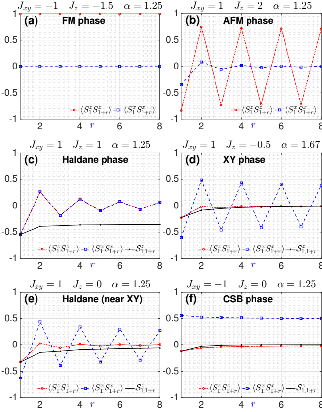
Figure 7: Signatures of all five phases for a N = 16 spin chain. Except for (e), we tune J_{xy} , J_z and \alpha to set the ground state deep into each phase. Each phase is distinguished from the other phases by different behaviors in various spin-spin correlation functions.
