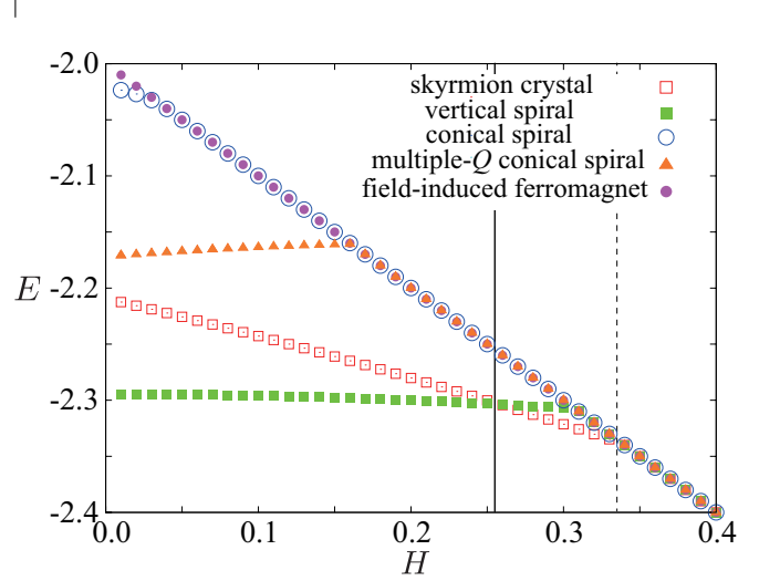
FIG. 2. (Color online) H dependence of the energy per site of different variational states for Q = 2\pi/5 and A = 0.5 . The vertical solid line marks the phase boundary between the single- \mathbf{Q} vertical spiral and skyrmion crystal phases. The vertical dashed line marks the phase boundary between the skyrmion crystal and fully polarized state. Here we only considered the multiple- \mathbf{Q} conical spiral with I_x = I_y .
