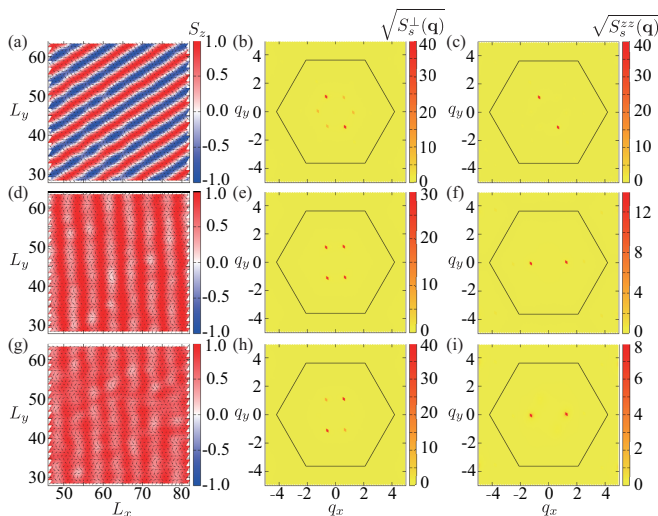
FIG. 7. (Color online) Snapshots of spin configurations and the square root of the spin structure factor for Q = 2\pi/5 , T = 0.02 and N = 75 \times 75 spins. (a)-(c) Multiple- \mathbf{Q} vertical spiral obtained for A = 0.03 and H = 0.19 , (d)-(f) multiple- \mathbf{Q} conical spiral with equal transverse amplitudes, I_x = I_y , obtained for A = 0.05 and H = 0.64 , and (g)-(i) Multiple- \mathbf{Q} conical spiral with different transverse amplitudes, I_x \neq I_y , obtained for A = 0.02 and H = 0.67 .
