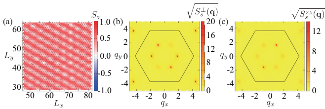
FIG. 9. (Color online) (a) Snapshot of spin configuration and (b)-(c) the square root of the spin structure factor of the multiple- \mathbf{Q} conical spiral in Fig. 8(a). The Hamiltonian parameters are Q = 2\pi/5 , A = 0.2 , H = 4.4 , T = 0.6 and the system size is N = 75 \times 75 . The snapshot of the spin configuration in (a) is obtained after averaging over 500 MCS to integrate out the short wavelength fluctuations. The field-induced \mathbf{q} = 0 component of the structure factor has been omitted in (b) and (c).
