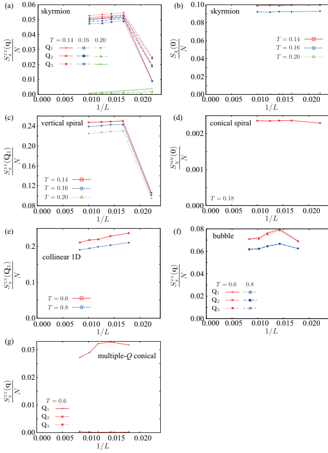
FIG. 10. (Color online) Size dependence of the order parameters for each phase: (a) z -component of the spin structure factor evaluated at \mathbf{q} = \mathbf{Q}_1, \mathbf{Q}_2, \mathbf{Q}_3 and (b) chirality structure factor evaluated at \mathbf{q} = \mathbf{0} ( S_\chi(\mathbf{q}) = S_\chi^{uu}(\mathbf{q}) + S_\chi^{dd}(\mathbf{q}) ) for Q = 2\pi/5 , H = 0.25 , A = 0.5 , and different temperatures in the skyrmion crystal phase ; (c) z -component of the spin structure factor evaluated at \mathbf{q} = \mathbf{Q}_1 for Q = 2\pi/5 , H = 0.0 , A = 0.5 in the vertical spiral state ; (d) chirality structure factor for the upward triangles of the triangular lattice evaluated at \mathbf{q} = \mathbf{0} for Q = 2\pi/5 , H = 0.4 and A = 0.02 in the conical spiral state ; (e) z -component of the spin structure factor with \mathbf{q} = \mathbf{Q}_1 for Q = 4\pi/7 , H = 0.0 , and A = 2.0 in the collinear 1D state ; (f) z -component of the spin structure factor evaluated at \mathbf{q} = \mathbf{Q}_1, \mathbf{Q}_2, \mathbf{Q}_3 for Q = 4\pi/7 , H = 2.0 and A = 2.0 in the bubble crystal phase ; (g) z -component of the spin structure factor evaluated at \mathbf{q} = \mathbf{Q}_1, \mathbf{Q}_2, \mathbf{Q}_3 for Q = 4\pi/7 , H = 4.4 and A = 0.2 in the multiple-Q conical state .
