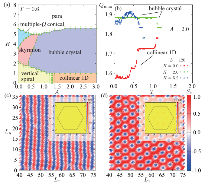
FIG. 8. (Color online) (a) A - H phase diagram of the J_1 - J_3 model at T = 0.60 and for Q = 4\pi/7 ( J_3 \sim 1.62 ). (b) T -dependence of the ordering-vectors of the collinear 1D and BC phases ( A = 2.0 ). The horizontal line corresponds to Q = 4\pi/7 . Panels (c) and (d) show typical spin configurations for the collinear 1D and BC phases, respectively. The insets of panels (c) and (d) show S_s^{zz} .
