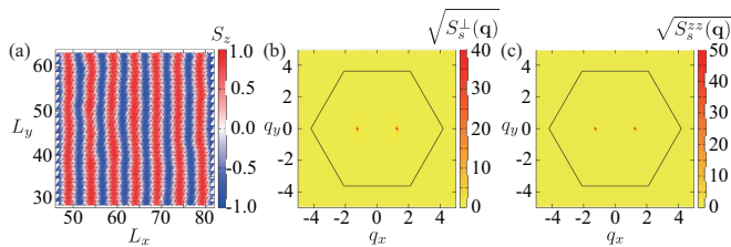
FIG. 4. (Color online) Snapshots of spin configurations and the corresponding spin structure factor of the vertical spiral appearing in Fig. 3(b) for Q = 2\pi/5 and N = 100 \times 100 . The data are taken for A = 0.5 , H = 0.15 , and T = 0.15 . In (a), we average over 500 MCS to integrate out the short wavelength fluctuations. Panels (b) and (c) show the square root of the xy and z components of the spin structure factor, respectively. Here and hereafter, the field-induced \mathbf{q} = 0 component is subtracted for clarity.
