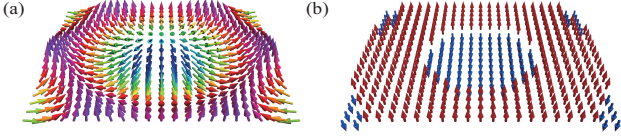
FIG. 1. (Color online) Schematic views of (a) a noncoplanar skyrmion texture and (b) a collinear bubble. Triangular crystals of these structures are induced by magnetic field and easy-axis anisotropy in high-symmetry frustrated magnets.
