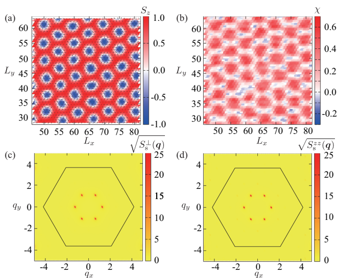
FIG. 5. (Color online) Snapshot of the real-space (a) spin configuration and (b) scalar chirality in the skyrmion crystal phase for H = 0.27 and T = 0.15 in Fig. 3(b). The color scale in (a) indicates the z spin component, parallel to H , while the arrows indicate the in-plane xy components. The lattice size is L = 100 and the MC results are obtained after averaging over 500 MCS. Panels (c) and (d) show the xy and z components of the spin structure factor, respectively.
