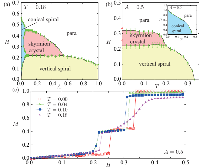
FIG. 3. (Color online) (a) A - H phase diagram obtained from MC simulations of the J_1 - J_3 model for J_3/|J_1| = 0.5 at T = 0.18 . (b) T - H phase diagram for A = 0.5 . The red triangles are determined from T = 0.0 variational calculations. The inset shows the phase diagram for A = 0.0 . (c) Field dependence of the magnetization at different temperatures for A = 0.5 . The error bars are smaller than the symbol size.
