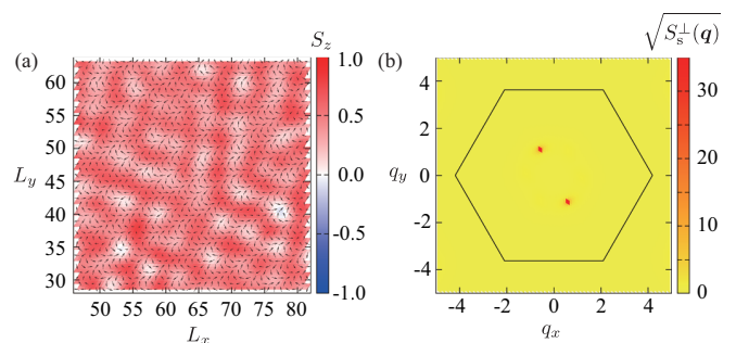
FIG. 6. (Color online) (a) Snapshot of the spin configurations and (b) the square root of the xy component of the spin structure factor for the conical spiral phase in Fig. 3(a). The Hamiltonian parameters are Q = 2\pi/5 , A = 0.02 , H = 0.43 , T = 0.18 and the lattice size is N = 75 \times 75 . The snapshot of the spin configuration in (a) is obtained after averaging over 2000 MCS in order to integrate out the short wavelength fluctuations. The field-induced \mathbf{q} = 0 component of the spin structure factor has been omitted in (b). Note that the z -spin component remains uniform in the conical spiral state.
