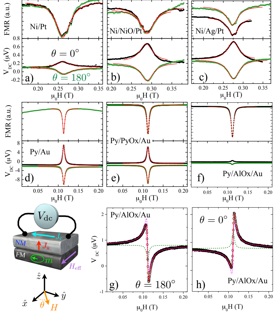
FIG. 4. Inverse spin Hall effect measurements via spin pumping excited by cavity FMR. Top plots of panels a-f ) show the FMR response as a function of field with 9.85 GHz microwave excitation. Bottom plots show the dc spin pumping voltage measured on the NM layer as a function of field. a) Ni/Pt, b) Ni/NiO/Pt, c) Ni/Ag/Pt, d) Py/Au, e) Py/PyOx/Au, f) Py/AlOx/Au. Note that presence of the native oxide in both series slightly increases the total \Delta V_{\text{ISH}} (see text), and that the Py/Au series generates large \Delta V . For only the Py/AlOx/Au, the film stack could not be placed exactly at the node of the electric field, and V_{\text{DC}} is dominated by a rectification-driven asymmetric (peak-dip) component. f) shows the spin pumping component extracted by fit from the raw signals shown in g) and h) . In g) and h) symbols are measured V_{\text{DC}} , solid red lines the fit, and dashed lines show the separate symmetric and anti-symmetric components.
