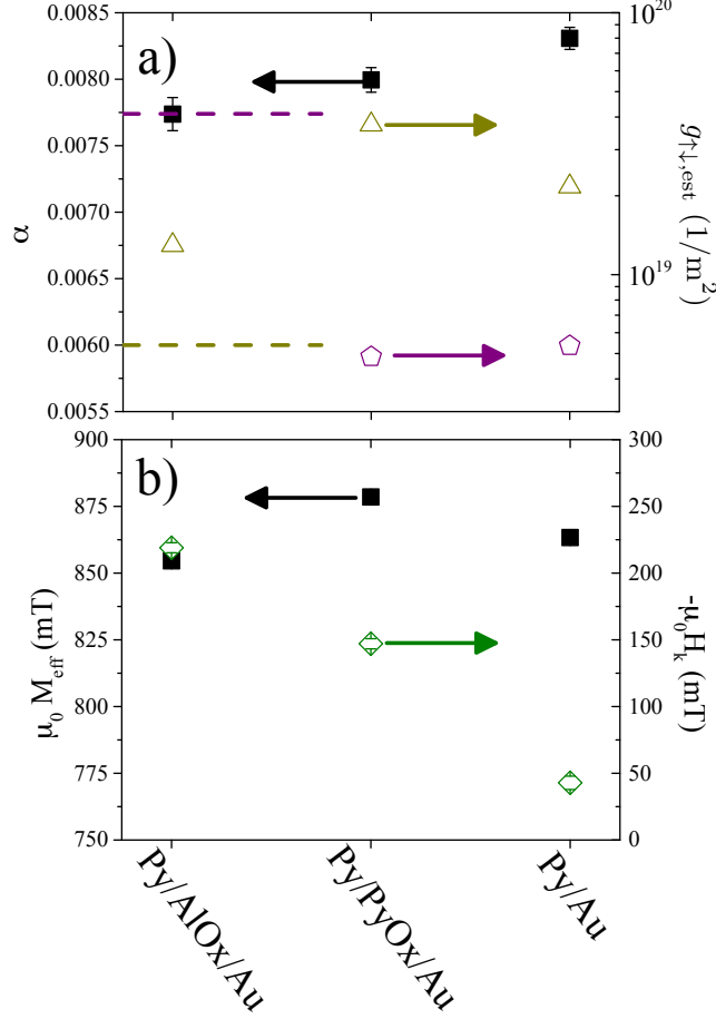
FIG. 10. Room temperature trends in a) \alpha (filled square), and g_{\uparrow,\text{eff}} (open triangle: for intrinsic damping = 0.006, open pentagon: for intrinsic damping = 0.0077), and b) M_{\text{eff}} (filled square) and H_k (open diamond) for the Py/Au sample series. Trends in \alpha here are in line with a spin-pumping origin, and we use two different estimates of intrinsic damping \alpha_0 to estimate the spin-mixing conductance independent from the electrically-detected spin pumping measurement. These values of g_{\uparrow,\text{eff}} fall in the range expected for transition-metal FM/NM interfaces.
