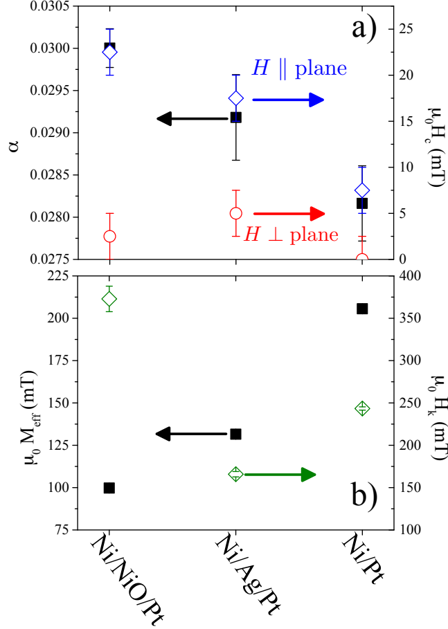
FIG. 9. Room temperature trends in a) \alpha (filled square), and H_c (both in-plane (open diamond) and out-of-plane (open circle)), and b) M_{\text{eff}} (filled square) and H_k (open diamond) for the Ni/Pt sample series. Trends in \alpha are similar to those in H_c , and suggest changes in damping are tied to magnetic anisotropy, rather than to spin pumping.
