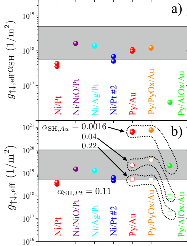
FIG. 11. a) g_{\uparrow\downarrow, \text{eff}}\alpha_{\text{SH}} calculated for each sample using Eqs. 11 or 13. All samples show relatively similar values other than Py/AlOx/Au, which is strongly suppressed as expected. b). g_{\uparrow\downarrow, \text{eff}} calculated from g_{\uparrow\downarrow, \text{eff}}\alpha_{\text{SH}} using assumed values for \alpha_{\text{SH}} . For Pt samples the commonly reported \alpha_{\text{SH}, \text{Pt}} = 0.11 gives g_{\uparrow\downarrow, \text{eff}} in the expected range. For Au, we use three values of \alpha_{\text{SH}, \text{Au}} . Values on order of tenths of percent give very large g_{\uparrow\downarrow, \text{eff}} , even for the sample with the AlOx layer. \alpha_{\text{SH}, \text{Au}} of several percent or more yields g_{\uparrow\downarrow, \text{eff}} in line with expectations for transition metal FM/NM interfaces.
