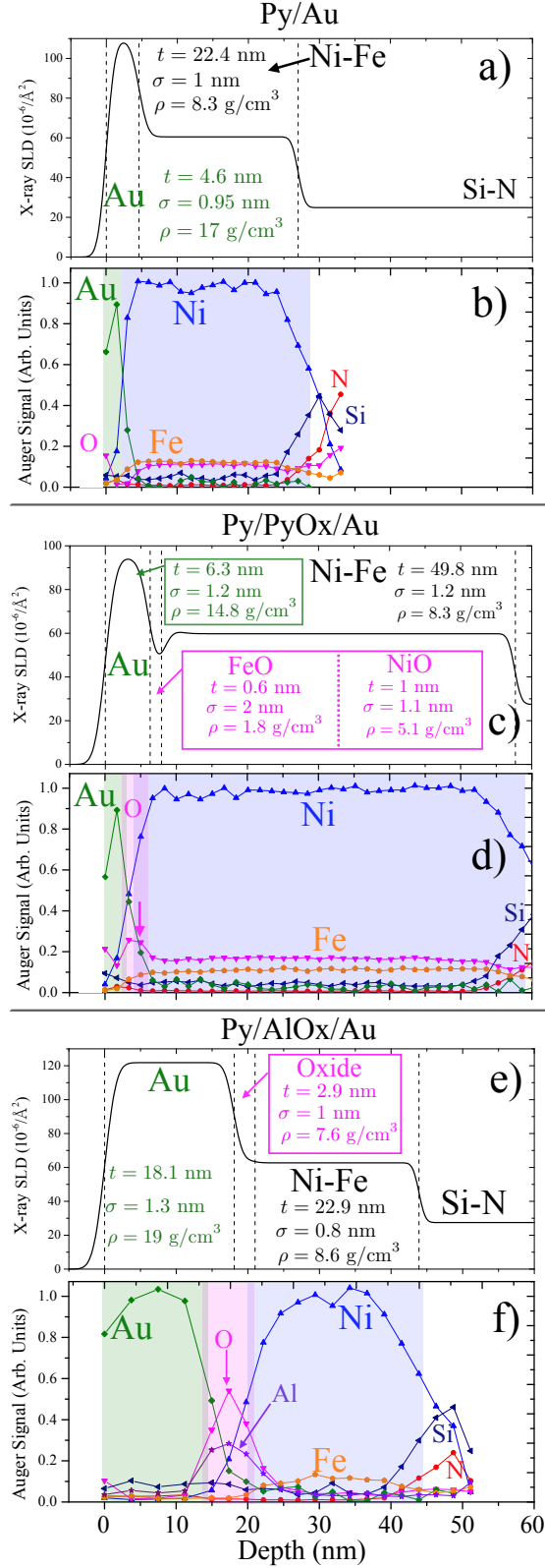
FIG. 3. Refined X-ray scattering-length density (SLD) and depth-profiled Auger electron spectroscopy for a-b) Py/Au, c-d) Py/PyOx/Au, e-f) Py/AlOx/Au heterostructures. Py layers left exposed to atmosphere for \sim 24 hours between FM and NM layer deposition show clear accumulation of O Auger electron signal localized to the interface.
