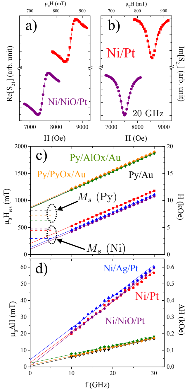
FIG. 5. FMR data for Ni- and Py-based samples. Example raw FMR response for Ni/Pt and Ni/NiO/Pt samples shown as a) real and b) imaginary parts of S_{21} at 20 GHz. The fits shown determine H_{\text{res}} and \Delta H for each f as shown in c) and d) for all samples. Lines in c) are fits to the out-of-plane Kittel Eq. (Eq. 3) and those in d) are linear fits (Eq. 4) to extract \alpha .
