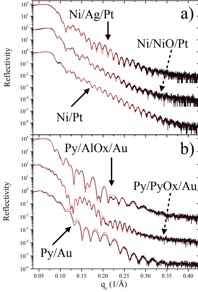
FIG. 1. X-ray reflectivity vs. q_z for a) Ni/Pt, Ni/NiO/Pt, Ni/Ag/Pt and b) Py/Au, Py/PyOx/Au, and Py/AlOx/Au samples. Black lines represent measured data with red lines the result of refinement to the model density profiles shown in Figs. 2 and 3. The top two plots in each panel are offset upward by a factor of 100 and 10,000.
