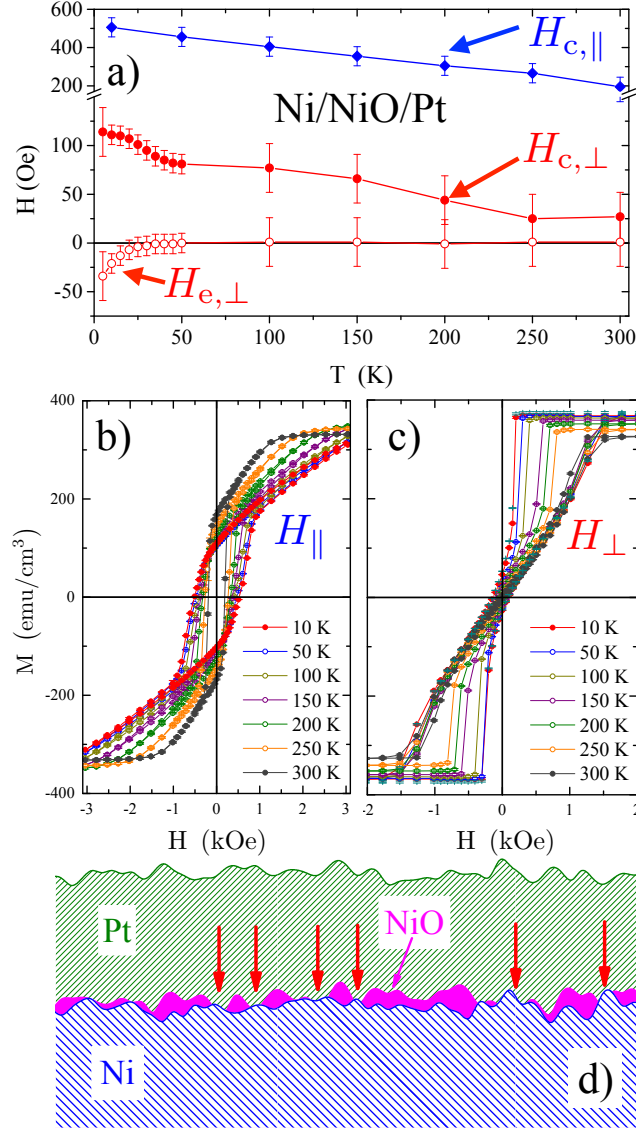
FIG. 8. Summary of evidence of perpendicular exchange bias in the Ni/NiO/Pt sample based on M measured after field cooling from 300 to 10 K under either in-plane or perpendicular external field bias of 3000 Oe. a) Coercive field for in-plane applied field ( H_{c,\parallel} ) and out-of-plane applied field ( H_{c,\perp} ) as well as perpendicular exchange bias field ( H_{e,\perp} ) vs. T . In-plane exchange bias was within error bars of H = 0 at all T and is not shown. b) M vs. H for in-plane applied field shown at various T . Larger field scans show a 10 K saturation near 5 kOe. c) M vs. H for out-of-plane applied field shown at various T . d) Schematic view of the interface based on GIXR results (Fig. 2) demonstrating the proposed mechanism for EB and enhanced coercivity. Note that we have not measured the lateral length scale of the roughness, and this schematic therefore only qualitatively represents the morphology of the surfaces. Red arrows indicate points of direct Ni/Pt contact.
