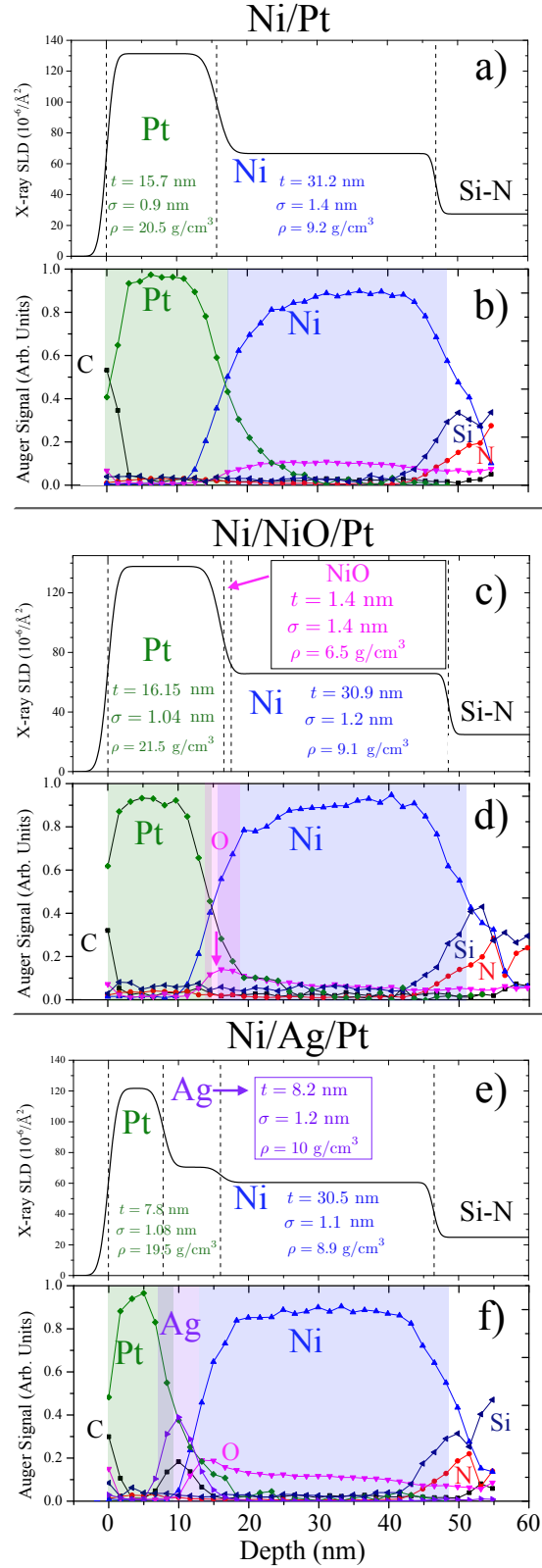
FIG. 2. Refined X-ray scattering-length density (SLD) and depth-profiled Auger electron spectroscopy for a-b) Ni/Pt, c-d) Ni/NiO/Pt, e-f) Ni/Ag/Pt heterostructures. Ni films left exposed to atmosphere for \sim 24 hours between FM and NM layer deposition show clear accumulation of O Auger electron signal localized to the interface. 9
