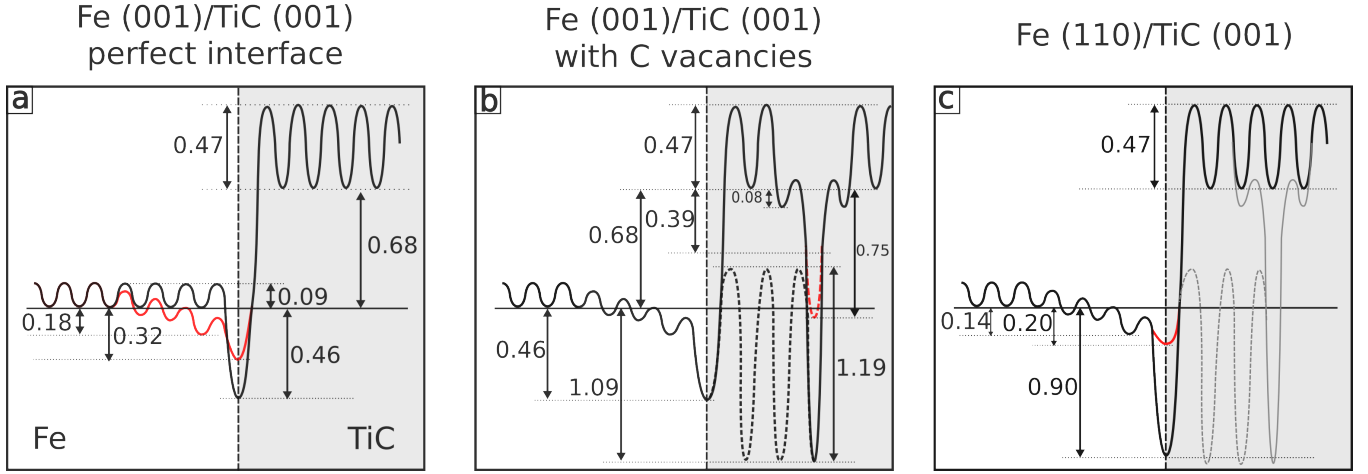
FIG. 11. (Color online) Energy profiles experienced by H atoms at: (a) the perfect coherent (001)_{\text{Fe}}/(001)_{\text{TiC}} interface (red curve) and the misfit dislocation core therein (black curve); (b) coherent (001)_{\text{Fe}}/(001)_{\text{TiC}} interface with single C vacancies at the interface and in the interior of the carbide (black curve), connected vacancies (dashed black curve), and single C vacancy in the interior of the carbide with double H occupancy (red dashed curve); (c) (110)_{\text{Fe}}/(001)_{\text{TiC}} interface with (black curve) and without (red curve) C vacancies at the interface, and with C vacancies in the interior of the carbide (grey line).
