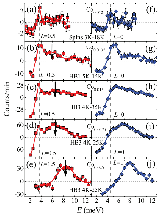
FIG. 2: (Color online) The neutron resonances in \text{NaFe}_{1-x}\text{Co}_x\text{As} as a function of increasing x , obtained as the difference of the energy-scans above and below T_c at the wave vectors \mathbf{Q}_{\text{AF}} = (1, 0, L) with L = 0.5, 1.5 (a-e) and Q = (1, 0, L) with L = 0, 1 (f-j). (a,f) x = 0.012 (UD); (b,g) x = 0.0135 (UD); (c,h) x = 0.015 (UD); (d,i) x = 0.0175 (UD); (e,j) x = 0.025 (OP). The plots are obtained directly by subtracting the superconducting state energy scan from those in the normal state without correcting for background, as is commonly done for determining the energy of the resonance 3-6 . The solid lines are fits with two Gaussians. The vertical dashed lines denote the low-energy resonance at E_{r1} in (a-d) and (f-i). The negative intensity below the resonance indicates the opening of a spin gap below T_c . The vertical arrows indicate the peak positions of the high-energy resonance E_{r2} at \mathbf{Q}_{\text{AF}} = (1, 0, L) with L = 0.5, 1.5 .
