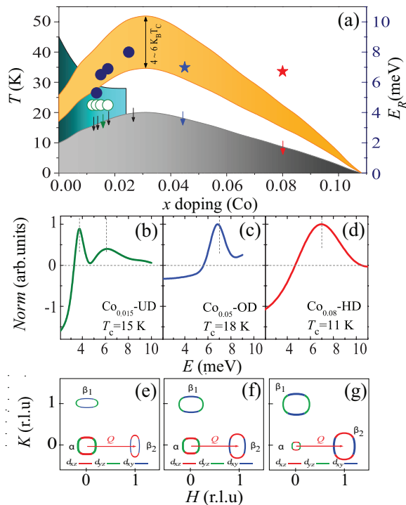
FIG. 1: (Color online) (a) The electronic phase diagram of \text{NaFe}_{1-x}\text{Co}_x\text{As} , where the arrow indicates the Co-doping levels studied in this work. The grey shaded area marks the Co-doping dependence of T_c . The region with AF order is represented by the green shaded area. The open circles are energies of the first resonance E_{r1} , and the filled circles and stars are energies of the second resonance E_{r2} . The yellow shaded area indicates approximate range of E_r \approx 4-6k_B T_c obtained from previous work 19,20 . (b-d) The schematic energy dependence of the resonance for three characteristic Co-doping levels, including underdoped (UD), optimally doped (OD), and highly overdoped (HD). (e-g) Schematic plots of the Fermi surfaces for the above three compositions. The color indicate different orbitals. The anisotropic superconducting gap \Delta_e on the electron pockets in the underdoped compounds become isotropic on the overdoped side 16 .
