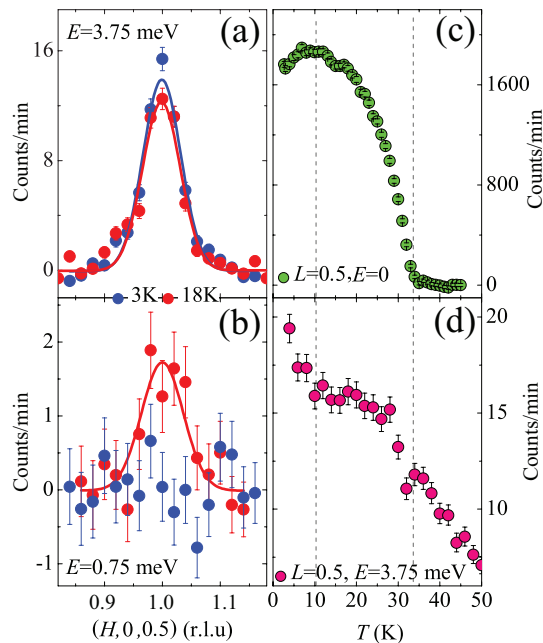
FIG. 3: (Color online) Wave vector and temperature dependence of the magnetic scattering for \text{NaFe}_{1-x}\text{Co}_x\text{As} with x = 0.012 when the system is near bulk superconductivity. The sample has T_N of \sim 35 K and T_c \approx 11 K. The data was collected on SPINS.
