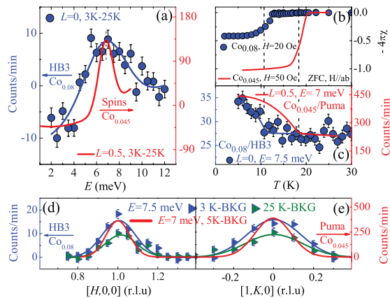
FIG. 5: (Color online) Comparison of the resonance in the overdoped regime at two compositions x = 0.045 and x = 0.08 . (a) The difference of the energy scans above and below T_c normalized by the corresponding peak intensities. The x = 0.045 and x = 0.08 compositions have similar peak energies around 7 meV, but have very different energy widths. For Co-doping levels above x = 0.025 , resonances are not dispersive along the L direction. (b) Temperature dependence of the susceptibility for x = 0.045 and x = 0.08 . The superconducting volume fraction of the x = 0.08 sample is about 40%. (c) Temperature dependence of the scattering intensity at the resonance energy, which show the onset of the resonance modes at their respective transition temperatures T_c . (d,e) The wave vector scans at the resonance energies along the [H, 0, 0] and [1, K, 0] directions below and above T_c for x = 0.08 . Similar data for x = 0.045 at 5 K is shown in red solid line 28 . The blue and green solid lines are Gaussian fits to the data.
