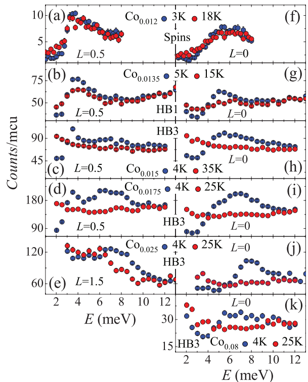
FIG. 4: (Color online) The raw data of energy scans at wave vectors \mathbf{Q}_{\text{AF}} = (1, 0, L) with L = 0.5, 1.5 (a-e) and L = 0 (f-k) obtained for \text{NaFe}_{1-x}\text{Co}_x\text{As} with different x above and below T_c .
