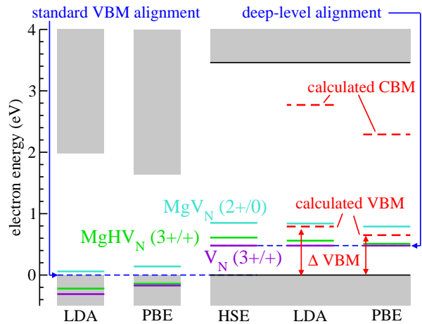
FIG. 1. (Color online). Alignment of the electron chemical potential scales between LDA, PBE, and HSE. For each of the functionals, the VBM defines the energy zero. Left: the standard alignment, using the calculated VBM as a common point of reference for all defects. Right: modified alignment, using the (3+/+) charge-state transition level for V_N (violet lines) as the common point of reference. The charge-state transition levels (2+/0) for MgV_N (cyan) and (3+/+) for MgHV_N (green) are also indicated, as well as the position of the calculated VBM and CBM of LDA and PBE.
