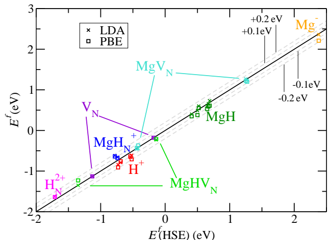
FIG. 4. (Color online). Comparison of the formation energies of LDA (crosses) and PBE (squares) with those of HSE, with corrections for the VBM and for the energies of the reference systems (see Table VII). Perfect agreement corresponds to the solid line. Dashed lines delimit deviations within the indicated bounds.
