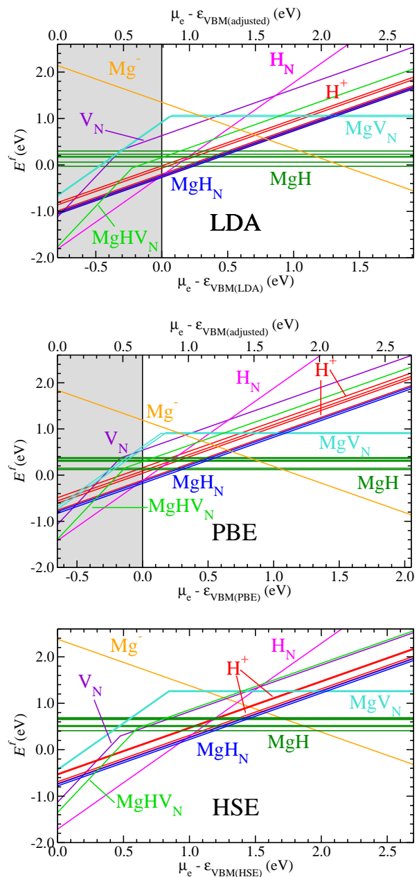
FIG. 3. (Color online). Defect formation energies as a function of electron chemical potential \mu_e = \varepsilon_{\text{VBM}} + \varepsilon_{\text{Fermi}} , calculated with LDA, PBE, and HSE. The bottom scale reflects the standard referencing scheme with respect to the calculated VBM at the respective level of theory. The top scale for LDA and PBE reflects the adjusted scale.
