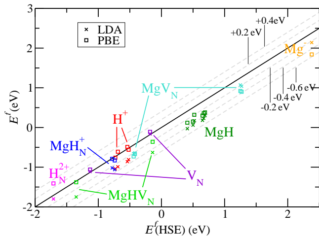
FIG. 2. (Color online). Comparison of the formation energies of LDA (crosses) and PBE (squares) with those of HSE, with corrections for the VBM (see Table VI). Perfect agreement corresponds to the solid line. Dashed lines delimit deviations within the indicated bounds.
