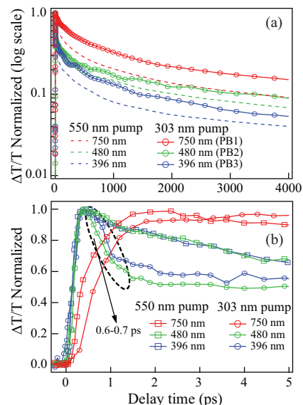
FIG. 2. Normalized kinetics at the PB peaks measured following excitation with different pumps (a) at longer time scales and (b) at shorter time scales. Panel (a) clearly illustrates the similarity of the decay of all three PB peaks independently of the pump, in agreement with the band-edge depopulation of photoexcited carriers.
