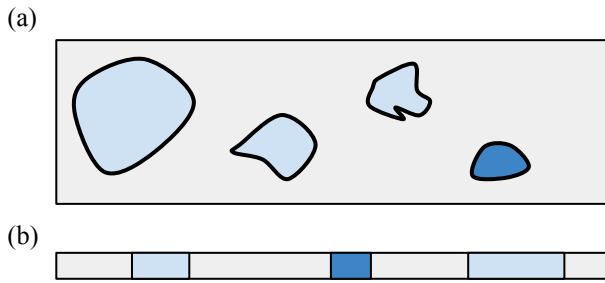
FIG. 1: Rare region effects in higher dimensions (a) vs. one dimension (b). In all cases, there are insulating inclusions with a wide distribution of sizes and local values of the control parameter (indicated here by shading). In higher dimensions, inclusions can be bypassed, and rare-region contributions are due to degrees of freedom inside the inclusions. In one dimension, inclusions act as bottlenecks, and thus affect dynamics even in typical regions.
