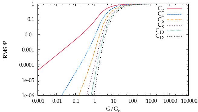
FIG. 3. Root-mean-square values of amplitudes defining excitation operators in the 12-site, half-filled pairing Hamiltonian with equally spaced levels using the configuration interaction parameterization of the wave function (Eq. 12). Results for larger systems are broadly similar.
