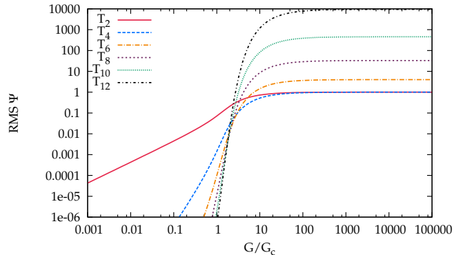
FIG. 2. Root-mean-square values of amplitudes defining excitation operators in the 12-site, half-filled pairing Hamiltonian with equally spaced levels using the coupled cluster parameterization of the wave function (Eq. 9). Results for larger systems are broadly similar.
