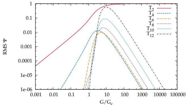
FIG. 4. Root-mean-square values of amplitudes defining excitation operators in the 12-site, half-filled pairing Hamiltonian with equally spaced levels using the Bessel parameterization of the wave function (Eq. 22). Compare to the coupled cluster and configuration interaction parameterizations in Figs. 2 and 3. Results for larger systems are broadly similar, although higher excitation amplitudes become fairly large before decaying to zero for large enough G/G_c .
