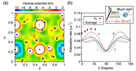
FIG. 3: (Color online) (a) Hartree potential map at z = 0.378 plane in pristine mayenite, where a free O atom is placed at the center of a cage (0, 0.25, 0.375) . The brown, gray, and blue dots represent the Ca, Al, and O atoms, respectively, within 0.25 \leq z \leq 0.5 . Potential minima for muon (shown by blue hatched area) are circularly spread around O. (b) Angle dependence of muon spin relaxation rate ( \delta_n ) under a transverse field of 20 mT. Dashed curves are simulated \delta_n for muons located at the position of 1~4, with their average represented by a solid curve. Inset: Schematic view of the relation between the magnetic field and sample rotation angle \theta from (001) surface.
