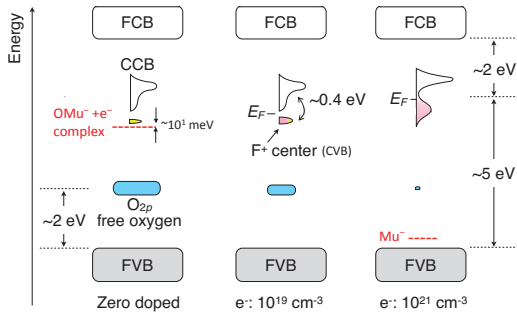
FIG. 4: (Color online) Schematic energy diagrams of mayenite 26–28 . The blue (pink) and yellow hatched regions show the occupied levels of oxygen (electron) in the cage center. The red dashed lines show the electronic levels associated with muon. FCB (FVB) and CCB (CVB) denote the frame conduction (valence) band and cage conduction (valence) band, respectively.
