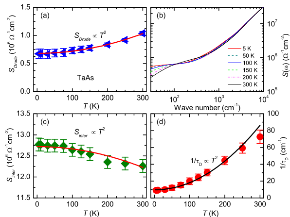
Figure 3. (color online) (a) Temperature dependence of the Drude weight. The solid line is a fit to a parabolic function. (b) Frequency-dependent spectral weight for several representative temperatures. (c) Evolution of the interband spectral weight with temperature. The solid line is a fit to a parabolic function. (d) shows the width of the Drude peak as a function of temperature. The solid line represents a T^2 behavior.
