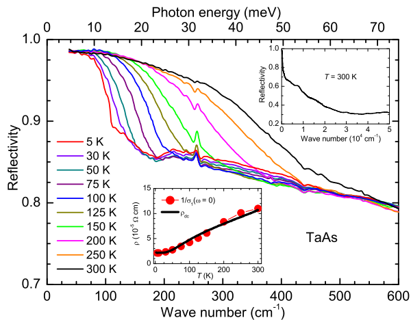
Figure 1. (color online) Far-infrared reflectivity for TaAs at different temperatures. Top inset: 300-K reflectivity over a broad frequency range. Bottom inset: Comparison of the DC resistivity, \rho (solid line), with the zero-frequency values of the Drude fits to the conductivity data (solid circles).
