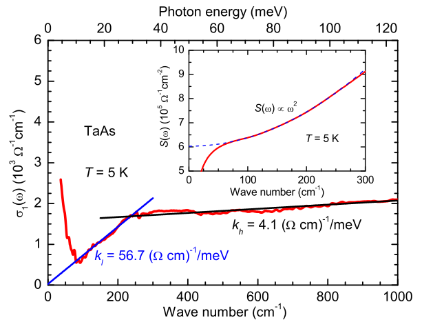
Figure 4. (color online) Optical conductivity for TaAs at 5 K. The blue and black solid lines through the data are linear guides to the eye. The inset shows the spectral weight as a function of frequency at 5 K (red solid curve), which follows an \omega^2 behavior (blue dashed line).
