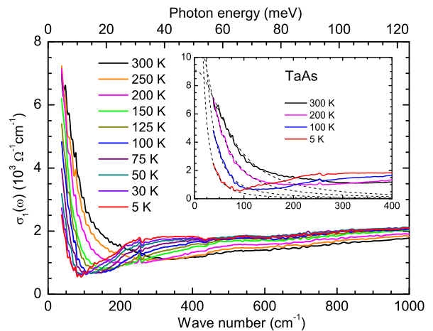
Figure 2. (color online) Temperature-dependent optical conductivity \sigma_1(\omega) in the far-infrared region for TaAs. Inset: Fits to the Drude model (dashed lines) at low frequencies for several representative temperatures.
