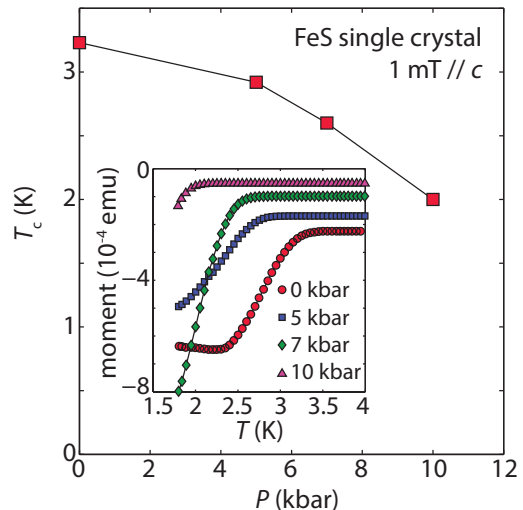
FIG. 9: Applied pressure dependence of the superconducting transition temperature of an \text{FeS} crystal as extracted from magnetic susceptibility measurements performed using a BeCu piston-cylinder clamp cell. Inset displays the measured susceptibility data (presented with a vertical offset for clarity). Pressure values are determined at room temperature.
