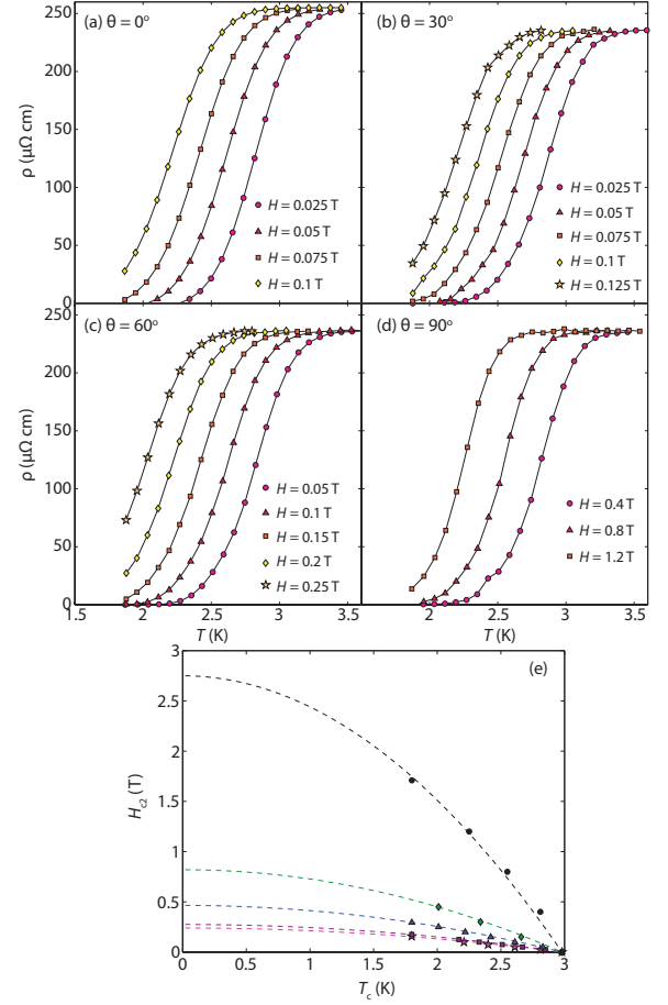
FIG. 7: Superconducting transition of FeS single crystal as a function of magnetic field applied along different angles \theta with respect to the crystallographic c -axis (transverse to current direction). Panel e) presents the compiled H_{c2}(\theta) temperature dependences for all angles measured. T_c values were determined by the resistance transition midpoint. Solid lines represent the WHH orbital pair-breaking expectation for H_{c2}(T) in each case (see text for details).
