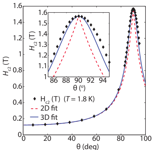
FIG. 8: Angular dependence of the superconducting upper critical field H_{c2} at 1.8 K. Black diamonds represented measured transition fields (defined as the resistive transition midpoint), and lines represent fits to the theoretical expectation for the angular dependence: solid line represents the Ginzburg Landau expectation for a 3D system with anisotropic effective mass, and dashed line represents the Tinkham's model expectation for 2D superconductors. Inset displays zoomed data near 90^\circ ( H \parallel ab ). All data were collected with magnetic field direction always transverse to the current direction.
