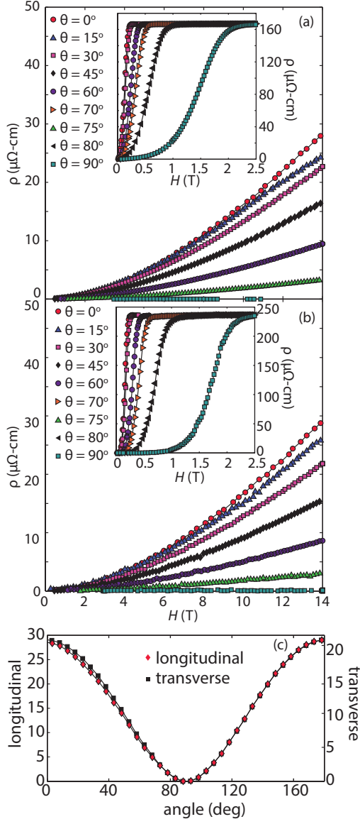
FIG. 6: Constant temperature scans of magnetoresistance (MR) of FeS as a function of field angle \theta , defined as the deflection from c -axis direction. Angular dependence of (a) longitudinal ( H(90^\circ) \parallel I ) and (b) transverse ( H(\theta) \perp I ) MR taken at 1.8 K are presented. Insets in each figure display a zoom of the superconducting H_{c2} transition. (c) Comparison of angular dependence of transverse and longitudinal MR at 1.8 K and 14 T.
