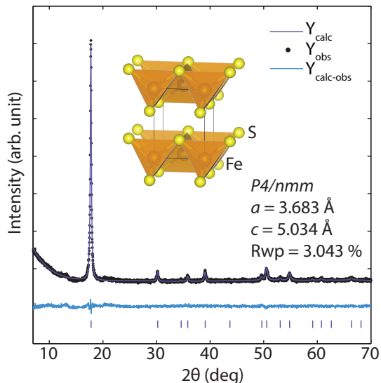
FIG. 1: Rietveld refinement with XRD powder diffraction on ground single crystal samples. (a) Refinement of K_x\text{Fe}_{2-y}\text{S}_2 template’s body-centered tetragonal structure ( I4/mmm ). (b) Refinement of the FeS product’s structure with a primitive tetragonal model ( P4/nmm ). Fe (orange) ions are tetrahedrally coordinated to S (yellow) anions, and the K (purple) cations are located between two FeS layers. Tick marks corresponding to their respective phase are shown below the difference curve.
