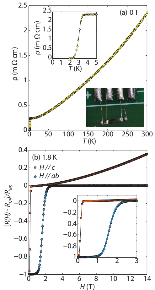
FIG. 5: Electrical resistivity of single crystalline FeS. (a) Temperature-dependent resistivity with inset highlighting low temperature transition to the superconducting state at T = 3.5 K. The geometry of the resistivity measurement for the single crystal also shown as inset. (b) Resistivity as a function of applied magnetic field for both H \parallel ab and H \parallel c orientations (always transverse to current direction).
