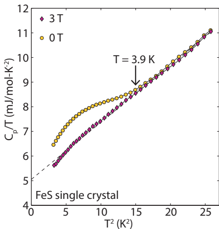
FIG. 4: Low temperature specific heat of single crystal FeS for 0 T and 3 T applied magnetic fields. The arrow indicates the onset of a superconducting feature at T = 3.9 K.
