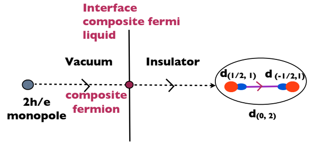
FIG. 7: Bulk-boundary correspondence for the composite fermi liquid. The composite fermion is the surface avatar of the electrically neutral strength-2 bulk monopole which itself is a bound state of the two (\pm\frac{1}{2}, 1) dyons. This strength-2 monopole is a fermion, and is Kramers-doublet under C . At the surface the two dyons that make up this monopole correspond to the two ends of the dipole of Fig. 2.
