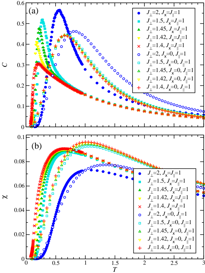
FIG. 12. (Color online) Comparison between the specific heat, C (a), and susceptibility, \chi (b), of a fully frustrated ladder ( J_{\parallel} = J_x = 1 , closed symbols and crosses) and an unfrustrated ladder ( J_{\parallel} = 1 , J_x = 0 , open and plus symbols) for a range of values of J_{\perp}/J_{\parallel} . Shown are QMC results for ladders of L = 100 rungs. Error bars on the unfrustrated ladder data are much smaller than the symbol sizes and are omitted.
