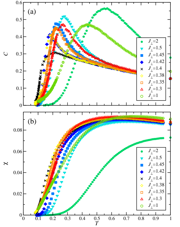
FIG. 11. (Color online) QMC results for the specific heat, C (a), and susceptibility, \chi (b), of the fully frustrated ladder ( J_x = J_{\parallel} = 1 ) for a range of values of J_{\perp}/J_{\parallel} .
