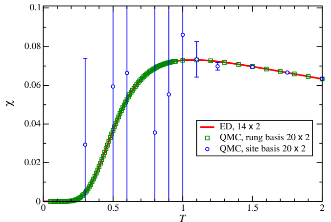
FIG. 7. (Color online) Comparison of the magnetic susceptibility, \chi , obtained for a fully frustrated ladder with J_{\perp} = 2 and J_{\parallel} = J_{\times} = 1 , between QMC results for a system of L = 20 rungs and ED results for L = 14 . QMC simulations were performed in both the single-site basis and the rung basis.
