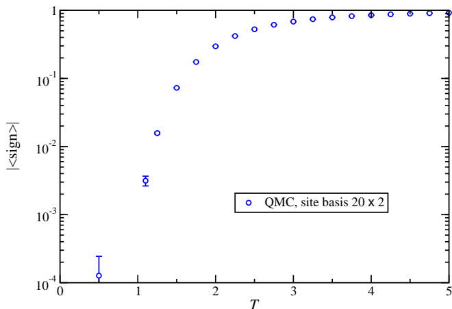
FIG. 8. (Color online) Average sign obtained during QMC simulations in the single-site basis of the L = 20 ladder with J_{\perp} = 2 and J_{\times} = J_{\parallel} = 1 .
