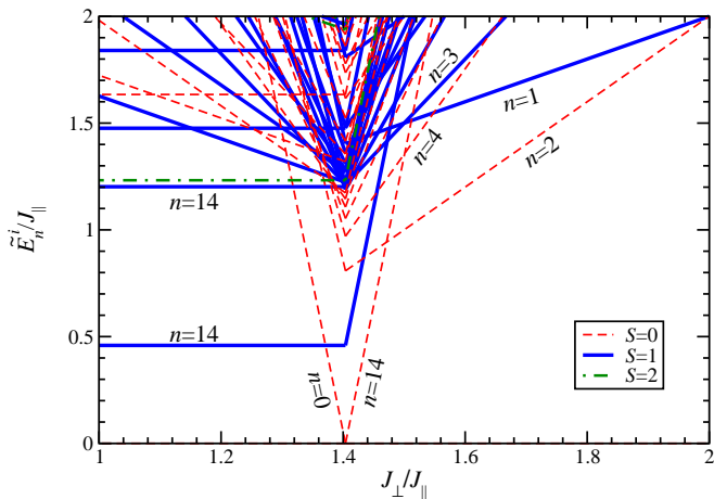
FIG. 2. (Color online) Low-energy excited levels, \tilde{E}_n^i , of a 14-rung fully frustrated spin-1/2 ladder, shown as a function of J_\perp/J_\parallel . All excitations are classified according to their total spin quantum number, S , and some by an additional label for the number, n , of consecutive rungs in the triplet state.
