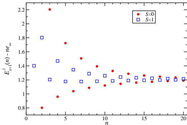
FIG. 3. (Color online) Energies of the two lowest states of an open, n -site, spin-1 Heisenberg chain relative to that of an n -site segment of an infinite chain, shown as a function of n and in units of J_{\parallel} . Red circles denote total singlets ( S = 0 ) and open blue squares total triplets ( S = 1 ).
