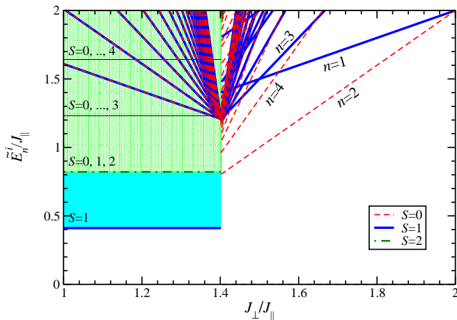
FIG. 4. (Color online) Schematic overview of the low-energy excitations, \tilde{E}_n^i , of the infinite, fully frustrated spin-1/2 ladder, shown as a function of J_{\perp}/J_{\parallel} for a broad region around the quantum phase transition at J_{\perp,c} = 1.410484 J_{\parallel} . Excitations are classified according to their total spin quantum number, S . The additional label n for the rung-singlet phase specifies the origin of excitations in the bound states of n -rung triplets. Shaded regions in the rung-triplet phase denote single- and multiple-magnon continua.
