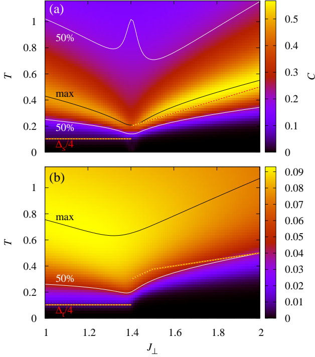
FIG. 10. (Color online) Exact diagonalization results for the specific heat, C (a), and susceptibility, \chi (b), of the fully frustrated ladder ( J_x = J_{\parallel} = 1 ) with L = 14 rungs, shown for the full range of J_{\perp}/J_{\parallel} ratios around the transition. Black lines mark the positions, T_{\max}^C and T_{\max}^{\chi} , of the peaks in both quantities. White lines mark the temperatures, T_{\text{half}}^C and T_{\text{half}}^{\chi} , where they have reached half of the peak height, and for C(T) the temperature, T_u^C , where the peak has fallen again to half of the peak height as T continues to increase. Red-yellow dashed lines mark 1/4 of the gaps relevant for each quantity, which for C(T) is the minimum gap \Delta_s and for \chi(T) the triplet gap \Delta_t (Subsec. II A).
