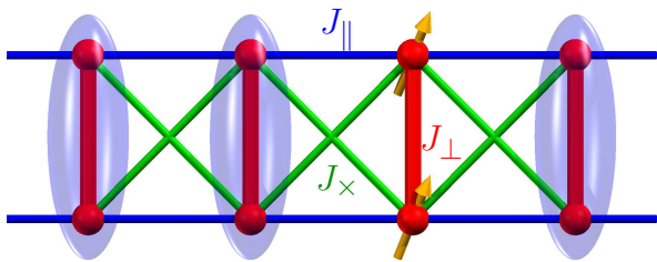
FIG. 1. (Color online) Representation of superexchange interactions in a frustrated spin ladder. Each ladder site (spheres) hosts an S = 1/2 quantum spin and the Heisenberg couplings between spins are specified by the parameters J_{\perp} for the ladder rungs, J_{\parallel} for the ladder legs, and J_{\times} for the cross-plaquette couplings, which we take to be symmetrical. Ellipsoids represent singlet states of the two rung spins and their absence a rung triplet.
