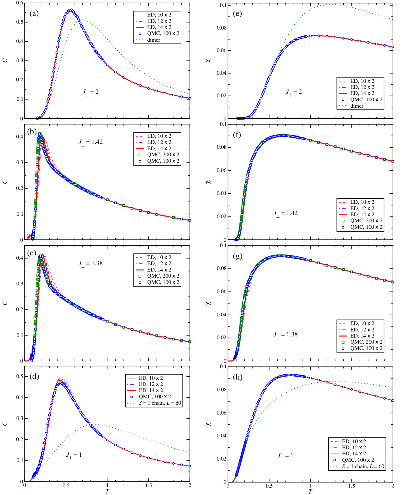
FIG. 9. (Color online) Specific heat, C (left column), and susceptibility, \chi (right column), per spin for fully frustrated ladders with inter-rung couplings J_x = J_{||} = 1 and rung couplings J_{\perp} = 2, 1.42, 1.38, and 1 (from top to bottom). Each panel compares ED results for system sizes of L = 10, 12, and 14 rungs with QMC results obtained for L = 100 rungs. In panels (a) and (e) we include the results (9) and (10) for isolated dimers of rung coupling J_{\perp} = 2 J_{||} . In panels (d) and (h) we include QMC results for a spin-1 chain of L = 60 sites [45], normalized to twice the number of spins in the chain.
