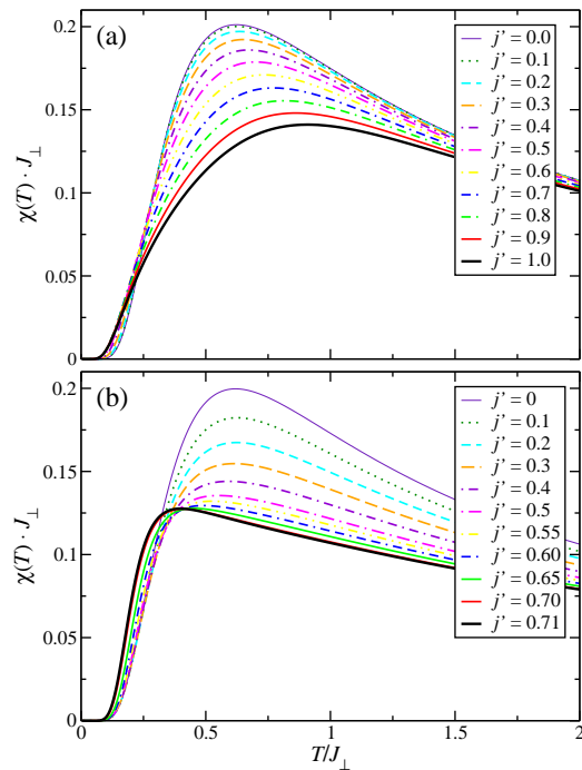
FIG. 6. (Color online) Magnetic susceptibility of (a) the unfrustrated ladder and (b) the four-rung approximation to the fully frustrated ladder, shown as functions of temperature for a range of values of the inter-rung coupling, j' = J_{\parallel}/J_{\perp} .
