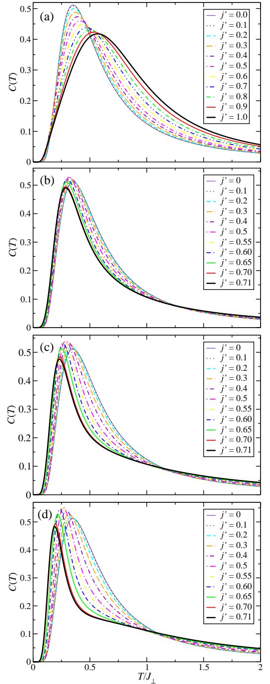
FIG. 5. (Color online) Magnetic specific heat of (a) the unfrustrated ladder, (b) two, (c) three, and (d) four fully frustrated rungs, shown as functions of temperature for a range of values of the inter-rung coupling, j' = J_{\parallel}/J_{\perp} .
