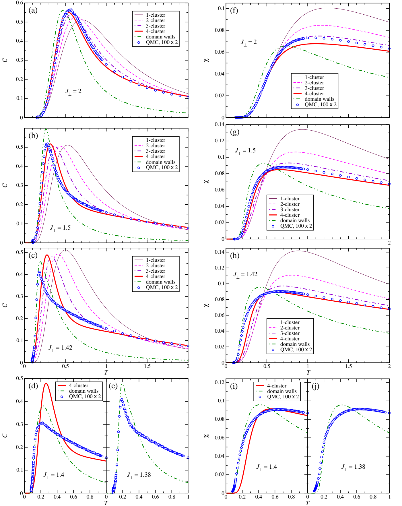
FIG. 13. (Color online) Specific heat, C (left column), and susceptibility, \chi (right column), of fully frustrated ladders ( J_{\times} = J_{\parallel} = 1 ) with rung coupling ratios J_{\perp}/J_{\parallel} = 2, 1.5, 1.42, 1.40, and 1.38 . QMC results for ladders of L = 100 rungs are compared with approximate calculations based on clusters of 2, 3, and 4 rungs (Subsec. II B) and on non-interacting domain walls (Subsec. V B).
