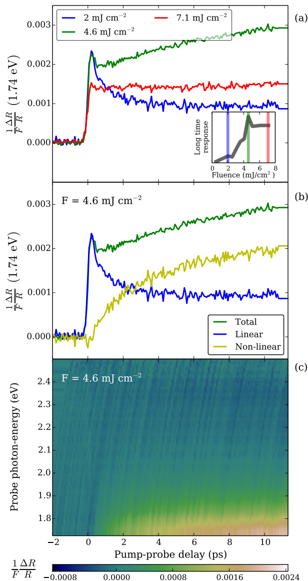
FIG. 8. (a) \frac{1}{F} \frac{\Delta R}{R}(t) at 1.74 eV for 2.0 \text{mJ cm}^{-2} (blue), 4.6 \text{mJ cm}^{-2} (green), 7.1 \text{mJ cm}^{-2} (red) pump fluences. Inset: visual reference to figure 7. (b) Green: as in (a). Blue (yellow): linear (non-linear) term of \frac{1}{F} \frac{\Delta R}{R} for F = 4.6 \text{ mJ cm}^{-2} at 1.74 eV photon-energy. (c) \frac{1}{F} \frac{\Delta R}{R}'(h\nu, t) for F = 4.6 \text{ mJ cm}^{-2} .
