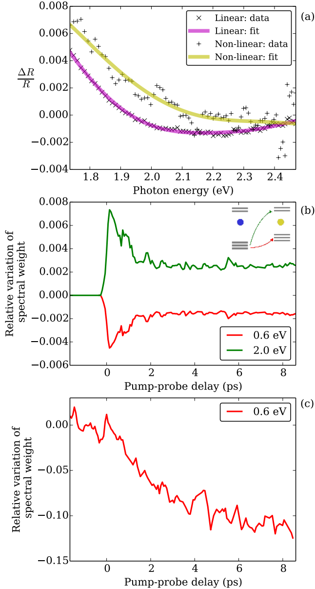
FIG. 10. (a) Linear and non-linear terms in \frac{\Delta R}{R} at 0.2 ps and 8.0 ps respectively, and their fits. (b) Variation of the spectral weight as a function of pump-probe delay of the 0.6 (red) and 2.0 (green) oscillators as resulting from the fit of the linear/low-fluence \frac{\Delta R}{R} . Inset: sketch of the involved transitions. (c) Variation of the spectral weight of the 0.6 eV oscillator from the fit of the non-linear term of \frac{\Delta R}{R} .
