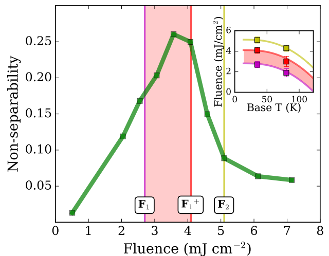
FIG. 9. Ratio of the second largest and largest singular values (from both, the noise level was subtracted), as a function of fluence. Inset: same inset as in figure 7, with the addition of the fluences at which the “non-separability” starts to decrease (red squares), as measured at 35 and 80 K. These match the calculated equivalent fluences needed to deliver the full latent heat to the sample (red line).
