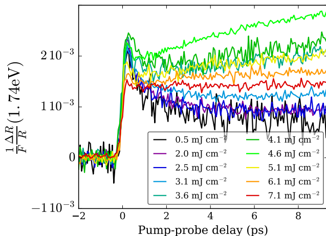
FIG. 6. Normalized relative variation of the reflectivity \frac{1}{F} \frac{\Delta R}{R}(h\nu = 1.74 \text{ eV}, t) at 35 K for all the available pump fluences.
