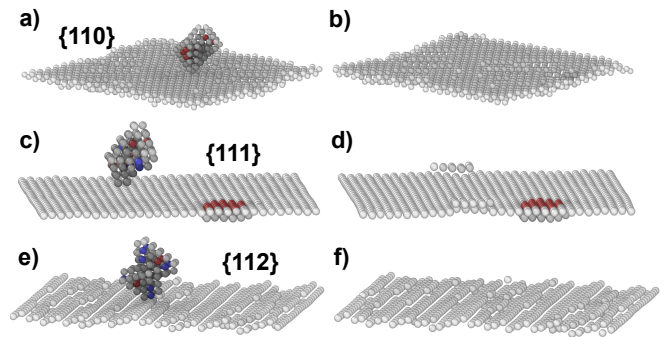
FIG. 1: (Color online) 12V-SFT interacting with (a) and (b) a {110}; (c) and (d) a {111}; and (e) and (f) a {112} free surfaces in single phase Cu. Atoms are colored according to their structure (as determined by a common neighbor analysis), hcp as red, bcc as blue and unknown structure as white; fcc atoms are not shown for clarity. In (a), (c), and (e), the configuration as the SFT first directly interacts with the surface is provided, while the configuration after full absorption of the SFT by each surface is provided in (b), (d) and (f). The perspective is from inside the material, viewing the surface from within.
