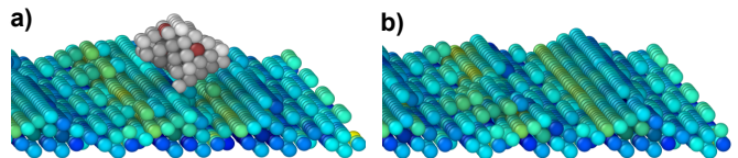
FIG. 10: (Color online) 12V-SFT interaction with an ARB KS hetero-interface in Cu-Nb. (a) shows the initial interaction and (b) illustrates the final interface configuration after the SFT has been absorbed. The color coding is the same as in Fig. 4.
