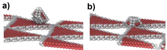
FIG. 6: (Color online) Interaction of a 12V-SFT with a 2^\circ \{111\} twist boundary in Cu. (a) Initial interaction; (b) Final configuration. The color coding is the same as in Fig. 1.
