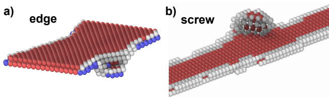
FIG. 2: (Color online) Resulting configuration after the interaction of a 12V-SFT with (a) an edge dislocation and (b) a screw dislocation in single phase Cu. Dislocations are split into Shockley partials bounding a stacking fault ribbon. The color coding is the same as in Fig. 1.
