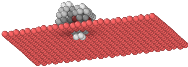
FIG. 8: (Color online) 12V-SFT interacting with a \Sigma 3 twin boundary in Cu. The color coding is the same as in Fig. 1.
