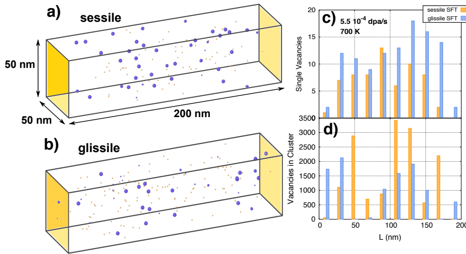
FIG. 12: (Color online) Single vacancies (brown) and vacancy clusters (blue) found from OKMC simulations considering vacancy clusters (SFTs) as (a) sessile or (b) glissile (b) at 700 K and a dose rate of 5.5 \times 10^{-4} dpa/s after 1 s. (c) shows the distribution of single vacancies and (d) the distribution of vacancies in clusters for both cases. L denotes the dimension perpendicular to the interfaces.
