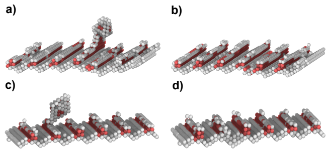
FIG. 3: (Color online) (a)-(b) 12V-SFT and (c)-(d) 18V-SFT interacting with an asymmetric \Sigma 11 tilt grain boundary in Cu. (a) and (c) show the initial interaction of the SFT with the boundary while (b) and (d) display the final configuration, after the SFT has been absorbed by the boundary. The color coding is the same as in Fig. 1.
