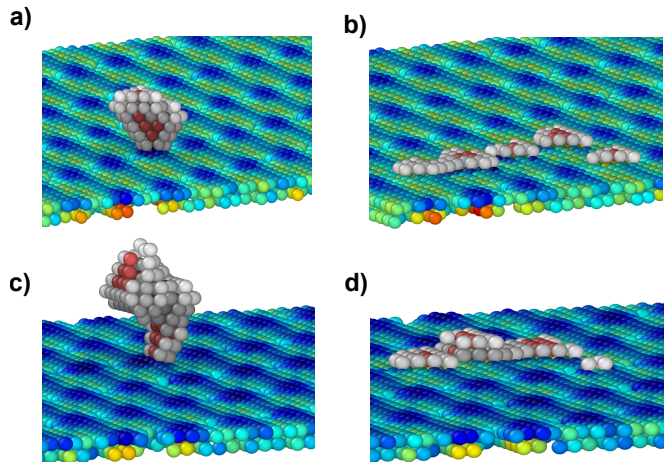
FIG. 9: (Color online) (a)-(b) Interaction of a 12V-SFT with a KS1 hetero-interface in Cu-Nb. (a) shows the first reaction and (b) the final interface configuration. (c)-(d) Interaction of a 18V-SFT with a KS1 hetero-interface: (c) shows the first reaction and (d) the final configuration. The color coding is the same as in Fig. 4. The dark blue regions correspond to the locations of the MDIs within the interface. In this perspective, the view is from inside Cu, looking down on the interfacial plane.
