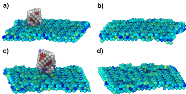
FIG. 4: (Color online) (a)-(b) 12V-SFT and (c)-(d) 18V-SFT interacting with a \Sigma 5 twist grain boundary in Cu. (a) and (c) show the initial interaction while (b) and (d) display the final configuration after absorption. The interface is colored according to \sigma_{xx} on each atom calculated with the virial theorem while the SFT is colored according to the atomic structure (hcp and unknown coordination as red and white, respectively).
