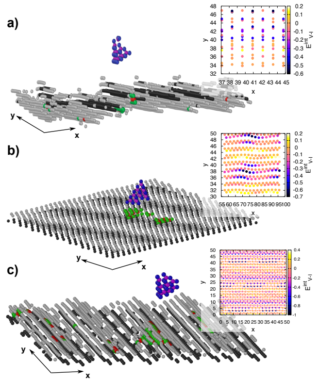
FIG. 11: (Color online) Analysis of the atomic displacement before and after the interaction of a 12V-SFT with the (a) asymmetric \Sigma 11 tilt, (b) CuNb KS1, and (c) ARB KS interfaces. Blue particles represent vacancies while purple describes "interstitial-like" particles before the interaction. Green particles represent vacancies and red "interstitial-like" particles after the interaction. These are identified via a lattice-reference method in which the structure is compared before and after the reaction. In (a) gray atoms belong to unknown structure and black to hcp. In (b) and (c) gray and black atoms are Cu and Nb, respectively, belonging to the interface. The maps in the insets show the vacancy-interface interaction energy with the pristine interface.
