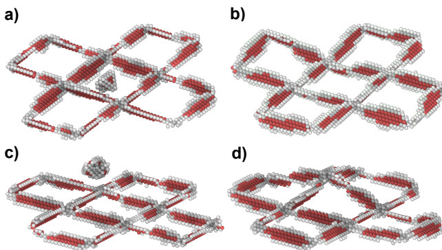
FIG. 5: (Color online) (a)-(b) 12V-SFT and (c)-(d) 18V-SFT interacting with a 4^\circ \{100\} twist boundary in Cu. (a) and (c) show the initial interaction of the SFT with the boundary while (b) and (d) show the final configuration after absorption. The color coding is the same as in Fig. 1.
