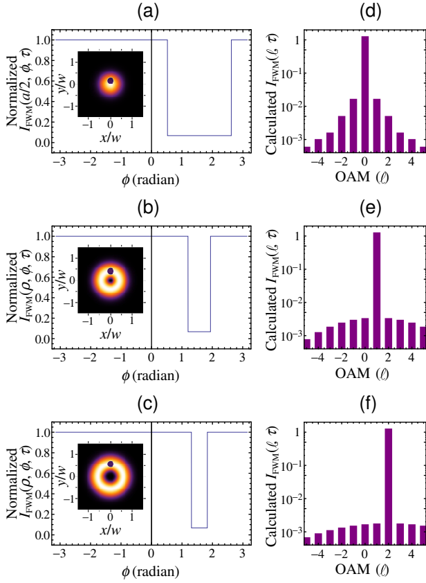
FIG. 6. (a)-(c) The calculated four-wave mixing (FWM) signals and their angular distributions at delay time \tau > 0 for l_x = 0, 1 , and 2 including the effects of the spatially dependent dephasing. In the calculation, we use \tau = 1/\gamma_0 and the exciton dephasing rate in the defect \gamma(r_0, \phi_0) = 2\gamma_0 , where \gamma_0 represents the exciton dephasing rate on the defect-free region. At \tau > 0 , the signal intensity rapidly decays in the point-like defect located at (r, \phi) = (\rho, \pi/2) except for the case of l_x = 0 . When l_x = 0 , the defect is slightly shifted from the beam center by a/2 . In the calculation, \gamma_0 = 1 and a = 0.3w are used. (d)-(f) The OAM spectra calculated for the FWM signals shown in (a)-(c) with the use of Eq. (8). In the figures, we use a logarithmic vertical scale and the OAM-resolved intensity is normalized so that the maxima are equal to unity.
