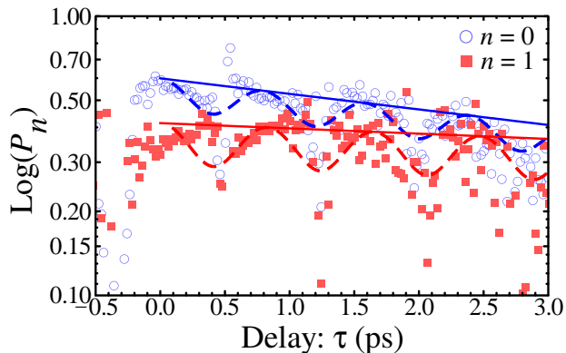
FIG. 5. The time evolutions of P_0 and P_1 (with a logarithmic vertical scale). The dashed curves indicate the sinusoidal exponential decays obtained by our fitting 36 . The solid lines are the exponential decays \exp(-2\tau/T_{\text{OAM}}) extracted from the fitting curves and shown to highlight the difference of the decay times T_{\text{OAM}} between P_0 ( 15.6 \pm 0.1 ps) and P_1 ( 46 \pm 2 ps).
