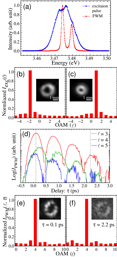
FIG. 2. (a) The spectrum of the four-wave mixing (FWM) signal. For reference, the spectrum of the excitation pulse is also overlaid. (b) The orbital angular momentum (OAM) spectrum of the pump pulse and (c) that of the probe pulse. For each spectrum, the vertical axis is normalized by its peak intensity. The insets show the intensity profiles of the corresponding beams. (d) The time evolutions of the OAM-resolved FWM signal (with a logarithmic vertical scale). In the figure, the \ell = 3 , \ell = 4 , and \ell = 5 components of the signal are plotted. (e), (f) The OAM spectra of the FWM signal at the selected delay time \tau (the first and fourth QB peaks indicated by the dashed vertical lines in (c)). The intensity profiles of the FWM signal are also shown in the insets.
