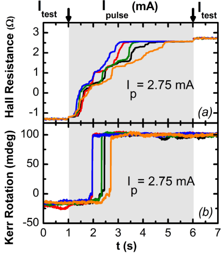
Figure 3. Hall resistance (a) between the contact pads shown in Fig.1.(d) as the device undergoes 5 switching events under identical conditions induced by 5.0 s duration current pulses, with amplitude I_p = 2.75 mA, triggered at t = 1.0 s (darker background on graph). The Hall resistance is measured before ( t = 0.0 - 1.0 s) and after ( t = 6.0 - 7.0 s) the pulse using a current of 0.1 mA. (b) shows the simultaneous measurement of the Kerr rotation within a sub micron region mid-way between the Hall contacts, also shown Fig.1.(d).
