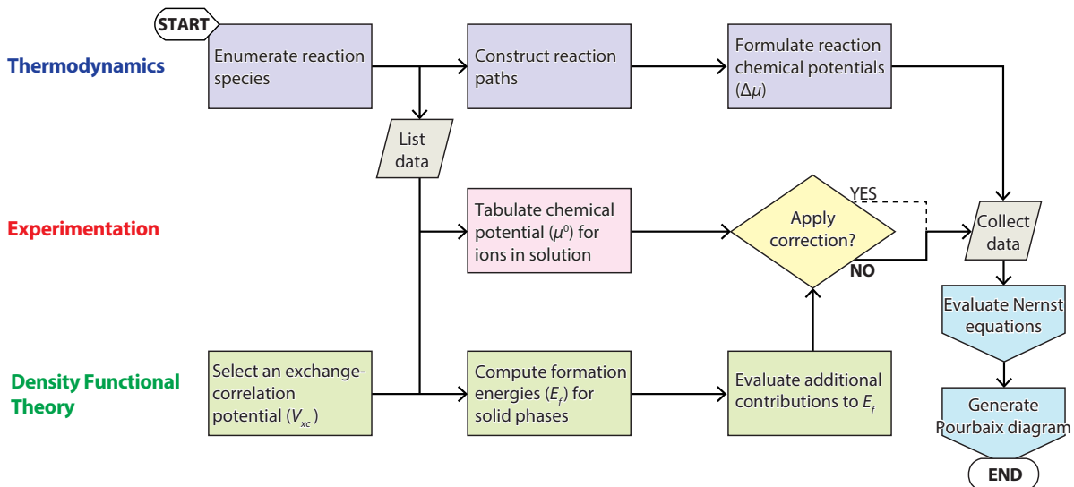
FIG. 2. Workflow diagram for accurate (correction free) simulation of electrochemical Pourbaix diagrams from density functional theory. The process involves inputs from thermodynamic formula, experimental data, and accurate density functional theory. The path taken in this work follows the bolded arrows and further details for what occurs at each step are given in the main text. Of note, we point out that a variety of corrections can be made to improve the agreement between density functional theory values and experiment; however, we avoid these ad hoc (and often tedious) corrections by using more accurate functionals that include additional forms of electronic exchange. In the outcome step involving the Nernst equations, the chemical potential is computed with collected theoretical and experimental data for each species with respect to pH and electrode potential; the molar concentration of the aqueous ions in solution is also specified. In the final step, the lowest energy species per pH value and electrode potential is obtained on a dense grid to generate the resulting Pourbaix diagrams that appear throughout the text.
