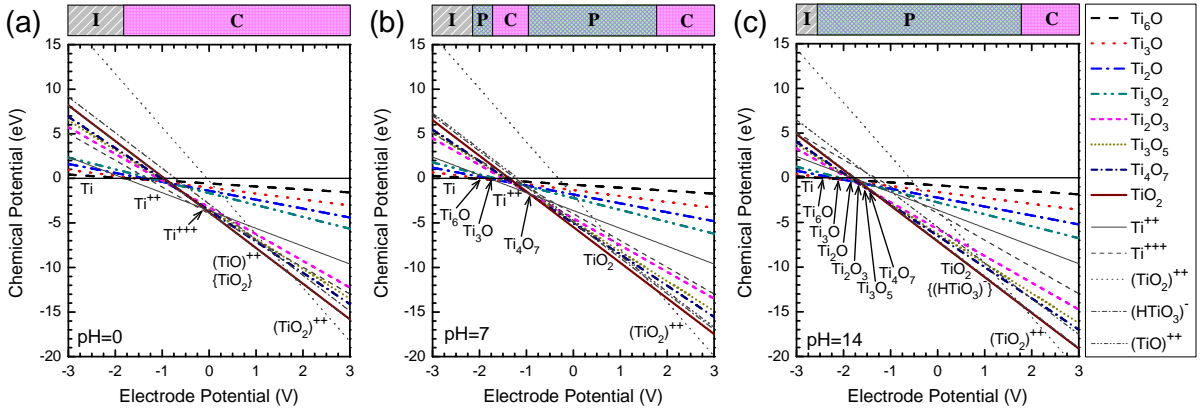
FIG. 6. Variation of chemical potentials ( \mu ) with electrode potential at different pH values (0, 7, and 14) calculated from the HSE06+vib method, where \mu(\text{Ti}) is the reference. The species with the lowest \mu are labeled, and in panel (a) and (c), \text{TiO}_2 and (\text{HTiO}_3)^- ion (in braces) are very close to the lowest \text{TiO}^{++} and (\text{TiO}_2)^{++} ions, respectively. The immunity (I), passivation (P), and corrosion (C) domains are indicated on the panel top.
