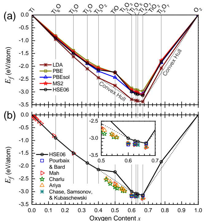
FIG. 3. (a) Calculated formation energies ( E_f ) of Ti oxides with respect to various exchange-correlation potentials. (b) The comparison between HSE06 and experimental results. 15,27,64,69 The inset in panel (b) shows in detail the range x \in (0.5, 0.7) .
