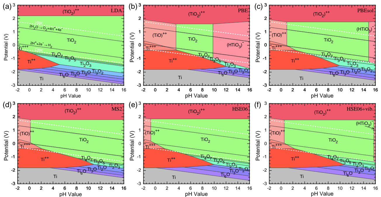
FIG. 5. Pourbaix diagrams calculated using (a) LDA, (b) PBE, (c) PBEsol, (d) MS2, and (e) HSE06 functionals, as well as (f) HSE06 functional plus vibrational (vib) contributions. The CBM and VBM levels of rutile \text{TiO}_2 , and the electrode potentials for the oxidation of \text{H}_2\text{O} to \text{O}_2 ( 2\text{H}_2\text{O} \rightarrow \text{O}_2 + 4\text{H}^+ + 4e^- ) and for the reduction of \text{H}^+ to \text{H}_2 ( 2\text{H}^+ + 2e^- \rightarrow \text{H}_2 ) are obtained from Ref. 74.
