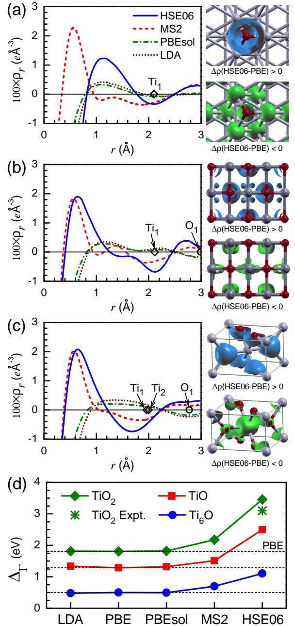
FIG. 4. Functional-dependent radial electron density ( \rho_r ) around an O atom (reference: PBE \rho_r ) and the electron density difference \Delta\rho(\text{HSE06-PBE}) (isovalue: \pm 0.01 e\text{\AA}^{-3} ) in (a) \text{Ti}_6\text{O} , (b) \text{TiO} , and (c) \text{TiO}_2 , where the locations of the Ti and O neighbors for an O atom located at the origin (0 \text{\AA} ) are indicated by hollow diamonds and circles, respectively. (d) The functional-dependent \Gamma -point band gap ( \Delta_\Gamma ) in \text{Ti}_6\text{O} , \text{TiO} , and \text{TiO}_2 , where the PBE gaps are indicated by dashed horizontal lines, and the experimental \Delta_\Gamma for rutile \text{TiO}_2 11,14,69,72 is indicated by the star.
