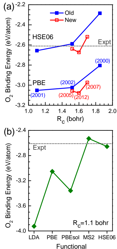
FIG. 1. The dependence of the \text{O}_2 binding energy on the type of (a) pseudopotential and (b) density functional at R_c = 1.1 bohr, where R_c is the ion radius in the PAW pseudopotential. The zero-point energy correction ( -0.049 eV) has been used in the experimental value ( -2.611 eV). In panel (a), the generation years of the pseudopotentials provided by VASP are indicated in parentheses.
