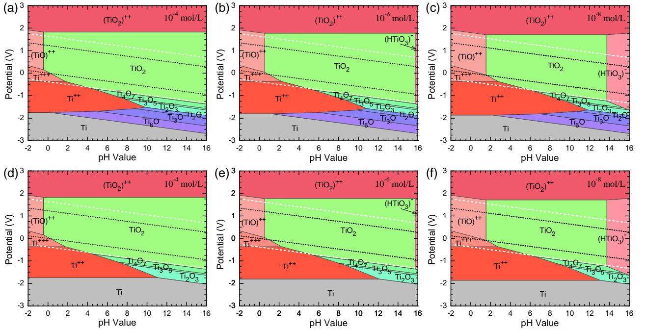
FIG. 7. Pourbaix diagrams with aqueous ion concentrations of (a, d) 10^{-4} , (b, e) 10^{-6} , and (c, f) 10^{-8} mol/L, obtained with the HSE06+vib method. The interstitial oxides are excluded in panels (d) through (e).
