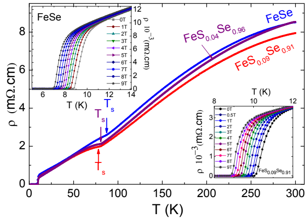
FIG. 1. (Color online) Temperature dependence of the in-plane resistivity of FeSe (blue curve) and \text{FeSe}_{1-x}\text{S}_x single crystals with x = 0.04 (purple curve) and x = 0.09 (red curve). The arrows indicate the temperature T_s at which the tetragonal-to-orthorhombic structural transition occurs. The two insets show the evolution of the superconducting transition in magnetic fields, up to 9 T, applied along the c -axis.
