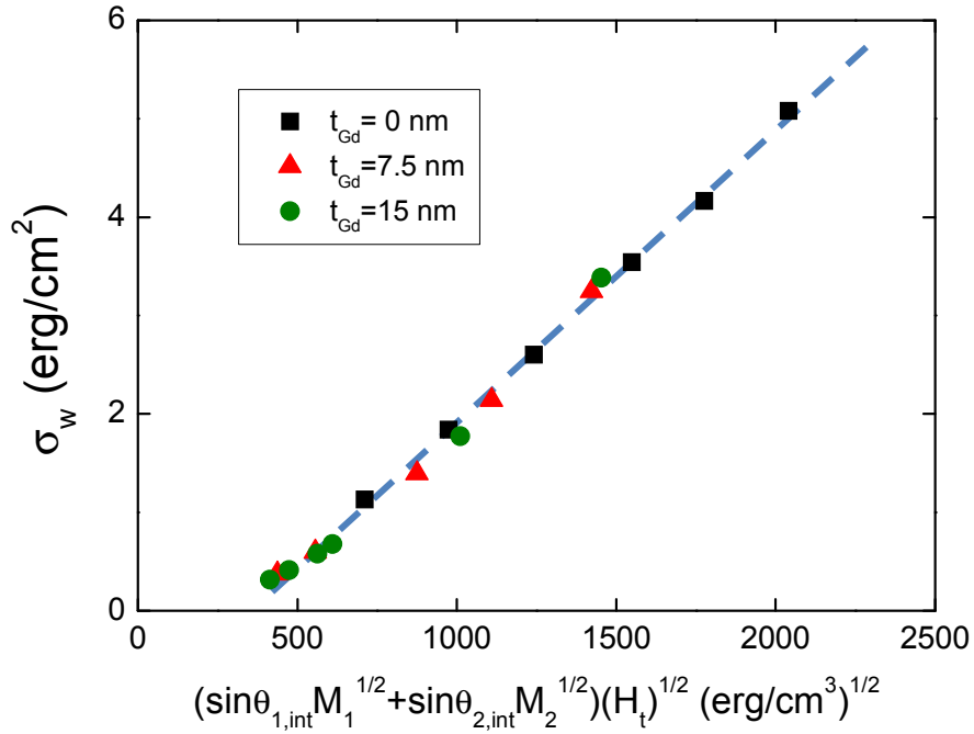
Figure 8. (color online) iDW energy calculated as \sigma_w = 2H_t M_2 t_2 from MOTKE loops in comparison with analytical model eq. (5); different \theta_{i,\text{int}} values are used for each sample, in order to obtain the scaling of the experimental data to a single line: \sin\theta_{1,\text{int}} = \sin\theta_{2,\text{int}} = 1 in \text{Gd}_{11}\text{Co}_{89}/\text{Gd}_{35}\text{Co}_{65} bilayer and \sin\theta_{1,\text{int}} = 0.8 , \sin\theta_{2,\text{int}} = 1 in \text{Gd}_{11}\text{Co}_{89}/\text{Gd}/\text{Gd}_{35}\text{Co}_{65} trilayers. Dashed line is a linear fit of \sigma_w vs. (H_t)^{1/2}[\sin(\theta_{1,\text{int}})M_1^{1/2} + \sin(\theta_{2,\text{int}})M_2^{1/2}] according to eq. (5). Its slope corresponds to exchange stiffness A_{\text{GdCo}} = 1.05 \times 10^{-6} erg/cm.
