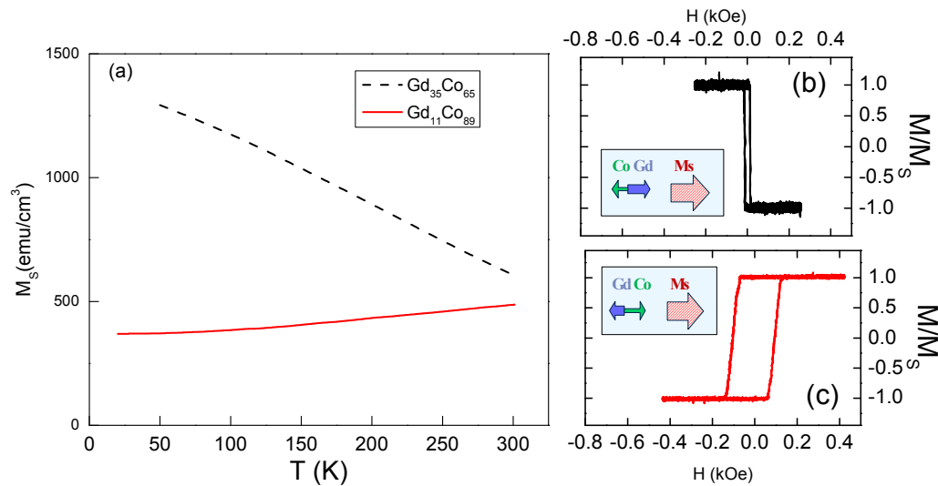
Figure 2. (color online) (a) Temperature dependence of the saturation magnetization of 50 nm thick Gd-Co single films with different compositions; MOTKE hysteresis loops for (b) \text{Gd}_{35}\text{Co}_{65} and (c) \text{Gd}_{11}\text{Co}_{89} at 50 K. Note that at this wavelength the magneto-optical signal comes exclusively from the Co sublattice: the inverted loop observed for \text{Gd}_{35}\text{Co}_{65} corresponds to an alloy with net magnetization dominated by the Gd sublattice whereas the direct loop observed for \text{Gd}_{11}\text{Co}_{89} corresponds to an alloy with magnetization dominated by the Co sublattice (see sketches in the insets).
