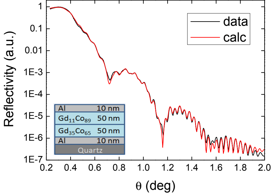
Figure 3. (color online) Resonant small angle X-ray reflectivity measured in a longitudinal geometry at E = 7245 eV (Gd L3 edge) for a 50 nm Gd_{35}Co_{65}/50 nm Gd_{11}Co_{89} bilayer. Red lines are structural fits with PPM code.
