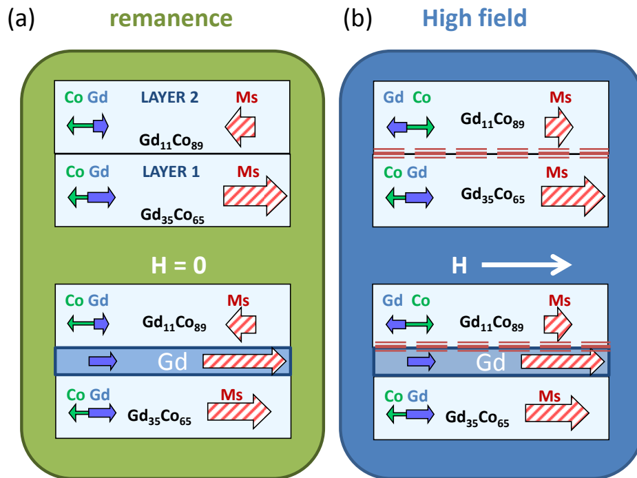
Figure 1: (color online) Sketch of the magnetic configuration of Gd-Co/Gd-Co' bilayers and Gd-Co/Gd/Gd-Co' trilayers at remanence (a) and at a high field (b). Dashed line indicates iDW at high field.
