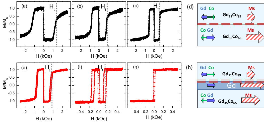
Figure 4. (color online) MOTKE hysteresis loops of top Gd 11 Co 89 layer (Layer 2) for a 50 nm Gd 11 Co 89 /50 nm Gd 35 Co 65 bilayer at (a) 50 K; (b) 150 K; (c) 200 K and for a 50 nm Gd 11 Co 89 /7.5 nm Gd/50 nm Gd 35 Co 65 trilayer at (e) 50 K; (f) 150 K; (g) 200 K. Dotted lines indicate H_t , the transition field for Layer 2. (d) and (h) are sketches of the magnetization configuration of the samples at high field, indicating the relative orientation of Gd and Co sublattices in each case. Thick dashed line indicates the iDW.
