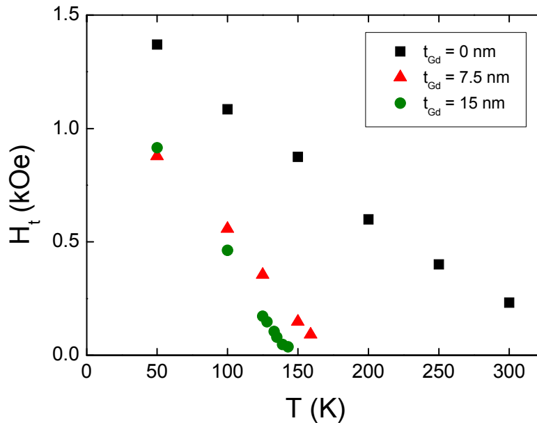
Figure 5. (color online) Temperature dependence of transition field in Gd_{11}Co_{89}/Gd/Gd_{35}Co_{65} trilayers.
