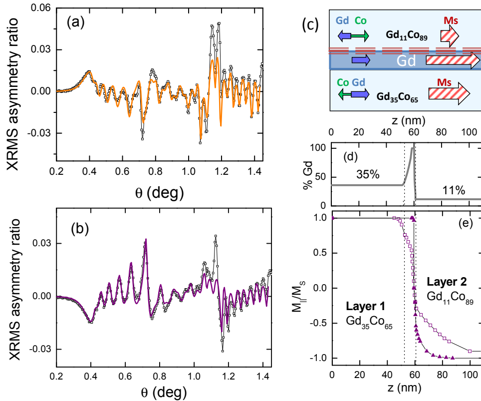
Figure 7. (color online) XRMS asymmetry ratio measured at 50 K at Gd L3 edge with circular polarization for a 50 nm Gd_{35}Co_{65} /7.5 nm Gd/50 nm Gd_{11}Co_{89} trilayer (a) H=0.2 kOe; (b) H = 10 kOe. Solid lines are fits to obtain magnetization depth profiles. (c) Sketch of high field magnetization configuration of the trilayer with iDW. (d) Depth dependence of %Gd obtained from the fit of XRMS data at 0.2 kOe (i.e. uniform magnetization profile). Dashed lines indicate the position of the interfaces according to the structural XRMS reflectivity fit. Note the presence of interdiffused Gd-Co regions with variable composition at Gd-Co/Gd interfaces. (e) Fitted magnetization depth profiles at H = 1.8 kOe (squares) and H = 10 kOe (triangles).
