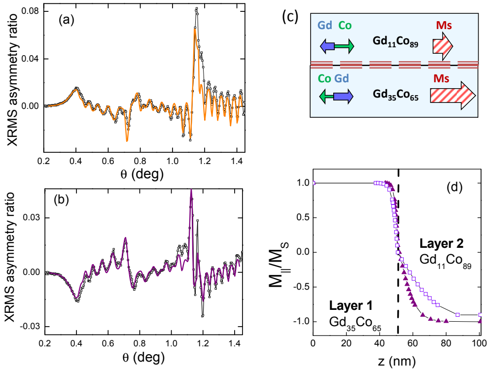
Figure 6. (color online) X-ray Resonant Magnetic Scattering (XRMS) asymmetry ratio measured at 50 K for a 50 nm \text{Gd}_{35}\text{Co}_{65} /50 nm \text{Gd}_{11}\text{Co}_{89} bilayer: (a) H = 0.2 kOe; (b) H = 10 kOe. Solid lines are fits to obtain magnetization depth profiles. (c) Sketch of high field magnetization configuration of the bilayer with iDW. (d) Fitted magnetization depth profiles at H = 1.8 kOe (squares) and H = 10 kOe (triangles). Dashed lines indicates interface between \text{Gd}_{35}\text{Co}_{65} and \text{Gd}_{11}\text{Co}_{89} layers. Note the asymmetric DW width at both sides of the interface.
