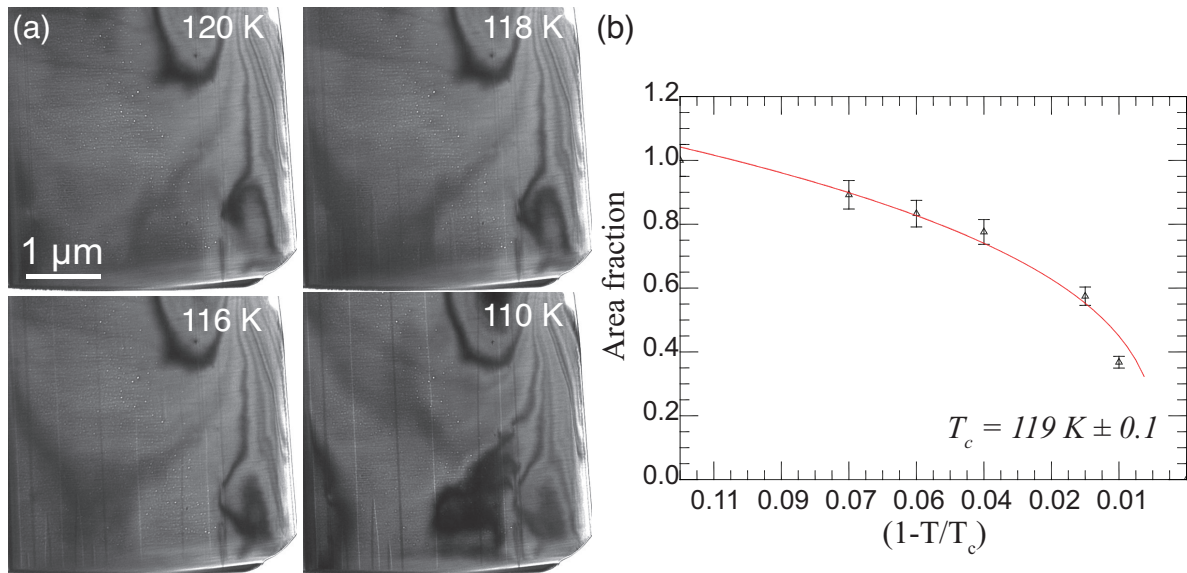
FIG. 4. (a) shows a series of under-focus LTEM images acquired during the cooling of sample S1 from 120 K to 110 K. (b) shows a plot of the area fraction of magnetic domains as a function of reduced temperature (1-T/T_c) as calculated from the in-situ cooling image series (diamonds) and a power-law fit to the data (red line).
