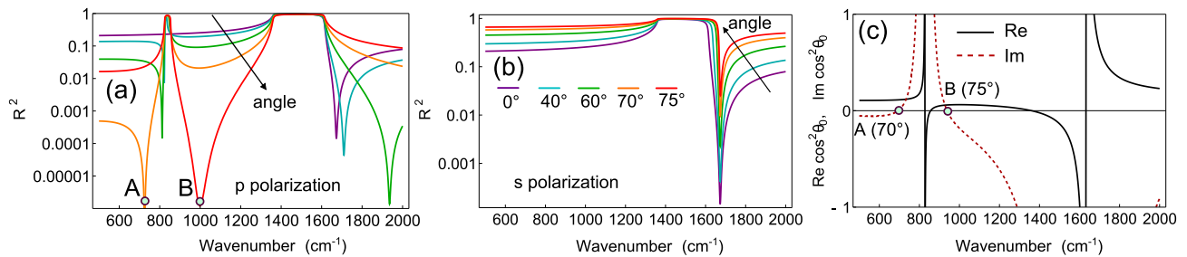
FIG. 3. Reflection by a semi-infinite hBN crystal. (a, b) Calculated reflectance spectra for p and s polarizations, respectively, for a series of different incidence angles. (c) The real and imaginary parts of squared cosine of the perfect absorption angle \theta_0 . At two points denoted by A and B on the graph, \cos^2 \theta_0 becomes real and positive, corresponding to a real-valued incidence angle.
