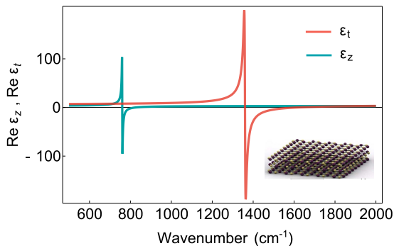
FIG. 2. Frequency dispersion of the real parts of the in-plane ( \varepsilon_t ) and out-of-plane ( \varepsilon_z ) hBN permittivity tensor components. Inset shows the schematic structure of the crystal.
