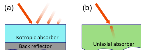
FIG. 1. Concept of an (a) interference-based and (b) interference-less perfect electromagnetic absorber.
