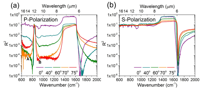
FIG. 5. Experimental reflectivity spectra for a series of incidence angles for (a) p and (b) s polarizations. The points A and B mark the position of perfect absorption points.
