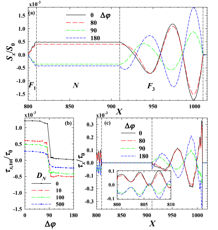
FIG. 12. Panel (a): Normalized x component of the spin current in an SF_1NF_3S Josephson junction vs. position. The geometric widths are D_{F_1} = 10 , D_{F_2} = 100 , and D_N = 100 . There is moderate interface scattering with H_B = 0.5 (see e.g., Fig. 4(a)). The dashed vertical lines mark the interfaces. Panel (b) The total torque \tau_{x,\text{tot}} acting within the F_1 region as a function of \Delta\phi . Several normal metal widths are considered, see legend. The D_N = 0 case has been shifted downwards by 4 \times 10^{-3} for comparison purposes. In panel (c) the x -component of the local torque is shown vs. position with the same phase differences used in (a). The inset is a magnification of the torque within the narrow F_1 region ( 800 < X < 810 ).
