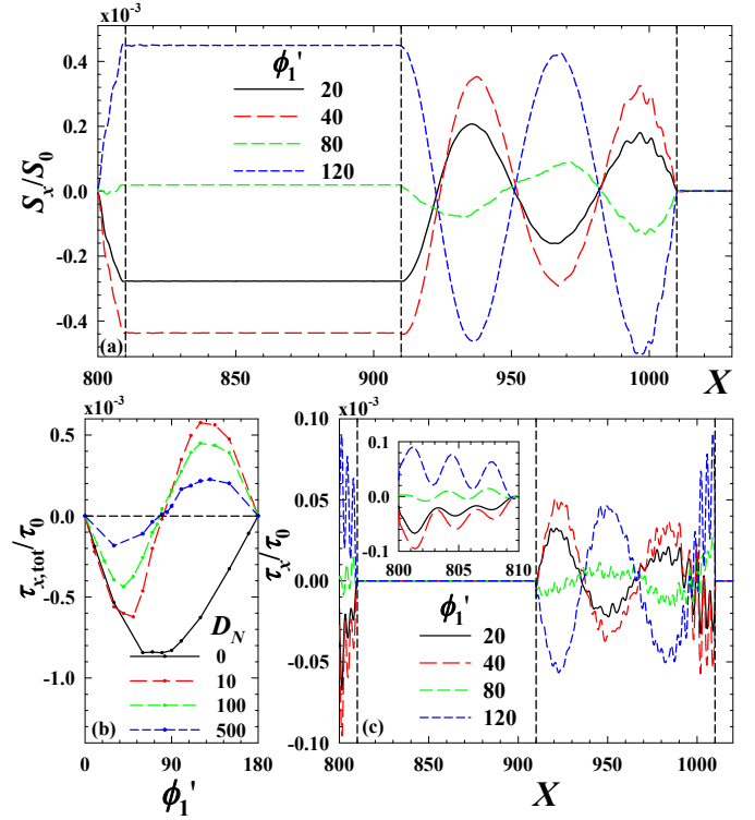
FIG. 13. Panel (a): Normalized spin current in an SF_1NF_3S Josephson junction as a function of position. The geometric widths are D_{F1} = 10 , D_{F2} = 100 , and D_N = 100 . The interface scattering strength is set to H_B = 0.8 . These values are the same as in Fig. 6(b). The dashed vertical lines mark the interfaces. Panel (b) illustrates the total torque \tau_{x,\text{tot}} within the F_1 region as a function of the relative in-plane magnetization angle, \phi_1' . Several normal metal widths are considered as depicted in the legend. The D_N = 0 results have been multiplied by 1/5 for comparison purposes. In panel (c) the x -component of the torque is shown as a function of position for the same case considered in (a).
