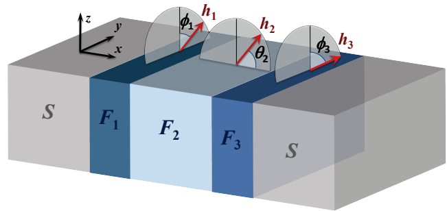
FIG. 1. Schematic of the SF_1F_2F_3S Josephson junction considered in this paper. A generic configuration is shown, described by the in-plane magnetization angles, \phi_i , and the out-of-plane angles, \theta_i ( i = 1, 2, 3 ). The ferromagnetic exchange field \mathbf{h}_i in each region is expressed as \mathbf{h}_i = h_i(\cos \theta_i, \sin \theta_i \sin \phi_i, \sin \theta_i \cos \phi_i) .
