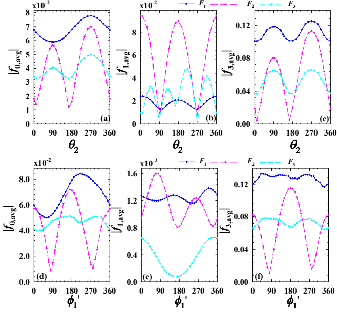
FIG. 11. Normalized triplet |f_{0,\text{avg}}| , |f_{1,\text{avg}}| , and singlet |f_{3,\text{avg}}| amplitudes, averaged over the F regions indicated on the overhead legends, plotted as functions of \theta_2 and \phi'_1 . The geometrical and material parameters corresponds to the D_{F_3} = 100 cases presented in Fig. 7.
