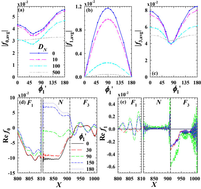
FIG. 10. Top row, panels (a)-(c): Normalized singlet and triplet correlations versus in-plane relative magnetization angle \phi'_1 \equiv \phi_1 + 90^\circ for a SF_1NF_3S structure. The magnitudes of these pair correlations are averaged over the F_3 region. The geometrical and material parameters are the same as in Fig. 6(b). The bottom panels (d) and (e) correspond to the local spatial behavior of the triplet correlations for the D_N = 100 case studied in the top panels. The two F regions are plotted in separate frames to discern the triplet correlations in the narrow F_1 region. The dashed vertical lines represent the interface between the N and F_3 regions. Several values of \phi'_1 are considered, as shown in the legend.
