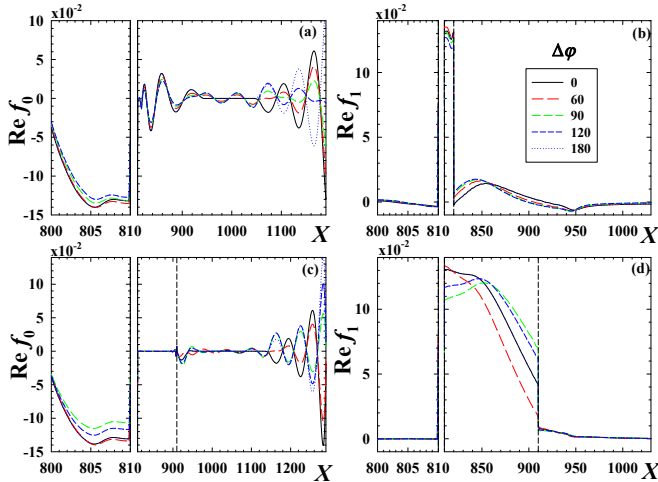
FIG. 9. Normalized triplet correlations in an SF_1NF_3S Josephson junction as a function of position. The F layers have widths D_{F1} = 10 and D_{F3} = 380 , and H_B = 0 , corresponding to the parameters used in Fig. 4(c). The top set of panels relate to structures with a normal metal spacer, N , of width D_N = 10 , while the bottom set represent a larger N layer with D_N = 100 . The dashed vertical lines represent the interface between the N and F_2 regions. Various phase differences \Delta\varphi are considered (see legend). The magnetization in F_1 is along z , while it is along y in F_2 .
