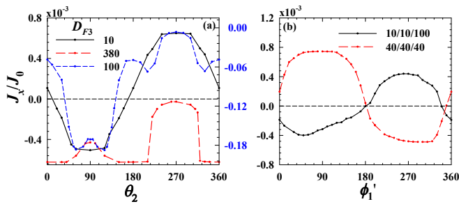
FIG. 7. Normalized Josephson current for a SF_1F_2F_3S junction versus (panel (a)) the out-of-plane angle \theta_2 (see Fig. 1), and (panel (b)) the in-plane angle \phi_1' . A set phase difference \Delta\varphi = 100^\circ is assumed for all cases. In (a), F_1 and F_2 have widths D_{F_1} = D_{F_2} = 10 , and the legend lists the three F_3 widths considered. The exchange field points along the y direction in F_3 and the z direction in F_1 . The right vertical axis is for the D_{F_3} = 100 case only. For the D_{F_3} = 380 case, there is no interface scattering ( H_B = 0 ), while the remaining D_{F_3} cases have H_B = 0.8 . In (b) \theta_1 = 90^\circ , and \mathbf{h} is directed along y in F_2 , and along z in F_3 . The legend indicates the F layer widths of the two trilayer ferromagnet structures considered: they have the same total width. Interface scattering in both cases is H_B = 0.8 .
