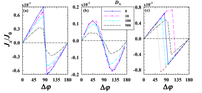
FIG. 4. Normalized Josephson current versus \Delta\phi for a SF_1NF_3S structure. The legend labels the N spacer widths, D_N . The relative in-plane magnetization angle between the two F layers is 90^\circ . For panels (a) and (b), the layers F_1 and F_3 have widths D_{F1} = 10 , and D_{F3} = 100 . In panel (a) H_B = 0.5 , in panel (b) H_B = 0.8 , and in panel (c), H_B = 0 , with ferromagnet widths D_{F1} = 10 , and D_{F3} = 380 . In panel (c) the additional dotted curve corresponds to D_N = 5 , illustrating the sensitivity of the current phase relation to D_N .
