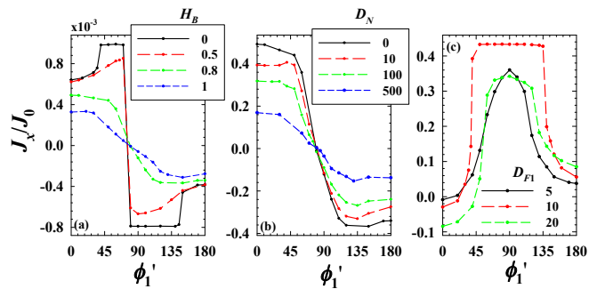
FIG. 6. Normalized Josephson current versus the in-plane relative magnetization angle \phi'_1 \equiv \phi_1 + 90^\circ (see text), for a SF_1F_2S junction (panel (a)), and for an SF_1NF_3S junction with H_B = 0.8 (panel (b)). The legends show the geometric and material parameters that are varied. In (a) \Delta\varphi = 100^\circ , D_{F_1} = 10 , and D_{F_2} = 100 . In (b) \Delta\varphi = 100^\circ , D_{F_1} = 10 , and D_{F_3} = 100 . In (c) an SF_1F_2S junction is considered with H_B = 0 and \Delta\varphi = 60^\circ . The outer ferromagnet layer has D_{F_2} = 380 , while three different D_{F_1} values are considered (see legend).
