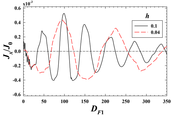
FIG. 8. Normalized Josephson current for a SF_1F_2S structure as a function of F layer width D_{F1} . The other ferromagnet's width is fixed at D_{F2} = 100 . The exchange field is along z in F_1 , and along y in F_2 . The legend indicates two normalized h values: The dashed curve corresponds to h = 0.04 , while the solid curve is for h = 0.1 . The interface scattering parameter is set to H_B = 0.8 , and a phase difference of \Delta\varphi = 100^\circ is maintained across the S electrodes.
