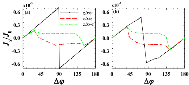
FIG. 5. Normalized Josephson current versus \Delta\varphi for a SF_1F_2F_3S structure. The legend labels the three relative magnetization directions between the F layers. They correspond in order to the configurations labeled N P and AP in the previous figures for F_1 and F_3 , while the intermediate layer F_2 has out-of-plane magnetization. The ferromagnetic layer F_3 has a fixed width corresponding to D_{F_3} = 380 . The adjacent F layers have widths (panel (a)) D_{F_1} = D_{F_2} = 10 , and (panel (b)) D_{F_1} = D_{F_2} = 20 .
