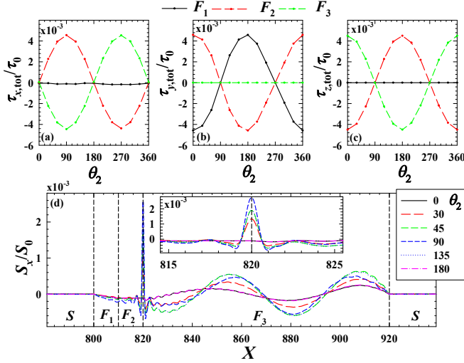
FIG. 14. Top panels: total torque within each of the ferromagnet regions (see overhead legend) in an SF_1F_2F_3S junction as the angle \theta_2 varies. The system parameters are those used in Fig. 7(a). The sum \tau_{i,\text{tot}} ( i = x, y, z ) over all three ferromagnetic regions vanishes for each component. In the bottom panel, the spatial behavior of the normalized x -component of the spin current is shown throughout the system for a few select magnetization orientations \theta_2 (see legend). The inset is a magnification of the region centered around the F_2/F_3 interface located at X = 820 . Vertical dashed lines in the main plot mark interface locations.
