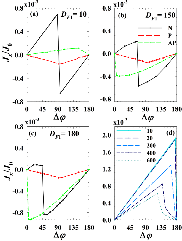
FIG. 3. Normalized Josephson current versus phase difference, \Delta\phi for a SF_1F_2S structure with no interface scattering, H_B = 0 . In panels (a)-(c) various widths of the F regions are considered, each panel labeled by the width D_{F1} of the ferromagnet layer F_1 , with the constraint that D_{F1} + D_{F2} = 390 . The legend in (b) labels the relative magnetization orientation (see Fig. 2). In (d) the magnetization configuration is N, D_{F1} = D_{F2} , and their individual widths are given in the legend.
