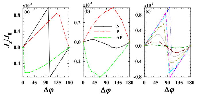
FIG. 2. Normalized (see text) Josephson current versus phase difference, \Delta\phi , for a SF_1F_2S structure with D_{F_1} = 10 , D_{F_2} = 100 , and h = 0.1 . For panels (a) and (b), the legend in (b) labels the relative in-plane magnetization orientations: parallel (P), antiparallel (AP), or normal (N). Two interface scattering strengths are considered: (a) H_B = 0 , and (b) H_B = 1 . In panel (c), the magnetization orientations are fixed in the normal configuration ( \phi_1 = 0 , \phi_2 = 90^\circ ), and the interface scattering is varied as H_B = 0, 0.2, 0.5, 0.6, 0.7, 0.8, 1 (in descending order of peaks).
