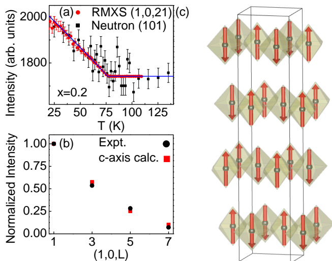
FIG. 7. (a) Intensity dependence of the (1 0 odd) magnetic reflection measured with neutrons at (101) and RMXS at (1,0,21) for \text{Sr}_2\text{Ir}_{0.8}\text{Ru}_{0.2}\text{O}_4 . The RMXS results are fit to a power law and give a transition temperature at T_N=76.3(6) . (b) Experimental intensities for magnetic reflections compared to the calculated intensities for c-axis aligned spins. (c) The magnetic structure for \text{Sr}_2\text{Ir}_{0.8}\text{Ru}_{0.2}\text{O}_4 with spins aligned along the c-axis.
