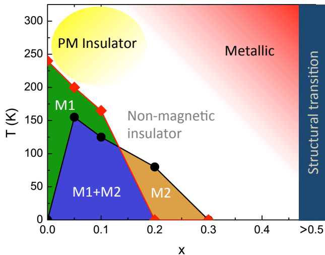
FIG. 10. Phase diagram for \text{Sr}_2\text{Ir}_{1-x}\text{Ru}_x\text{O}_4 . The data points correspond to transition temperatures from single crystal neutron diffraction and RMXS. M1 denotes ab-plane magnetic ordering and M2 indicates c-axis ordering. The insulating regions are based on results presented in Ref. 15.
