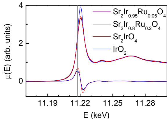
FIG. 1. XANES measurements at the Ir L_3 -edge for \text{Sr}_2\text{Ir}_{1-x}\text{Ru}_x\text{O}_4 , with x=0, 0.05 and 0.2 , and a \text{IrO}_2 standard. The white line absorption intensity and the derivative are both shown for each sample. The same absorption energy of 11.2175 \text{ keV} is observed for all the samples measured indicating a valence of \text{Ir}^{4+} .
