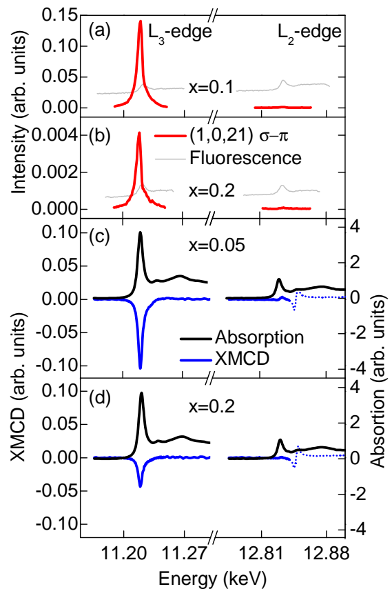
FIG. 8. (a)-(b) Energy scans through the Iridium L_2 and L_3 edges using RMXS on \text{Sr}_2\text{Ir}_{0.9}\text{Ru}_{0.1}\text{O}_4 and \text{Sr}_2\text{Ir}_{0.8}\text{Ru}_{0.2}\text{O}_4 single crystals within the magnetically ordered phase ( T=5 K). The red solid lines correspond to RMXS with polarization of \sigma-\pi . The grey line, a fluorescence measurement, is performed to indicate the energy of the resonant L-edges only and has been scaled to fit on the plot. (c)-(d) XMCD and x-ray absorption energy scans in a \pm 3 T field at 1.8 K for \text{Sr}_2\text{Ir}_{0.95}\text{Ru}_{0.05}\text{O}_4 and \text{Sr}_2\text{Ir}_{0.8}\text{Ru}_{0.2}\text{O}_4 . The variation of the XMCD signal above 12.84 keV (dotted line) is an artifact of the optics rather than from any XMCD signal from the sample.
