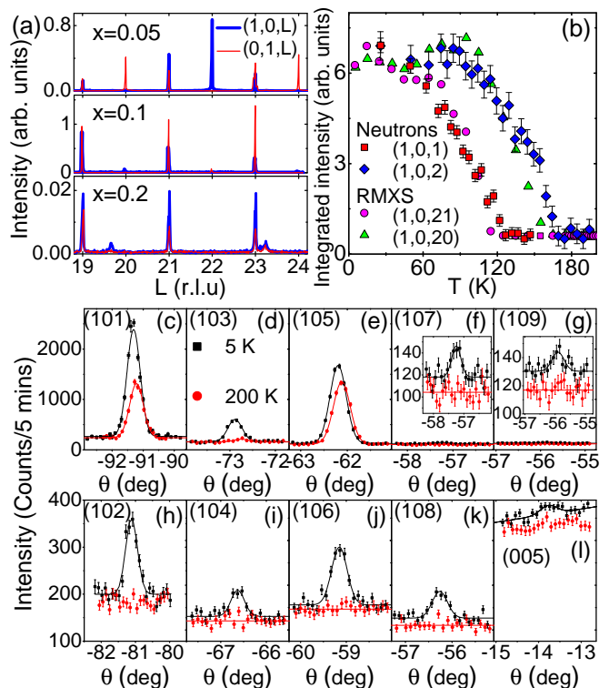
FIG. 3. (a) RMXS measurements on single crystals of \text{Sr}_2\text{Ir}_{1-x}\text{Ru}_x\text{O}_4 with x=0.05, 0.1 and 0.2 . (b) Comparison of the intensity of (1,0,2n+1) and (1,0,2n) magnetic reflections in \text{Sr}_2\text{Ir}_{0.9}\text{Ru}_{0.1}\text{O}_4 measured with both neutrons and RMXS. The neutron and x-ray measurements involved different crystals from the same batch. The intensities have been normalized to their respective background intensities and scaled so all reflections are in a single plot. (c)-(l) Neutron scattering rocking scan measurements on a single crystal of \text{Sr}_2\text{Ir}_{0.9}\text{Ru}_{0.1}\text{O}_4 for several reflections. Scattering is observed at (1,0,L) for both L =odd and L =even.
