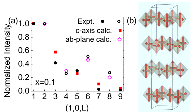
FIG. 6. (a) Experimental neutron scattering intensities for the magnetic reflections in \text{Sr}_2\text{Ir}_{0.9}\text{Ru}_{0.1}\text{O}_4 are compared with calculated magnetic structures for the case of spins in the ab-plane and c-axis. (b) Corresponding magnetic structures within the nuclear unit cell.
