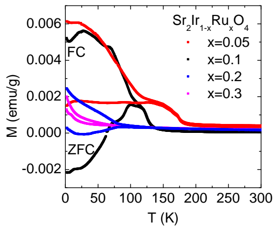
FIG. 2. Magnetization measurements on single crystals in the series \text{Sr}_2\text{Ir}_{1-x}\text{Ru}_x\text{O}_4 for x=0.05, 0.1, 0.2 and 0.3 . Field cooled (FC) and zero field cooled (ZFC) results in an applied field of 100 Oe are shown. The ZFC curve is always lower than the FC for all concentrations measured.
