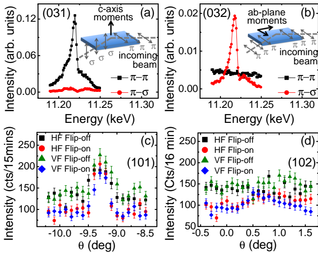
FIG. 4. By performing polarization analysis of (a)-(b) x-ray energy scans and (c)-(d) neutron rocking scans on \text{Sr}_2\text{Ir}_{0.9}\text{Ru}_{0.1}\text{O}_4 single crystals the spin direction associated with the magnetic reflections is determined. Both measurements were performed at 5 K.
