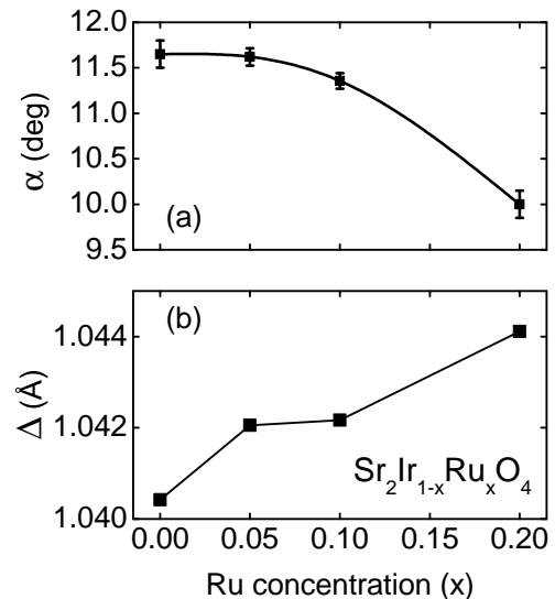
FIG. 9. Single crystal neutron diffraction on \text{Sr}_2\text{Ir}_{1-x}\text{Ru}_x\text{O}_4 for x=0, 0.05, 0.1 and 0.2 at 50 K. (a) The octahedral rotation in the ab -plane ( \alpha ). (b) Tetragonal distortion of the octahedra due to the difference between Ir-O bonds in the ab -plane and along the c -axis ( \Delta_{\text{Ir-O}} ).
