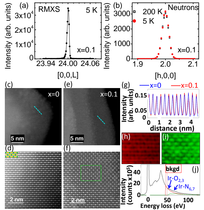
FIG. 5. (a) Single crystal synchrotron x-ray diffraction measurements of \text{Sr}_2\text{Ir}_{0.9}\text{Ru}_{0.1}\text{O}_4 indicated no splitting of diffraction peaks, consistent with a homogenous sample. (b) Neutron diffraction additionally found no evidence for structural phase separation. (c)-(j) High Resolution Z-STEM analysis of \text{Sr}_2\text{Ir}_{1-x}\text{Ru}_x\text{O}_4 samples. (c) and (d), Z-contrast images of \text{Sr}_2\text{IrO}_4 at different magnifications with the beam parallel to [201]. Inset in (d) is a schematic model of the crystal with the Ir columns in green, the Sr columns in yellow and the O columns (not imaged) in cyan. (e) and (f), Z-contrast images of \text{Sr}_2\text{Ir}_{0.9}\text{Ru}_{0.1}\text{O}_4 with the same zone axis and the same magnification as in (c) and (d). (g) Line profile along the cyan segments in (c) and (e), showing the intensity (proportional to Z^2 ) of the Ir columns in \text{Sr}_2\text{IrO}_4 and \text{Sr}_2\text{Ir}_{0.9}\text{Ru}_{0.1}\text{O}_4 samples. (h) Uniform thickness map and (i) Ir map of the region indicated with a green rectangle in (f). (j) Electron energy-loss spectrum from the region within the green rectangle in (f) showing the Ir edges used to generate the Ir map by plotting their combined integrated intensity. The red curve is a power-law background fitting function and the green curve shows the background-removed Ir edges.
