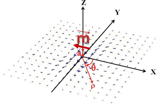
FIG. 10. The screening current ( J ) induced in a superconductor due to a point magnetic dipole \vec{m} with a distance “ a ” above the superconducting surface plane ( Z = a ). \rho and \theta are the radial distance and azimuth angle respectively. Surface current calculation from Ref. [44].
