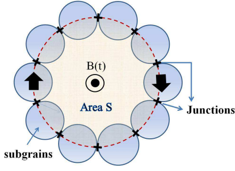
FIG. 8. Schematic illustration of an induced screening current loop created by the magnetic field pointing out of the paper. Multiple defects such as subgrains are connected by weak link Josephson junctions between the defects. Note S is the area of the screening current loop. The arrow directions illustrate the direction of diamagnetic current. This figure indicates 10 Josephson junctions.
