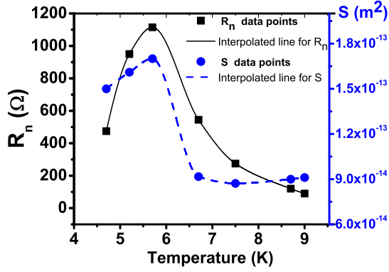
FIG. 12. Temperature dependent fitting parameters R_n (normal resistance of the junction as square symbols) and S (area of the induced screening current loop as circle symbols). Each value is determined by the fitting method of the phase slip model from the P_{3f} versus P_f data in Fig. 6. Note that all data points for both R_n and S are connected by an interpolation spline function.
