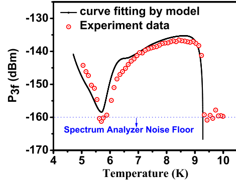
FIG. 13. Temperature dependence of the third harmonic response for the bulk Nb sample at the excitation power 5.5 dBm and excitation frequency 5.025 GHz measured by the magnetic write head probe (dot points). The noise floor of the spectrum analyzer at this excitation frequency is about -161 dBm. A calculated result (solid curve in black) based on the phase slip model is fit to the data. The fitting parameter is B_{rf} = 11.75 mT , with fixed values for the remaining parameters: l_{gap}=100 nm , N = 10 , a = 100 nm .
