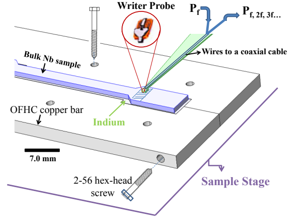
FIG. 4. The setup inside the cryostat probe station for measuring the bulk Nb nonlinearity. The slashed region on the top of the bulk Nb sample indicates where the P_{3f} measurements are performed. The circled zoom-in picture schematically highlights the magnetic write head probe on the surface of the bulk Nb. Note that thermal anchoring is critical for cooling the bulk Nb sample below T_c .
