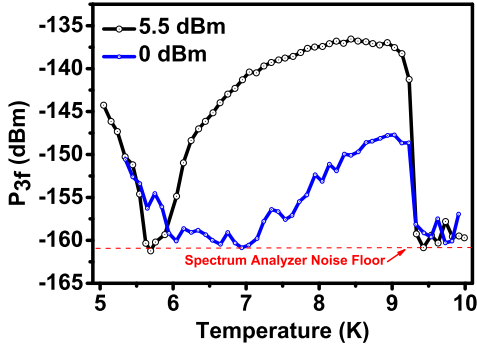
FIG. 7. The temperature dependent P_{3f}(T) (measured as temperature decreases) of the bulk Nb sample at two specific input powers and 5.025 GHz excitation. Note the T_c of the bulk Nb sample is 9.2 K and the onset of nonlinearity at low excitation power also begins at exactly 9.2 K.
