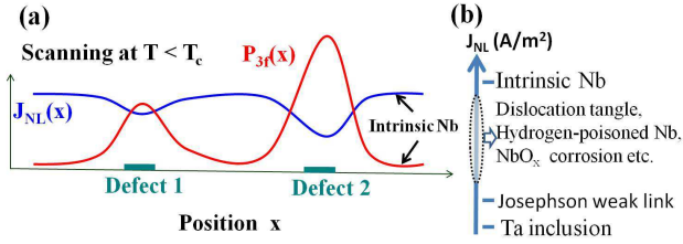
FIG. 2. (a) Schematic J_{NL} variation on the superconducting surface from intrinsic Nb to different discrete defects. The P_{3f} generation from defects is local. The defects with greatest disruption of the superfluid density have the lowest J_{NL} and strongest P_{3f} . Hence measuring P_{3f} at different positions can be used to find defects on superconductors. (b) A speculative schematic hierarchy of a few representative defects and their associated J_{NL} values. The dashed oval region indicates the unknown order of J_{NL} hierarchy for these types of defects.
