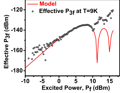
FIG. 11. Effective P_{3f} versus P_f for the bulk Nb sample measured by the magnetic write head probe at 9 K under 5.025 GHz excitation as shown by the dot points. The solid line is the theoretical calculation based on the phase slip model of the Josephson junction. The parameters are as follows: T=9.0 \text{ K} , Frequency=5.025 GHz, R_n = 90 \Omega , S = 9.11 \times 10^{-14} \text{ m}^2 , a = 100 \text{ nm} , N=10 , l_{gap} = 100 \text{ nm} . Only R_n and S were varied to perform the fit.
