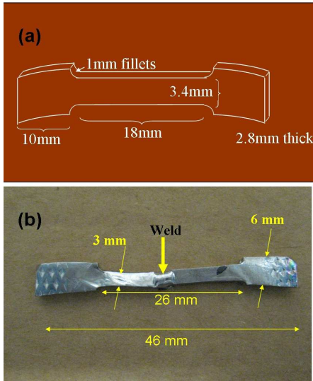
FIG. 3. (a) A schematic picture of the bulk Nb tensile specimen before deformation. All dimensions of the specimen are labeled. (b) The finished specimen after tensile test and welding treatment in the center of the sample.
