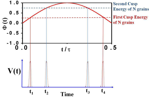
FIG. 9. (Upper frame) Normalized magnetic flux without the presence of DC field ( \Phi(t) = \Phi_{rf} \sin(\omega t) ). This figure assumes the cusps of the energy appear when \Phi = 0.25 and 0.75 . (Bottom frame) The generated voltage spikes in a half of RF cycle ( \tau ) due to the presence of phase slips of Josephson junctions in the loop of N subgrains.
