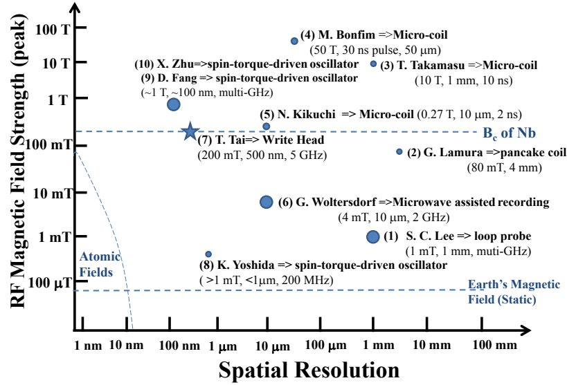
FIG. 1. High-Field, High-Resolution AC/Transient Magnetic Microscopy Generating Highly-Confined Magnetic Fields with Frequency \geq 100 MHz : A selected summary of methods to generate a highly concentrated RF magnetic field. Each technique lists a typical RF magnetic field scale, degree of spatial confinement/resolution, and an associated time/frequency scale demonstrated. All of the candidate technologies are numbered and referenced as follows (1) S. C. Lee \Rightarrow loop probe. [10] [11] [12]. (2) G. Lamura \Rightarrow pancake coil [15] (3) T. Takamasu \Rightarrow micro-coil [16] (4) M. Bonfim \Rightarrow micro-coil [17] (5) N. Kikuchi \Rightarrow micro-coil [18] (6) G. Woltersdorf \Rightarrow microwave assisted recording [19]. (7) T. Tai \Rightarrow magnetic write head [26][28]. (8) K. Yoshida \Rightarrow spin-torque-driven oscillator [20]. (9) D. Fang \Rightarrow spin-torque-driven oscillator [21]. (10) X. Zhu \Rightarrow spin-torque-driven oscillator [22]. Note that larger circle (●) and star sign (★) indicates the operation frequency/speed corresponds to higher frequencies. The star sign also indicates the method used in this paper.
