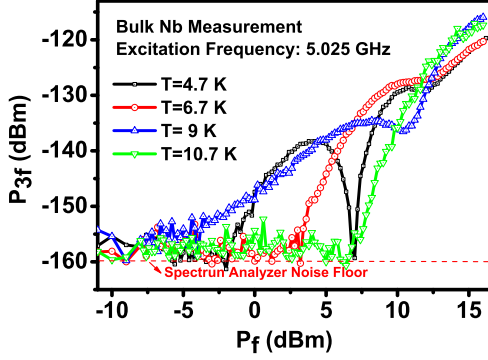
FIG. 6. The P_{3f} dependence on P_f at selected temperatures on the bulk Nb sample with the magnetic write head probe. The P_{3f} dependence on P_f at 4.7 K shows a different nonlinear behavior compared to the other two temperatures. The nonlinearity of the probe is measured at T=10.7 K in this data set.
