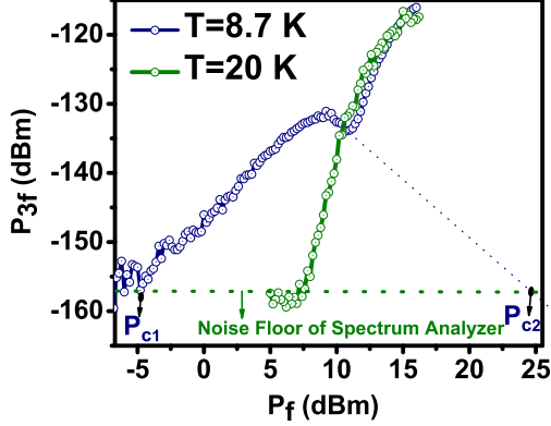
FIG. 5. The P_{3f} dependence on P_f at a selected temperature, 8.7 K, for local microwave excitation of bulk Nb with the magnetic write head probe. Note the T_c of the bulk Nb sample is 9.2 K. The P_{3f} at T=20 K results from the probe nonlinearity itself.
