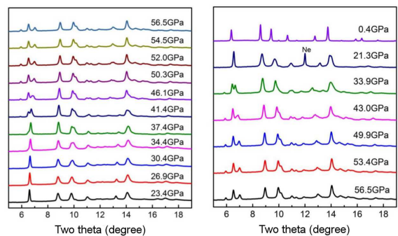
FIG. 2. (Color online) X-ray diffraction patterns of V_2O_3 as a function of pressure at room temperature (left panel - compression, right panel - decompression).
