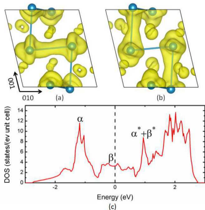
FIG. 5. (Color online) The partial charge densities and density of states (DOS) of high pressure phase V_2O_3 at 50 GPa. The isosurfaces of the partial charge densities in the HP phase V_2O_3 are shown for (a) the energy range of -2.8 to -0.7 eV at the isosurface level of 0.03 \text{ e}/\text{\AA}^3 , (b) the energy range of -0.7 to 0 eV at the isosurface level of 0.007 \text{ e}/\text{\AA}^3 . Only the V atom are shown (blue spheres). For simplicity, oxygen atoms are not shown. (c) The total DOS of the HP phase V_2O_3 at 50 GPa. \alpha , \beta and \alpha^* , \beta^* represent bonding and antibonding orbitals.
