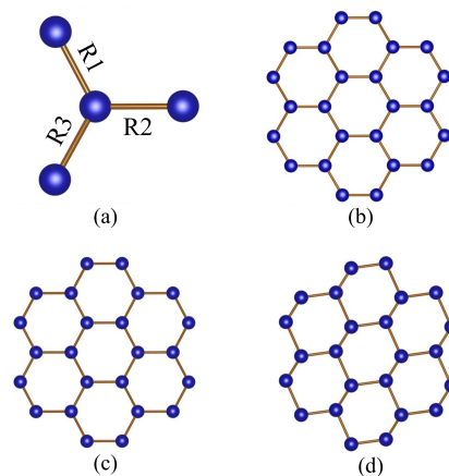
FIG. 4. (Color online) (a) Each vanadium atom in V_2O_3 has three nearest neighbors with three bond lengths (R1, R2 and R3), with blue spheres representing the vanadium atom. The puckered honeycomb lattices in the basal plane for (b) the room temperature phase with R1=R2=R3 , (c) the low temperature phase with R2 > R1 \approx R3 below 150K, and (d) the high pressure phase with R3 < R2 < R1 above 47 GPa. For simplicity, oxygen atoms are not shown.
