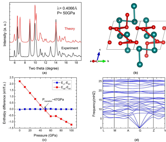
FIG. 3. (Color online) (a) Comparison of theoretical and experimental X-ray powder diffraction patterns of the high pressure phase V_2O_3 . (b) The V-V bond structure in high pressure monoclinic V_2O_3 . The teal and red balls represent the vanadium and oxygen atoms, respectively. (c) The pressure evolution in the relative enthalpies of high pressure and low temperature monoclinic structures from static calculations. The dashed line indicates zero enthalpy difference. (d) Phonon dispersion curves for the high pressure monoclinic structure at 50 GPa.
