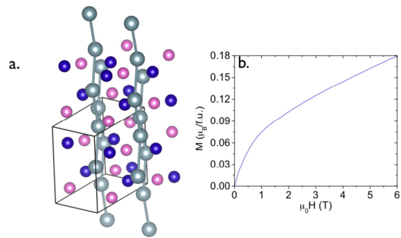
FIG. 1: Color online: a. The crystal structure of UCoGe. The grey atoms are U atoms showing the zig-zag alignment, dark blue are Co and purple are Ge. The box outlines the unit cell. b. Bulk magnetization of UCoGe at 1.8 K along the c -axis, measured with a SQUID which includes both the spin and orbital moments.
