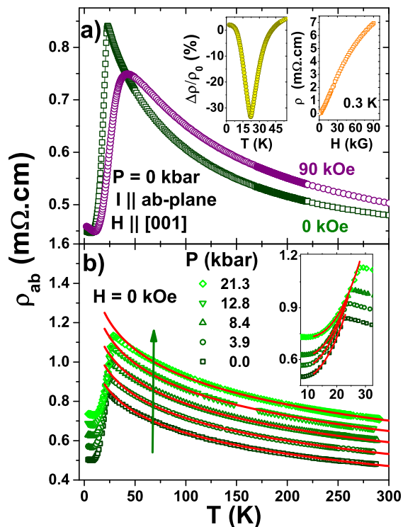
FIG. 3: (a) Temperature dependence of the electrical resistivity, \rho(T) , at H = 0, 90 kOe. The right inset shows the resistivity at 0.3 K as a function of magnetic field and the left inset shows the temperature dependence of MR, defined as \Delta\rho/\rho_0(\%) = [\rho(H = 90 \text{ kOe}, T) - \rho(H = 0 \text{ kOe}, T)] \times 100/\rho(0, T) . (b) \rho(T) for different values of applied hydrostatic pressure up to 21 kbar. An offset of 0.05 m \Omega cm was used for clarity. Solid lines display the best fits of the data to Eq. (2). The inset shows the low-T behavior for selected pressures and the corresponding fits (solid lines) to Eq. (3).
