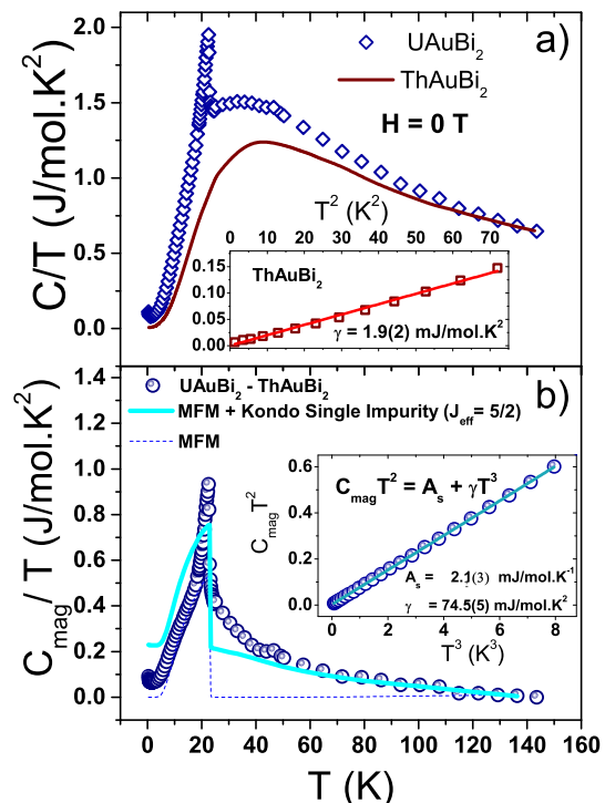
FIG. 2: a) Temperature dependence of the specific heat of UAuBi 2 and its non-magnetic reference compound ThAuBi 2 . The inset shows a linear fit of C(T)/T vs T^2 for ThAuBi 2 . (b) Magnetic contribution to the specific heat of UAuBi 2 as a function of the temperature and the corresponding fits using a mean field model (dashed lines) and an additional single impurity term (solid lines). The inset shows a linear fit to the data in a CT^2 vs T^3 plot.
