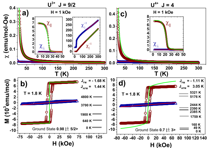
FIG. 1: a) Temperature dependence of the magnetic susceptibility measured with H = 1 \text{ kOe} applied parallel, \chi_{\parallel} , and perpendicular, \chi_{\perp} , to the c -axis. Left inset shows the FM transition at 22.5 \text{ K} . Right inset shows the inverse susceptibility. (b) Magnetization as a function of the magnetic field applied parallel (open circles) and perpendicular (open triangles) to the c -axis at T = 1.8 \text{ K} . The solid lines are the best fits of the data to the \text{U}^{3+} CEF mean field model. Figs. 1c-d displays the same data of Figs. 1a-b with the best fits assuming a \text{U}^{4+} scheme.
