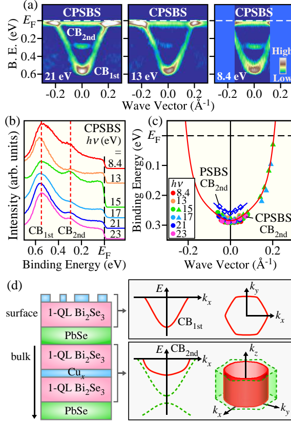
FIG. 3: (Color online) (a) Second-derivative ARPES intensity around the \bar{\Gamma} point for CPSBS at various photon energies plotted as a function of binding energy and wave vector. CB_{1st} and CB_{2nd} denote the conduction bands stemming from the topmost 1-QL Bi_2Se_3 unit and the second Bi_2Se_3 unit located beneath the PbSe layer, respectively. (b) Comparison of the EDC at the \bar{\Gamma} point measured with various photon energies. (c) Photon-energy dependence of the band dispersion for CB_{2nd} in CPSBS extracted from the second-derivative intensities. Filled circles and triangles represent the results for the fresh and aged surfaces, respectively. Detailed procedures used to extract the data points for the aged surface are presented in Figs. 2(j)-2(l) and Supplemental Material 28 . Red curve is a guide for the eyes to trace the band dispersion. The band dispersion for PSBS measured with h\nu = 21 eV is also plotted by open diamonds. (d) Schematic illustration of the band dispersion and the Fermi surface in the topmost and the second Bi_2Se_3 units in CPSBS.
