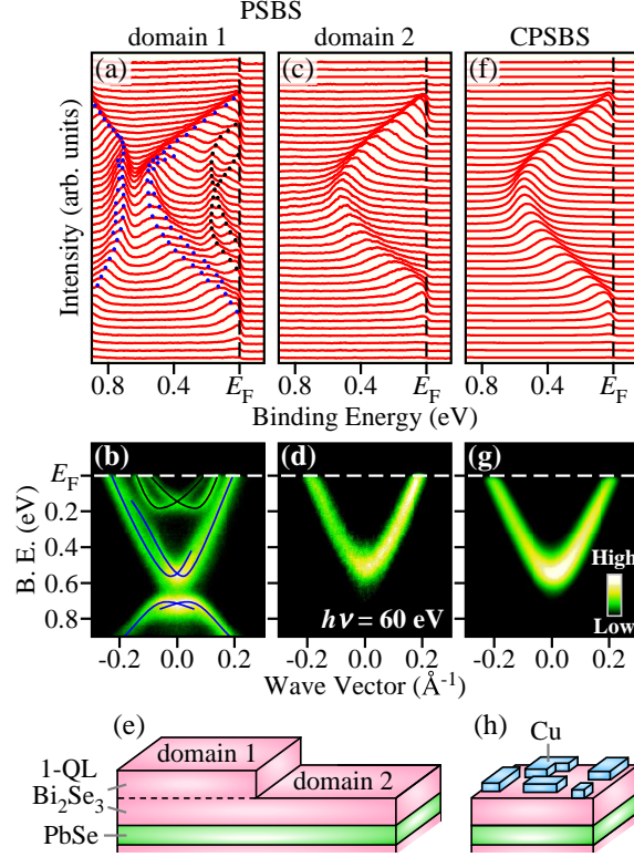
FIG. 1: (Color online) (a)-(d) Comparison of near- E_F energy distribution curves (EDCs) around the \bar{\Gamma} point [(a) and (c)] and corresponding ARPES intensity [(b) and (d)]. The data in (a),(b) and (c),(d) were taken on different domains of the cleaved surface of pristine (\text{PbSe})_5(\text{Bi}_2\text{Se}_3)_6 (PSBS). All the data have been obtained at T = 30 K with 60-eV photons. Black and blue dots in (a) [as well as black and blue curves in (b)] are a guide to the eyes to trace the dispersions of bulk conduction band and gapped Dirac-cone bands, respectively. (e) Schematic illustration of the cleaved surface of PSBS. (f),(g) Near- E_F EDCs and corresponding ARPES intensity plot, respectively, for \text{Cu}_{1.47}(\text{PbSe})_5(\text{Bi}_2\text{Se}_3)_6 (CPSBS) measured with h\nu = 60 eV. (h) Schematic illustration of the cleaved surface of CPSBS.
