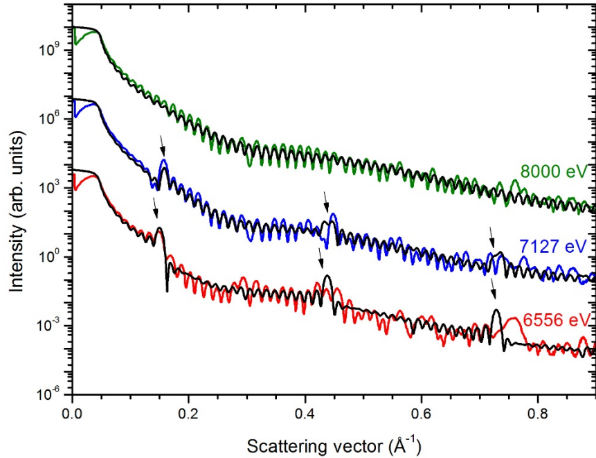
Fig. 2: Experimental (colored) and simulated (black) XRR spectra acquired with x-ray energies of 8000 eV, 7127 eV (near Fe K edge), and 6556 eV (near Mn K edge). Optimized parameters used to simulate XRR spectra are listed in Table I. Features in resonant XRR spectra corresponding to a periodicity of 4.4 nm are indicated by arrows.
