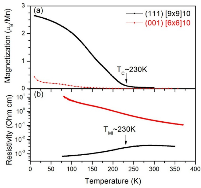
Fig. 3: Temperature dependence of (a) magnetization and (b) resistivity for a (111)-oriented [9x9]10 superlattice and (001)-oriented [6x6]10 superlattice.
