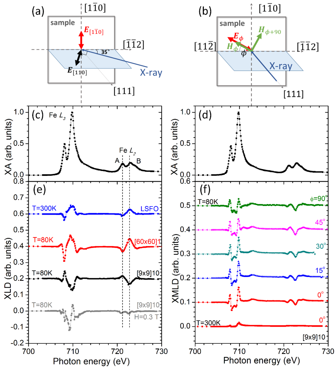
Fig. 5: (a-b) Schematics of the two XMLD measurement geometries; (c-d) XA spectra of the (111)-oriented [9 \times 9]10 superlattice measured in (c) geometry 1, and (d) geometry 2 with \phi = 0^\circ ; (e) Comparison of XMLD(1) spectra for three (111)-oriented samples; The (111)-oriented [9 \times 9]10 superlattice was measured without (black) and with (grey) a magnetic field of 0.3 T applied along the x-ray beam direction. (f) \phi angular dependence of XMLD(2) spectra of the (111)-oriented [9 \times 9]10 superlattice.
