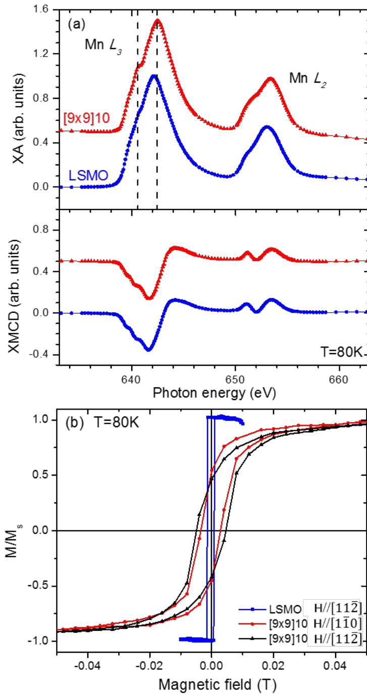
Fig. 4: (a) Mn XA and XMCD spectra, and (b) Mn XMCD hysteresis loops for the (111)-oriented [9x9]10 superlattice and LSMO thin film
