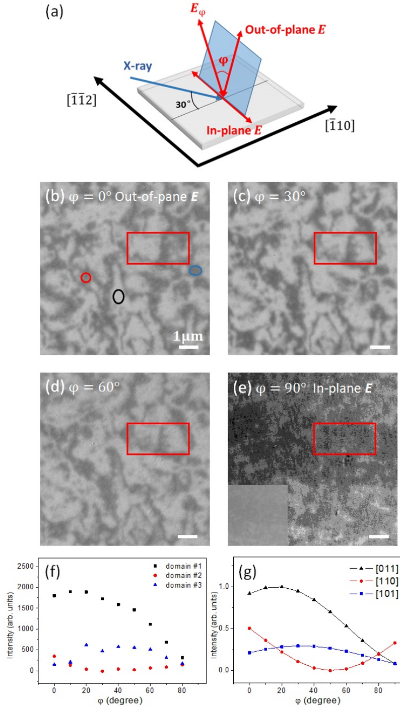
Fig. 6 (a) Measurement geometry of X-PEEM. \varphi is defined as the angle between the x-ray polarization and the plane of incidence. (b-e) AF domain image of the (111)-oriented [9\times 9]10 superlattice taken at 100 K with (b) \varphi = 0^\circ (out-of-plane E ), (c) \varphi = 30^\circ , (d) \varphi = 60^\circ , and (e) \varphi = 90^\circ (in-plane E ). The contrast in (e) has been enhanced in order to more clearly see the features, while the inset shows the image at the same contrast level as in (b-d). (f) The variation of the intensity with \varphi for three domains circled in Fig. 6(b) (black: domain #1, red: domain #2, and blue: domain #3). (g) The calculated intensity for domains with the AF spin axis along the [011] , [110] , and [101] directions.
