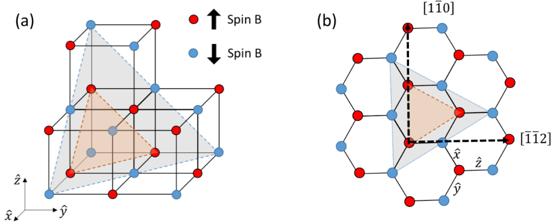
Fig. 1: (a) Schematic of a G-type AF perovskite oxide ABO 3 with the A-site cations and oxygen anions omitted. Red and blue spheres represent two sets of B-site cations with antiparallel spins. The red and blue triangles denote (111) planes with all spin up / spin down B-cations. (b) 2D projection of (111) planes resulting in a honeycomb-like structure. \langle \bar{1}\bar{1}2 \rangle and \langle 1\bar{1}0 \rangle are the two low-index families of directions in the (111) plane.
