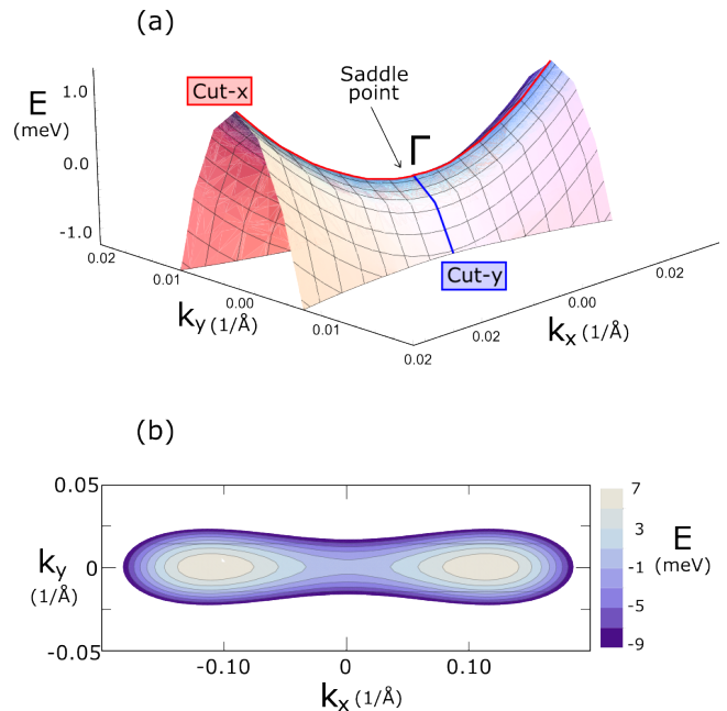
Figure 2: (Color online) (a) 3D plot of the phosphorene valence band around the VHS ( \Gamma point) (PBEsol functional). Cut-x(y) indicates the \Gamma - X ( Y ) path used in the band structure calculation. (b) 2D contour plot of the valence band in a larger region around \Gamma . The contour lines are drawn at 2 meV intervals. The energy at the VHS is set to zero in both plots.
