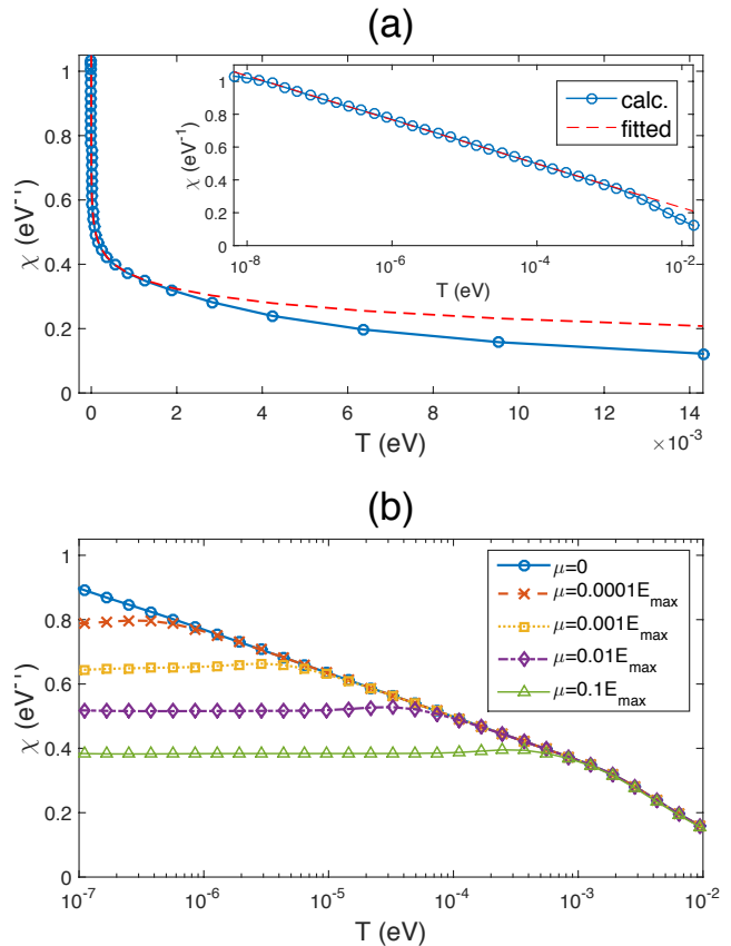
Figure 3: (Color online) (a) Temperature dependence of the bare spin susceptibility \chi calculated directly from Eq. (6) (blue dots) or approximated with the logarithmic divergence in Eq. (7) (dashed red line). The low-temperature behaviour for T < T^* \sim 1.5 \text{ meV} is seen in the inset to follow the logarithmic law. The dashed red line is fitted to Eq. (7) with \omega_D = 0.5004 \text{ eV} . The Fermi level is set to E_{\text{VHS}} = 0 . (b) Spin susceptibilities \chi at different Fermi energies \mu . Away from the VHS, the low-temperature logarithmic behaviour stops at T \approx \mu and turns into Pauli susceptibility.
