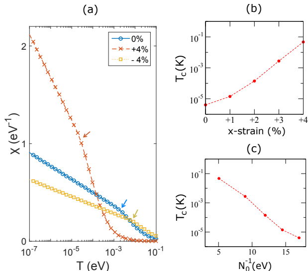
Figure 4: (Color online) Effect of zigzag ridge [ x -axis in Fig.1(a)] strain on the VHS (a) Temperature dependence of the bare spin susceptibility \chi for different strains. The arrows indicate the temperature T^* at which the susceptibility starts to deviate from the logarithmic behaviour. (b) Critical temperature T_c as a function of strain. (c) T_c versus N_0^{-1} . The behaviour of T_c still follows the exponential law of Eq. (10) even if strain is applied.
