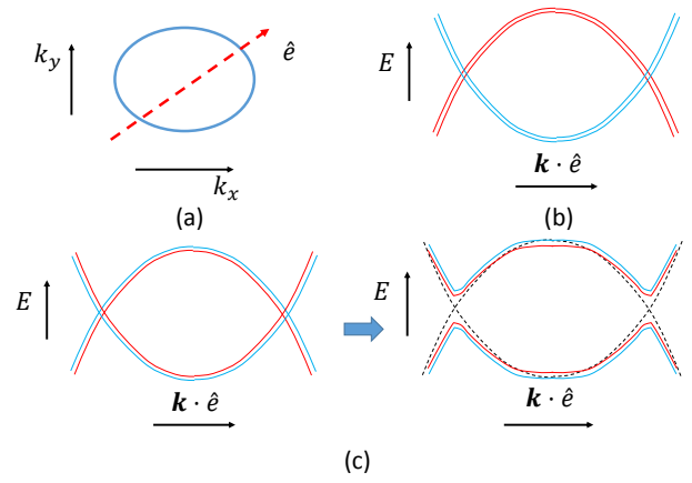
FIG. 2: (a) A band crossing line on some mirror invariant plane at k_z = 0 or k_z = \pi , with an arbitrary cut along which the band structure is plotted. (b) The band structure along the cut in (a) on k_z = \pi , with the corresponding eigenvalues of R_z shown, where the degenerate states of a doublet band have the same eigenvalue. (c) The same band structure on k_z = 0 , where the degenerate states of a doublet band have opposite R_z eigenvalues, which can anti-cross with another doublet band due to the spin mixing enabled by SOC.
