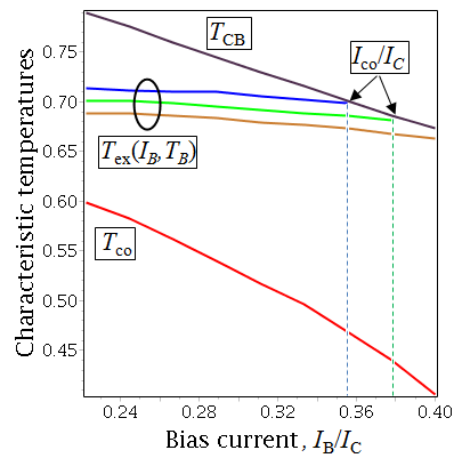
FIG. 9: T_{CB} , T_{ex}(I_B) for T_B=2.0 K (blue), 1.75 K (green) and 0.25 K (orange) and T_{co} as a function of bias current for \lambda = 1550 nm
