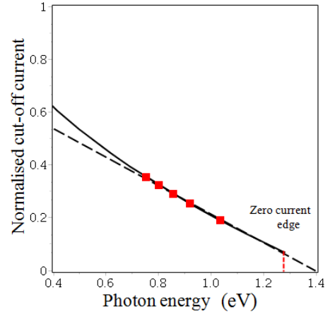
FIG. 12: Cut-off current as a function of photon energy. Solid line - theory, solid boxes - experiment, dashed line - linear extrapolation
