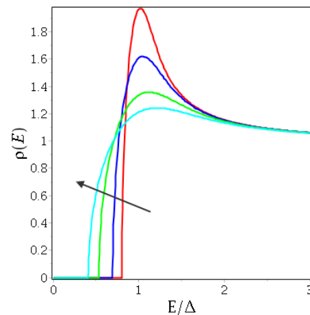
FIG. 1: Normalised density of states in a disordered current-carrying superconductor for different de-pairing energies \Gamma/\Delta = 0.05 (red), 0.1 (blue), 0.2 (green), 0.3 (cyan). The black arrow indicates the direction of increasing pair breaking energy.
