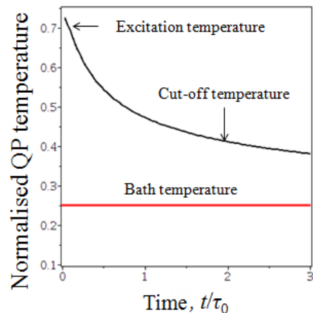
FIG. 7: Temperature evolution in the relaxing hotspot.
