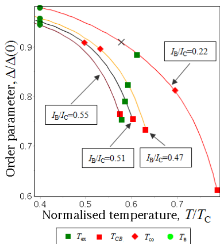
FIG. 14: Hotspot relaxation paths for NbN nanowires at different currents.
