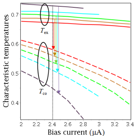
FIG. 6: Hotspot excitation, T_{ex} , (solid lines) and cut-off, T_{co} , (dashed lines) temperatures as a function of bias current for photons of different wavelengths, \lambda = 1200, 1350, 1450, 1550 and 1650 nm. Bath temperature is T_B=250 mK.
