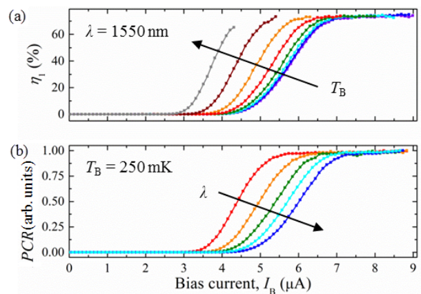
FIG. 10: Single photon system detection efficiency (a) and PCR (b) as a function of temperature and wavelength respectively
