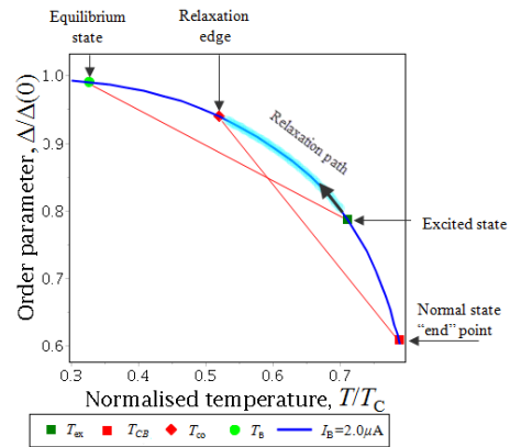
FIG. 4: Different states of a nanowire and relaxation path of the hotspot
