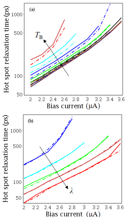
FIG. 13: Hotspot relaxation time, t_{HS} , dependence on deparing energy \Gamma_0 . (a) t_{HS} as a function of bias current for different bath temperatures from 0.25 to 2.0 K with an increment 0.25 K. An arrow indicates increasing bath temperature. Solid curves - \Gamma_0 = 0 , \delta = 325 \text{ meV}^{-1} , \gamma = 0.3 , \tau_0 = 496 \text{ ps} , \Delta T = 500 \text{ mK} ; dash-dot curves, - \Gamma_0 = 0.2\Delta(0) , \delta = 325 \text{ meV}^{-1} , \gamma = 0.3 , \tau_0 = 375 \text{ ps} , \Delta T = 0.25 \text{ K} . (b) t_{HS} as a function of bias current for different wavelengths - 1200, 1350, 1450, 1550, 1650 nm, T_B = 250 \text{ mK} . An arrow indicates increasing wavelength. Solid curves - \Gamma_0 = 0 , \gamma = 0.3 , \tau_0 = 439 \text{ ps} , \delta = 325 \text{ meV}^{-1} ; dash-dot curves - \Gamma_0 = 0.2\Delta(0) , \gamma = 0.3 , \tau_0 = 330 \text{ ps} , \delta = 325 \text{ meV}^{-1} (red)
