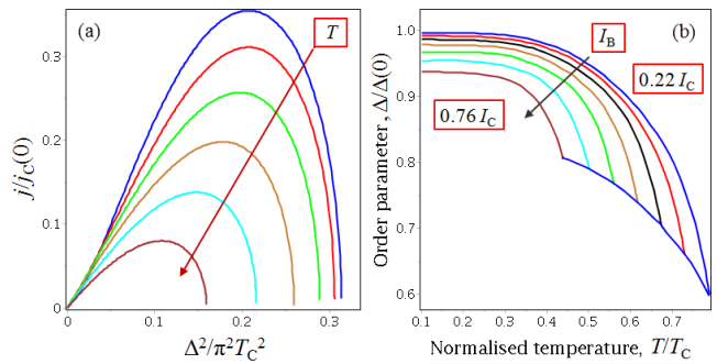
FIG. 2: (a) Dependence of a current in a superconducting nanowire on square order parameter in the interval of temperatures from 0.3T_C to 0.8T_C with 0.1T_C increment from top to bottom. (b) Order parameter as a function of QP temperature in a dirty superconducting nanowire carrying a current. Arrow shows the direction of current increase from 0.22 to 0.76I_C with an increment of 0.09I_C
