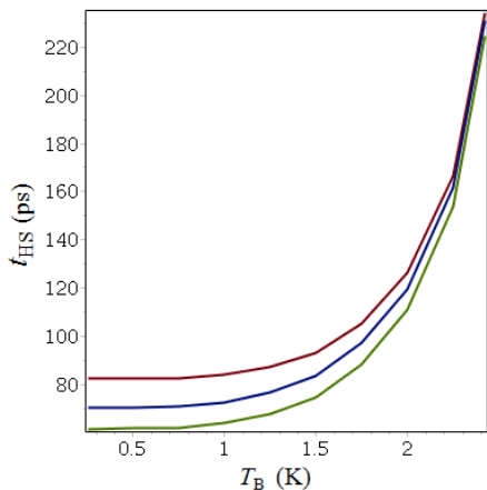
FIG. 8: Hotspot lifetime as a function of bath temperature at fixed bias current I_B=2.0 \mu\text{A} for \gamma=0 -top curve, \gamma=0.3 middle curve, \gamma=3 - bottom curve.
