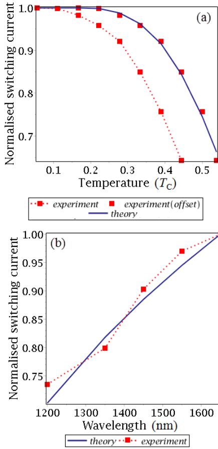
FIG. 11: Normalised cut-off current as a function of bath temperature for \lambda=1550 nm - (a) and wavelength for T_B=250 mK - (b)
