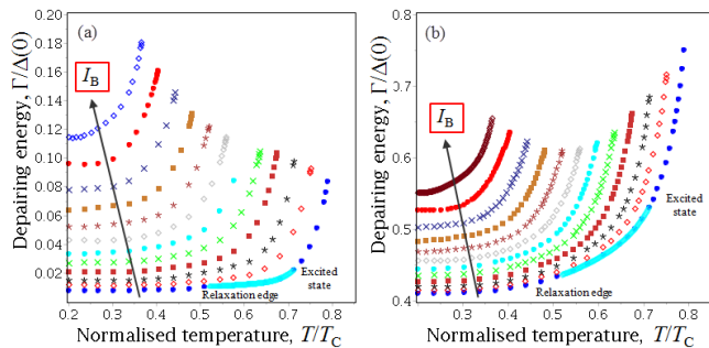
FIG. 5: Ratio of pair-breaking energy to order parameter as a function of temperature in a dirty superconducting nanowire carrying a current. The current increases from 0.22 to 0.83 I_C with an increment of 0.06 I_C in the direction of the arrows: (a) - \Gamma_0 = 0 , (b) - \Gamma_0 = 0.2\Delta(0) . Variations along the relaxation paths are shown for I_B = 2\mu\text{A} (continuous curves)
