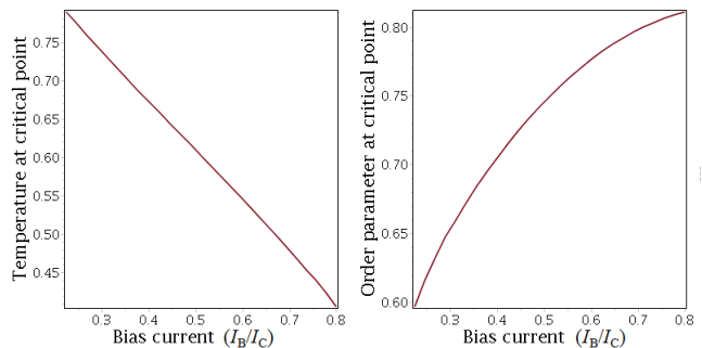
FIG. 3: Dimensionless temperature, T_{CB}/T_C , (a) and order parameter, \Delta_{CB}/\Delta(0) (b) at critical (end) points of relaxation curves in Fig.2 b as a function of dimensionless bias current, I_B/I_C
