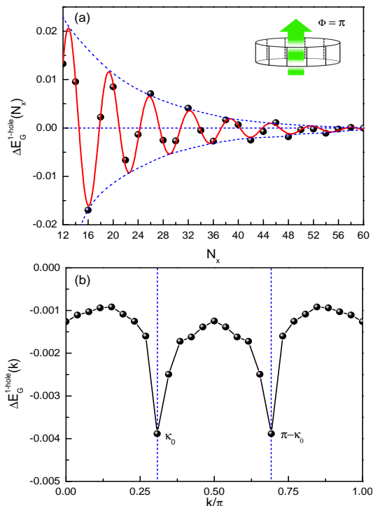
FIG. 5. (Color online) (a) The energy difference \Delta E_G^{1\text{-hole}}(N_x) of a single-hole doped two-leg t - J ladder displays an oscillation in N_x , with the amplitude decaying exponentially when N_x approximately is larger than 12. To calculate the energy we compactify the ladder by “gluing” its two ends and let a magnetic flux of \Phi = \pi pierce through it (upper right). (b) The Fourier transformation of this energy difference exhibits two peaks at \kappa_0 and \pi - \kappa_0 , respectively. Here, \alpha = 13/15 and t/J = 3 .
