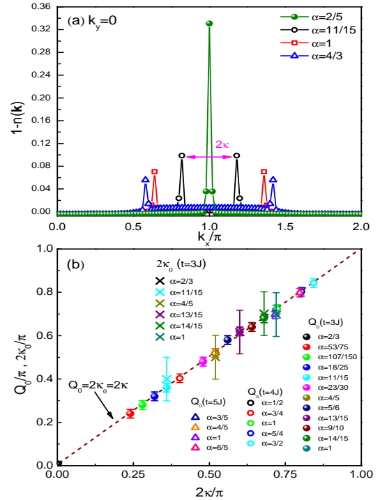
FIG. 4. (Color online) (a) The single-hole momentum distribution ( k_y=0 ) for different values of \alpha in the two-leg t - J ladder, where t/J = 3 and the critical value \alpha_c = 0.7 . For \alpha below \alpha_c the distribution displays a quasiparticle peak at k_x = \pi ; above \alpha_c this quasiparticle peak splits into two symmetric with respect and of a distance \kappa to k_x = \pi . (b) The wave number of the charge modulation Q_0 and the peak distance of the single-hole momentum distribution 2\kappa are found to be identical to twice the wave number of the oscillation of \Delta E_G^{1-\text{hole}}(N_x) , i.e., Q_0 = 2\kappa = 2\kappa_0 (dashed line). Note that Q_0 = 2\kappa = 2\kappa_0 \equiv 0 at \alpha < \alpha_c .
