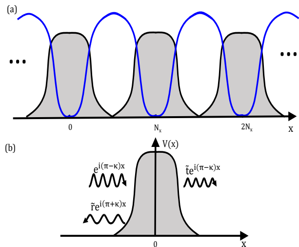
FIG. A1. (a) By enforcing the periodic boundary condition on a ladder we obtain an infinite periodic system. The period of this 1D “crystal” is N_x . The self-localized profile of the hole density (blue solid curve) within a single unit cell implies that the unit cells are weakly coupled to each other via a symmetric tunneling barrier (grey area). (b) A plane wave of momentum (\pi - \kappa) incident on a single tunneling barrier is partially transmitted and reflected. The reflected wave has a momentum of (\pi + \kappa) .
