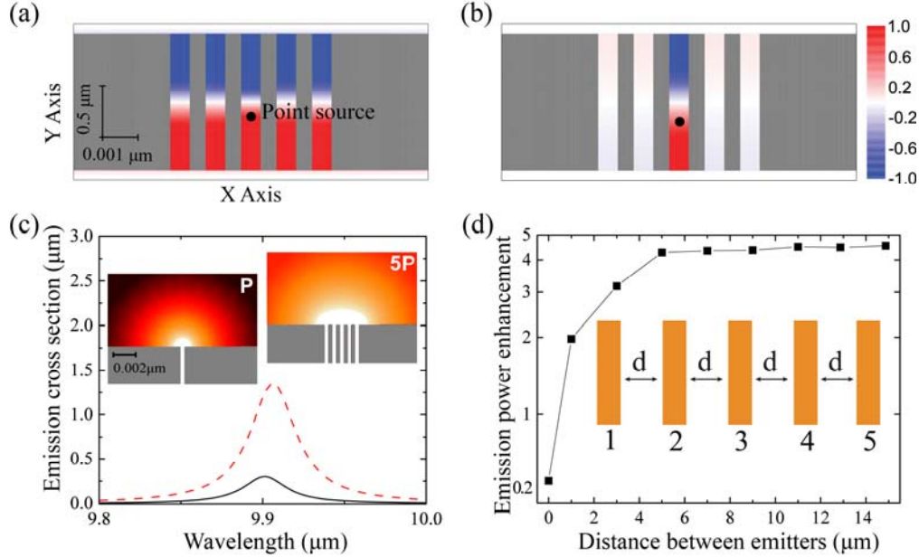
Figure 4. (a) When the absorption rate is low, a point source excites photons with equal amplitudes and phases in all emitters. Color shows the snapshot of the amplitude of the electric field. (b) When the absorption is high, excited amplitude is localized in the slit with the source. (c) Quench of the superradiance effect in the high-loss regime. Spectra of the emission cross section of a single (black solid line) and 5 (red dashed line) resonant emitters. Insets are the intensity distribution of the emission. (d) The emission power as a function of distance between emitters in the low-loss regime. It is normalized by the power generated a single emitter alone. The superradiance effect is weakened as the inter-emitter distance increases.
