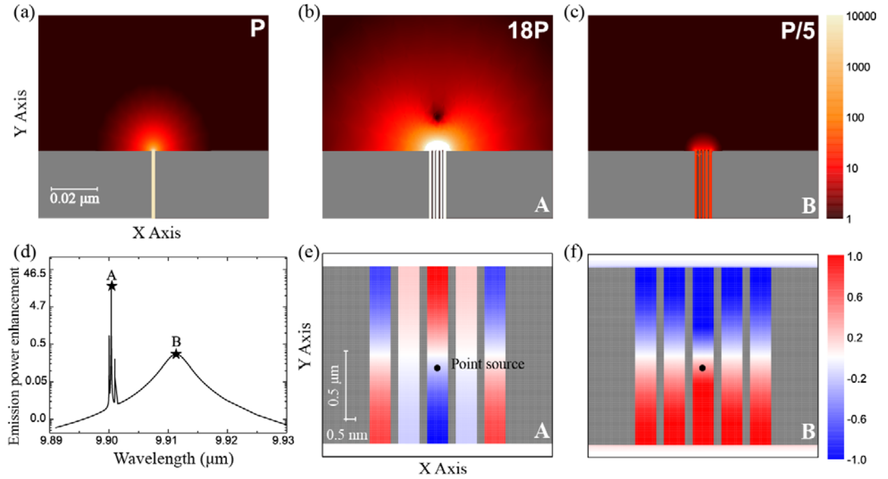
Figure 6. (a) Intensity distribution of the emission from a single emitter. (b) and (c) Intensity distribution of the emission from 5 emitters at the subradiant mode (b) and the superradiant mode (c), respectively. (d) The spectrum of the emission power for 5 emitters, normalized by the peak power of a single emitter. (e) and (f) The amplitude of the electric field excited by a point source in one of the slit for the subradiant mode (e) and the superradiant mode (f), respectively.
