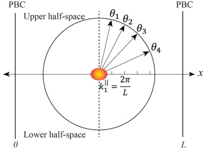
Figure 3. Schematic of the orthogonal radiation channels. An emitter is located within two boundaries where periodic boundary condition (PBC) is applied. The infinite non-periodic case will be obtained by taking the period L \rightarrow \infty .
