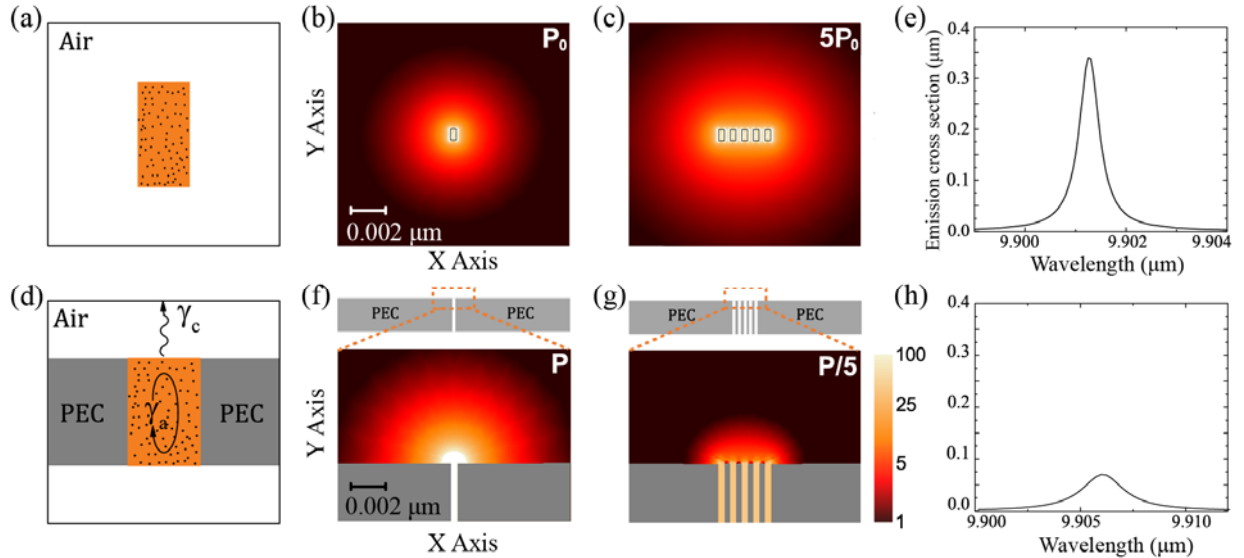
Figure 2. (a) The structure of a non-resonant emitter: a block of emissive materials. Random positioned current sources (black dots) with random phases are used to simulate the thermal emission. (b) and (c) Intensity distribution of the emission at wavelength of 9.9 \mu\text{m} for 1 and 5 non-resonant emitters, respectively. (d) The structure of resonant emitters consisting of a slit in a PEC slab. The length and width of the slit are 1.4 \mu\text{m} and 0.5 \text{ nm} , respectively. It is filled with an emissive material with a dielectric constant of \epsilon = 12.5 + 0.00001i . The resonator is in the over-coupling region. (e) Spectra of emission cross section for 1 resonant emitter. The emission cross section is calculated by integrating the absorption cross section over all angles and also by considering the reciprocal relation between the absorption and the emission. (f) and (g) Distribution for 1 and 5 emitters, respectively.
