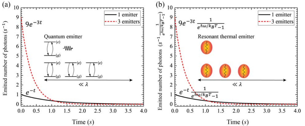
Figure 5. (a) The emitted number of photons flux from quantum emitters as a function of time in the transient decay process. The lifetime of photons is assumed to be 1 s. A single quantum emitter is shown as black solid line. When 3 such quantum emitters are placed together (dashed red), the total number of photons is tripled, and the lifetime of photons is reduced to 1/3 s. As a result of more photons and faster decay, the initial intensity from the emitters is enhanced at t = 0 and drops faster below the black line at a later time. (b) Emitted thermal photons as a function of time for single (black line) and three (red dashed line) resonant thermal emitters. For 3 resonant thermal emitters in a superradiant configuration, the decay rate increases 3 times. The thermal emission increases 9 times at t = 0 , which is the same as the case of quantum emitters.
