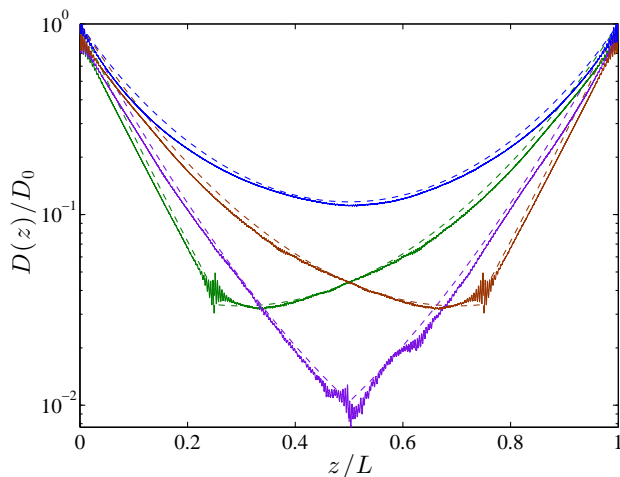
FIG. 2: (Color online) The position-dependent diffusion coefficient inside 1D passive random media with L = 7.6\xi , computed for four source positions: z' = 0 (upper curves), L/4 , L/2 and 3L/4 . The latter three curves have cusps at the position of the source. Dashed lines were found by substituting the analytical result Eq. (13) into Eq. (12). The solid lines were obtained numerically.
