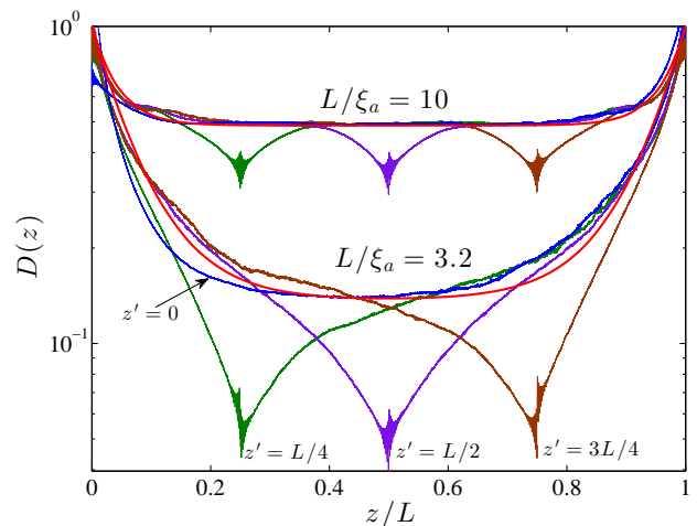
FIG. 3: (Color online) The position-dependent diffusion coefficient in an absorbing random medium with L/\xi = 15.2 . The lower set of curves corresponds to the absorption L/\xi_a = 3.2 and four positions of the source. Thick red line is the prediction of SCT from Eq. (14,15). For a stronger absorption L/\xi_a = 10 (upper set), SCT provides an adequate prediction for PDDC .
