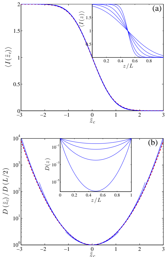
FIG. 1: (a) Spatial distribution of the ensemble-averaged intensity \langle I(z) \rangle from Eq. (7) (blue lines) without scaling (inset) for systems with L/\xi = 5, 10, 20, 50, 100 (left to right). The main panel presents the same data in terms of the scaled coordinate \tilde{z}_c = (z - L/2)/\sqrt{L\xi} ; the approximate expression given by Eq. (8) is shown with thick dashed line. (b) The position-dependent diffusion coefficient found from Eq. (6) for systems with L/\xi = 5, 10, 20, 50 without (inset) and with (main panel) scaling. Thick dashed line is found from the asymptotic L \gg \xi expression in Eq. (9).
