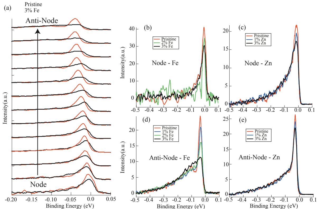
FIG. 3: Effect of the impurity substitution on the coherence peaks. (a) Comparison of the EDCs at k_F of the 3% Fe substituted sample and the pristine sample at 13 different k_F points. (b) Effect of Fe substitution on the coherence peak at the Node. (c) Effect of Zn substitution on the coherence peak at the Node. (d) Effect of Fe substitution on the coherence peak at the Anti-Node. (e) Effect of Zn substitution on the coherence peak at the Anti-Node.
