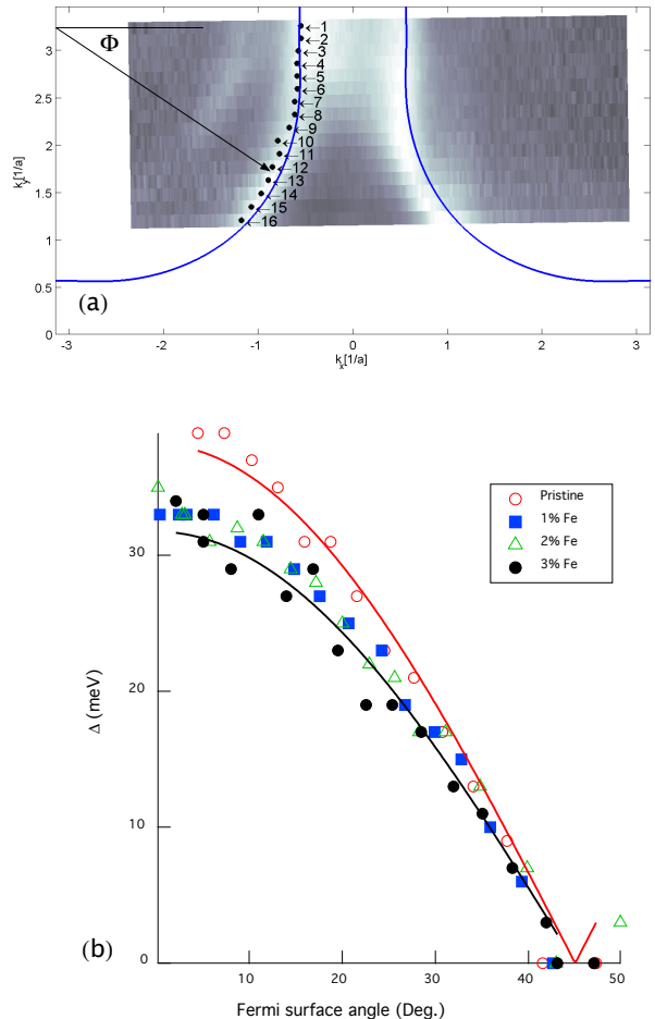
FIG. 2: (a) Intensity map for the 1% Fe substituted sample around the Fermi-level. The intensity was integrated over 40meV around the Fermi-level to show the entire Fermi-surface. The solid-line represents a tight-binding model of the Fermi-surface. (b) The superconducting gap of a pristine samples and the three Fe substituted samples plotted as function of the Fermi-surface angle. The Fermi-surface angle is defined in Fig. 5(a).
