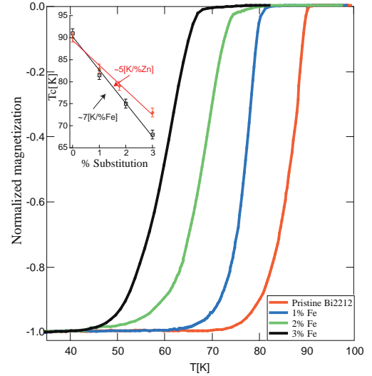
FIG. 1: Normalized magnetization as function of temperature for a pristine samples and the three Fe substituted samples. Inset: T_c as function of the impurity concentration for Fe and Zn substituted Bi2212.
