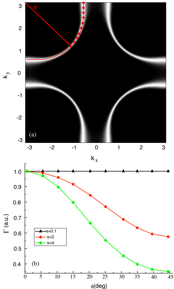
FIG. 5: Effect of the scattering range on the anisotropy of the scattering rate. (a) Shape of the Fermi-surface used in Eq. 4, we used a the tight-binding model of Ref [12] and 10 meV broadening. The red dots represents the points for which we show the scattering rate in panel (b). \phi is the Fermi-surface angle. (b) Scattering rate as a function of the Fermi-surface angle for a Gaussian scattering-potential for various scattering-lengths. S represents the FWHM of the Gaussian in units of lattice constants.
